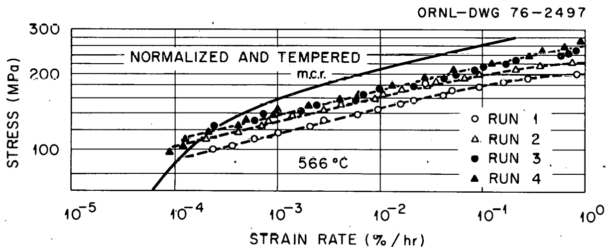
Fig. 11. Creep Rates Determined from Relaxation Data on Normalized-and-Tempered 2 1/4 Cr-1 Mo Steel at 566°C.
