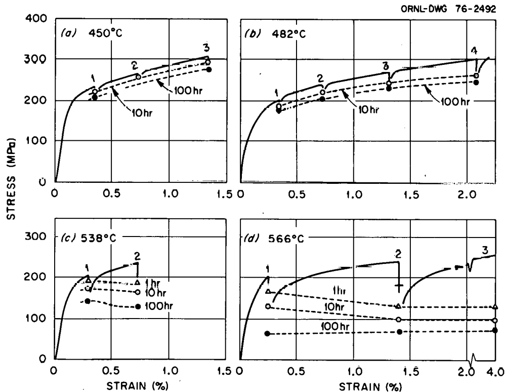
Fig. 3. Isochronous Stress-Strain Curves Obtained from Multiple-Loading Relaxation Tests on Annealed 2 1/4 Cr-1 Mo Steel.
