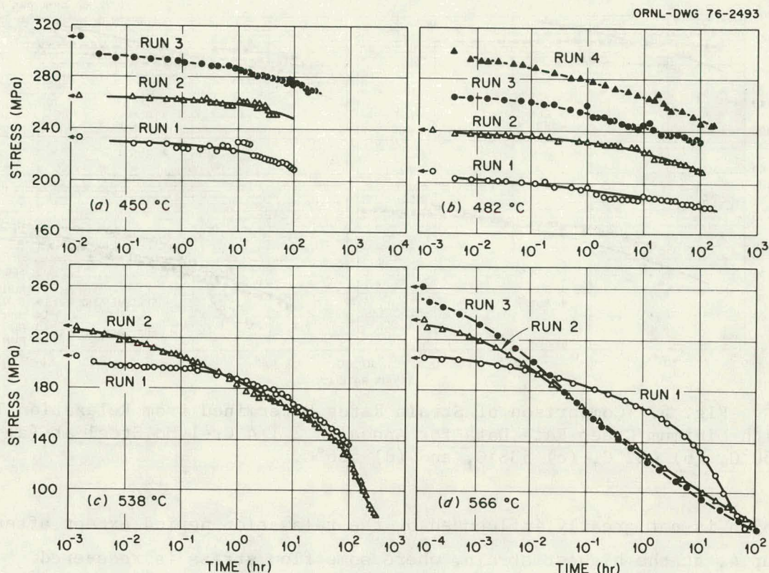
Fig. 4. Relaxation Data Obtained from Multiple-Loading Tests on 2 1/4 Cr-1 Mo Steel at (a) 450°C, (b) 482°C, (c) 538°C, and (d) 566°C.
