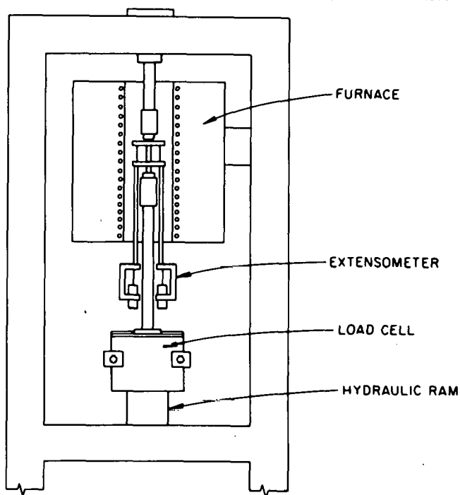
Fig. 2. Schematic of Experimental Setup for Relaxation Testing.
