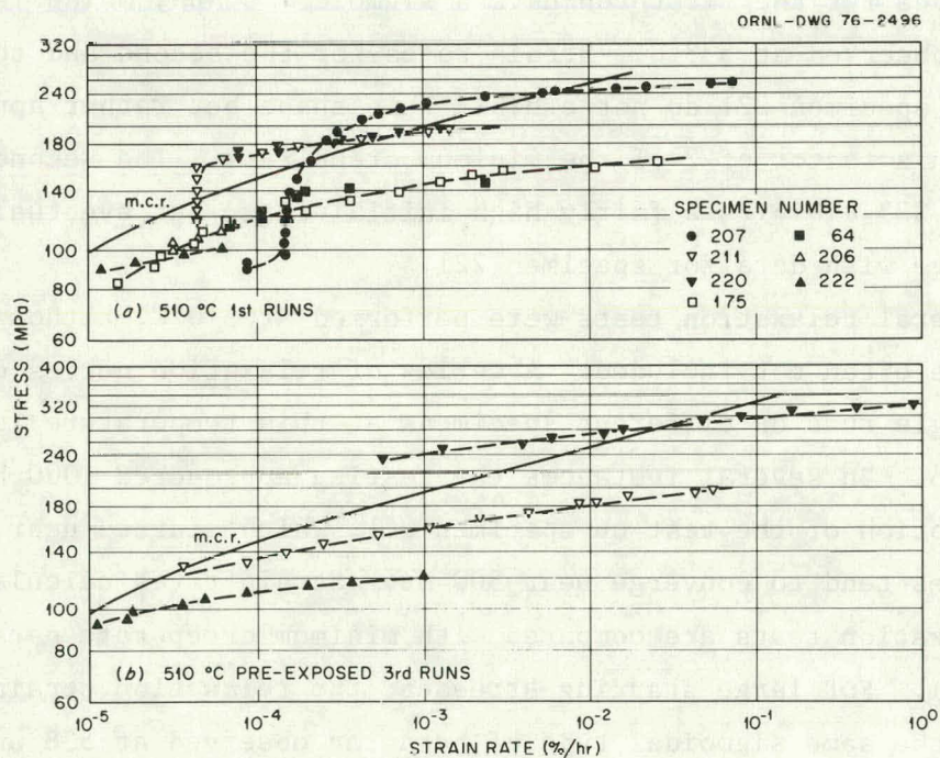
Fig. 7. Strain Rate Data Determined from Relaxation Tests on Annealed 2 1/4 Cr-1 Mo Steel at 510°C.
