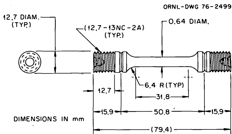
Fig. 1. Relaxation Specimen.
