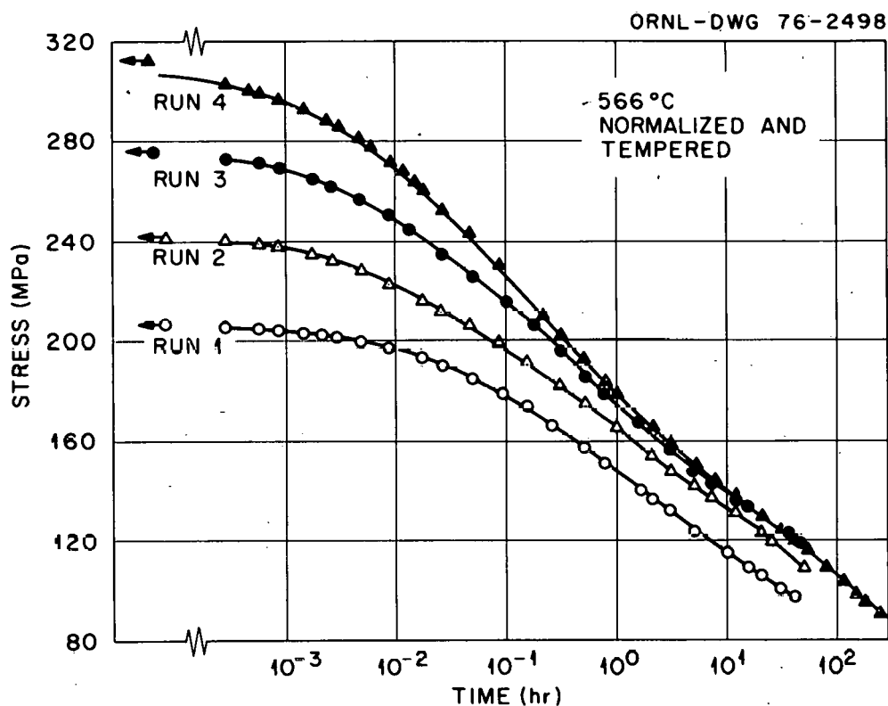
Fig. 10. Relaxation Data Obtained from Multiple-Loading Tests on Normalized-and-Tempered 2 1/4 Cr-1 Mo Steel at 566°C.
