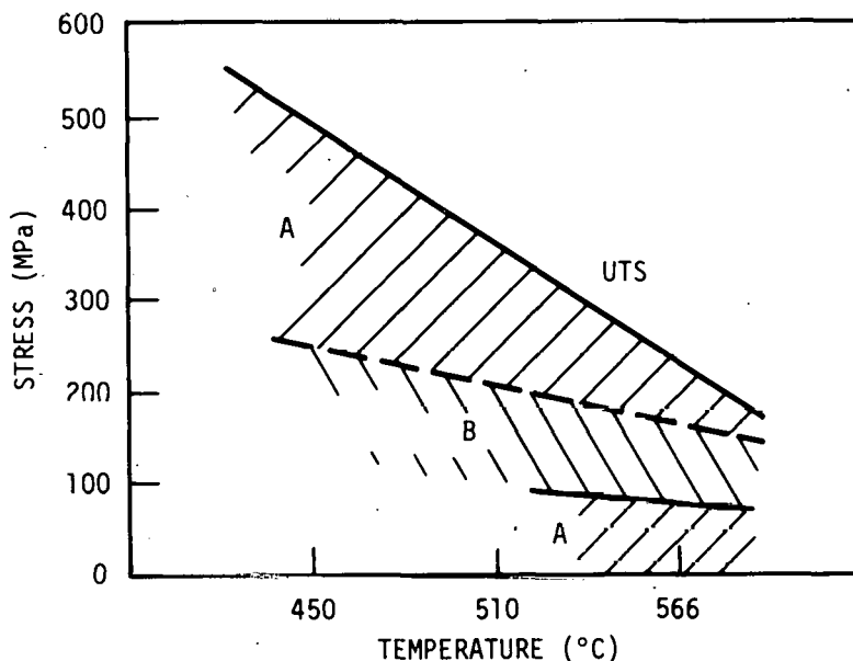
Fig. 9. Region of Stress and Temperature Where Nonclassical Creep is observed in Annealed 2 1/4 Cr-1 Mo Steel.
