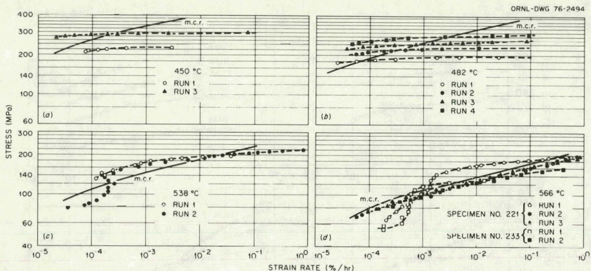
Fig. 5. Comparison of Strain Rates Determined from Relaxation Tests with Minimum Creep Rate Data for Annealed 2 1/4 Cr-1 Mo Steel at (a) 450°C, (b) 482°C, (c) 538°C, and (d) 566°C.
