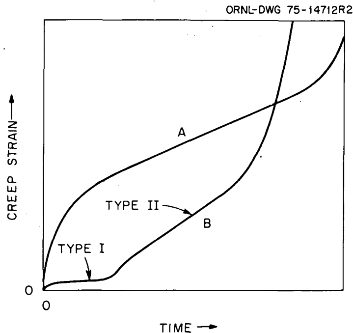
Fig. 8. Schematic Diagrams for Classical (A) and Nonclassical (B) Curves of the Type Observed for 2 1/4 Cr-1 Mo Steel.
