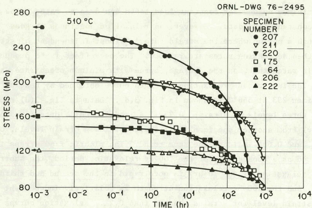
Fig. 6. Relaxation Data Obtained from Single Loadings on 2 1/4 Cr-1 Mo Steel at 510°C.
