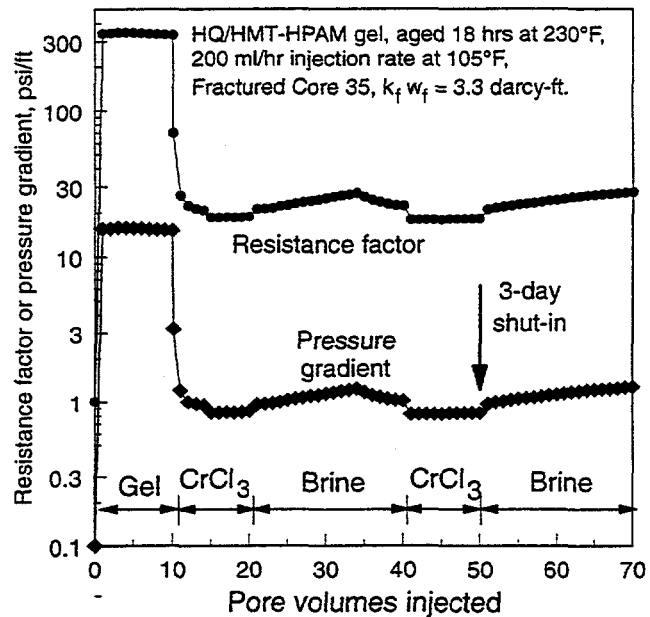
Fig. 56. Effect of CrCl_3 injection after placement of a HQ/HMT-HPAM gel.
