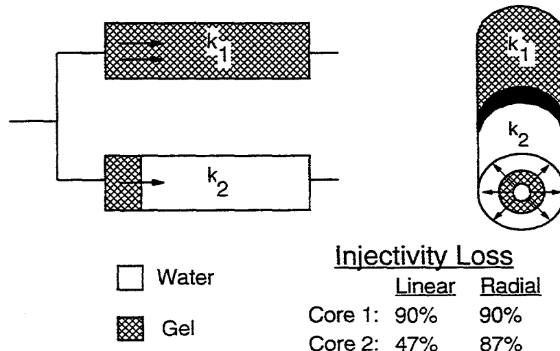
Fig. 1. Linear versus radial parallel coreflows.
