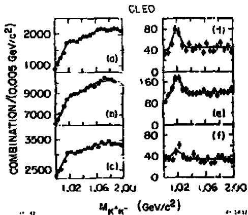
Fig. 24. CLEO K^+K^- invariant mass spectra for T(1S) (a) and (d), T(4S) (b) and (e) and continuum (c) and (f). No particle identification is used in (a)-(c); one identified kaon is required for (d)-(f).
