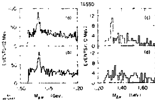
Fig. 10. Invariant mass spectra from TASSO for (a) p\pi^- , (b) p\pi^+ , (c) \Lambda\pi^- + \bar{\Lambda}\pi^+ and (d) \Lambda\pi^+ + \bar{\Lambda}\pi^- .
