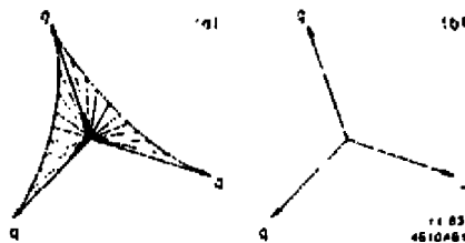
Fig. 37. Artist's perception of the difference between the string picture (a) and the independent fragmentation picture (b). For these pictures \sigma_q = 0 .
