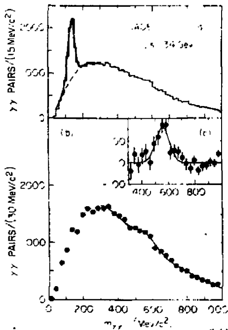
Fig. 11. (a) Photon-photon invariant mass distribution for E_\gamma > 200 \text{ MeV} , E_{\gamma\gamma} > 700 \text{ MeV} from JADE. (b) Same as (a) except photons with E > 300 \text{ MeV} which form a \pi^0 are removed and (c) \eta signal with background subtracted.
