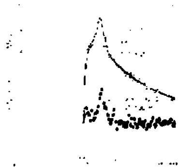
Fig. 16 The K^{\pm} \pi^{\mp} invariant mass spectrum from the TPC.
