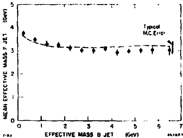
Fig. 40. HRS data for jet mass correlations.
