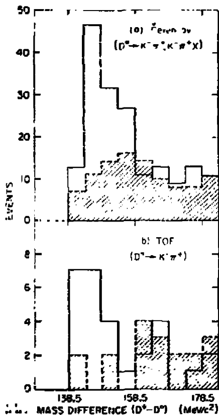
Fig. 26. The mass difference \Delta = M(D^0\pi^+) - M(D^0) is shown for the DELCO experiment. (a) Using the Cherenkov tag and (b) using the time of flight tag. The shaded region is an estimate of the background obtained from wrong sign K 's.
