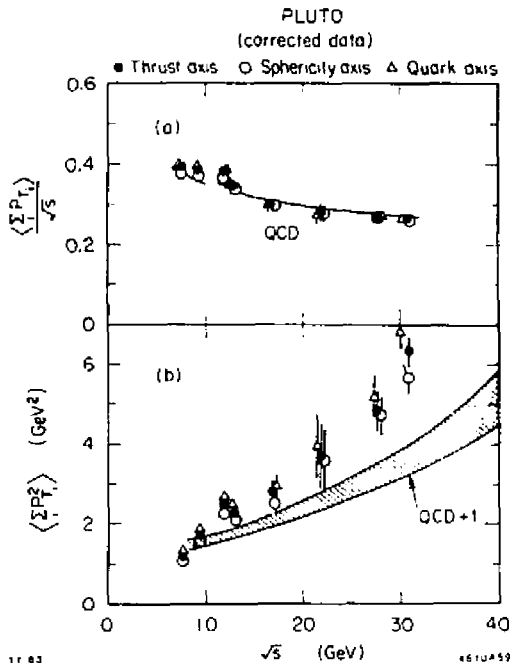
Fig. 43. The PLUTO data for (a) \langle \sum P_{T_i} \rangle / \sqrt{s} as a function of \sqrt{s} . The full (open) circles refer to P_T relative to the thrust (sphericity axis). The triangles refer to values of P_T obtained with respect to the most energetic parton direction. The solid line indicates the LLA QCD prediction of Rakow and Webber for \Lambda = 600 MeV. (b) \langle \sum P_{T_i}^2 \rangle as a function of \sqrt{s} . The prediction of Rakow and Webber is represented by the shaded area.
