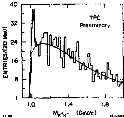
Fig. 18. The TPC K^+K^- invariant mass spectrum.
