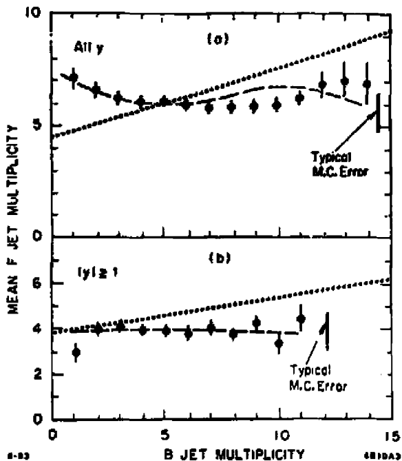
Fig. 48. IRS data for multiplicity correlations for (a) all the data and (b) the central region |y| \leq 1 is removed. The dashed line is the prediction of the Monte Carlo and the trend of the 540 GeV pp data is indicated as a dotted line.
