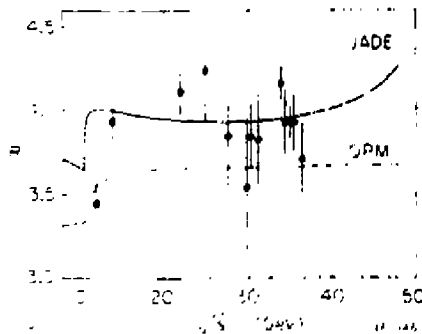
Fig. 38. R as a function of \sqrt{s} from JADE.
