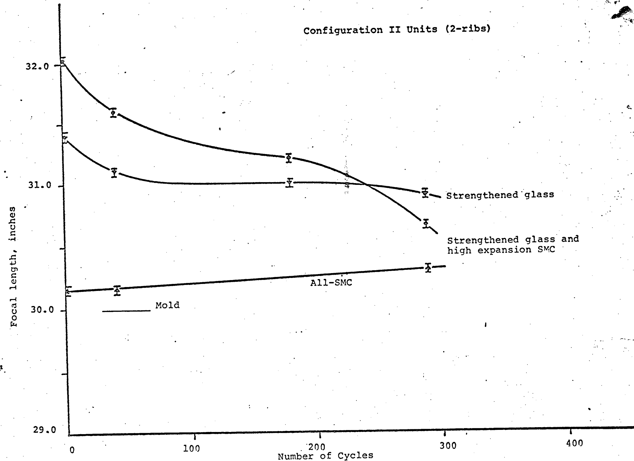
Figure 10 Change in focal length with thermal cycling
