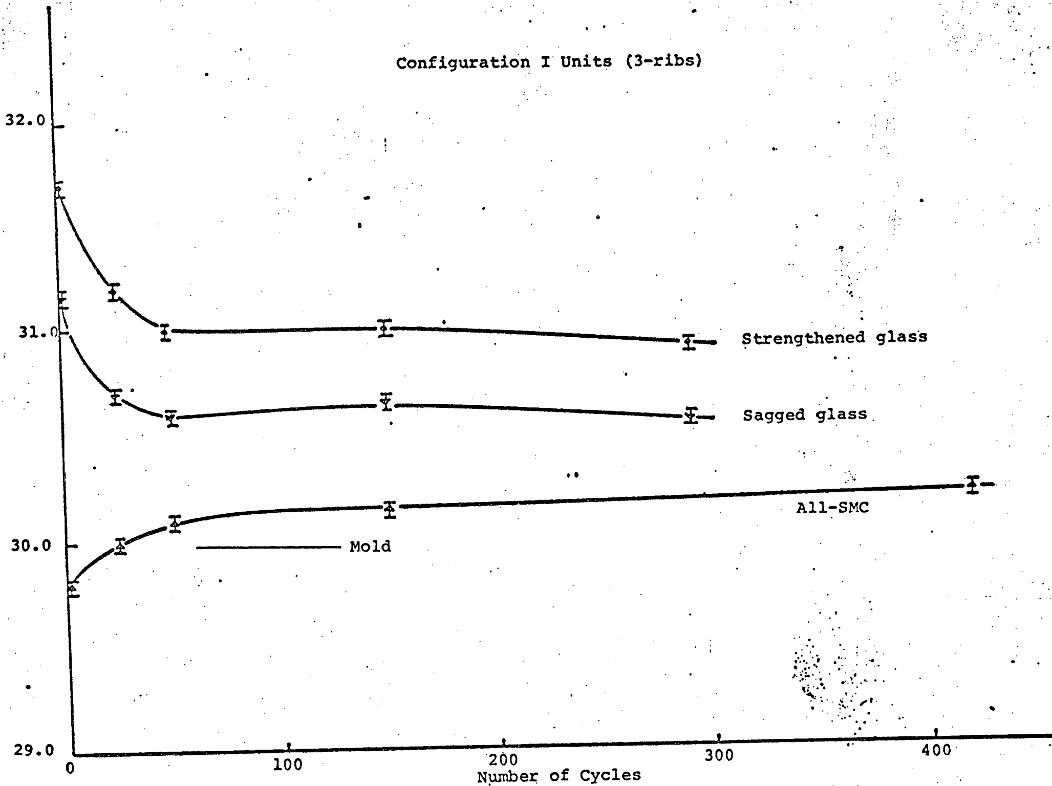
Figure 9 Change in focal length with thermal cycling
