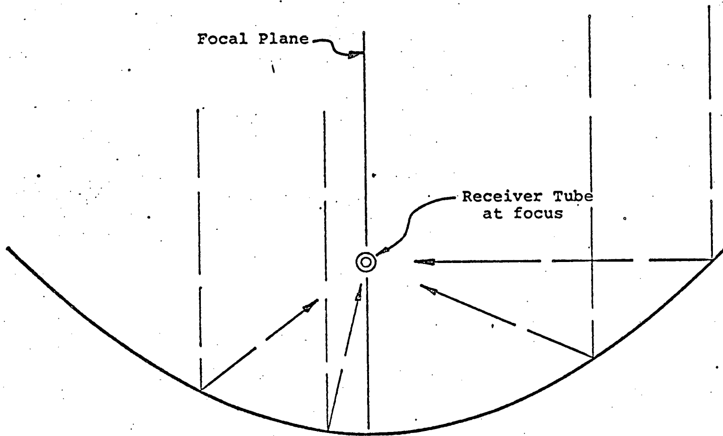
Figure 2. Parabolic Reflector
