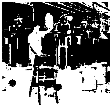
Fig. 5. SLC 50-MW Flytrons mounted in their oil-filled pulse-transformer tanks and surrounded by their focusing electromagnets. The collector is upright and shielded in lead and the double-window output circuit is next to it.
