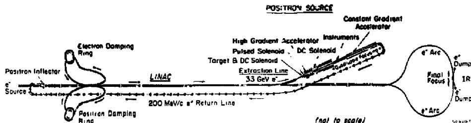
Fig. 7. Schematic diagram of the positron source system.
