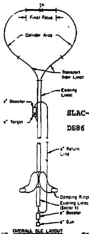
Fig. 1. Schematic layout of the SLC.
