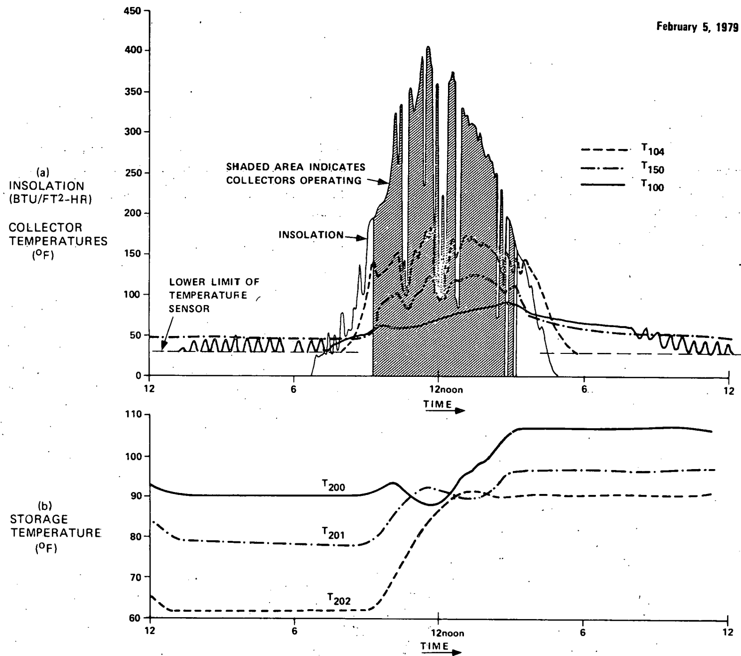
Figure 2.1-1 Typical System Operating Parameters
