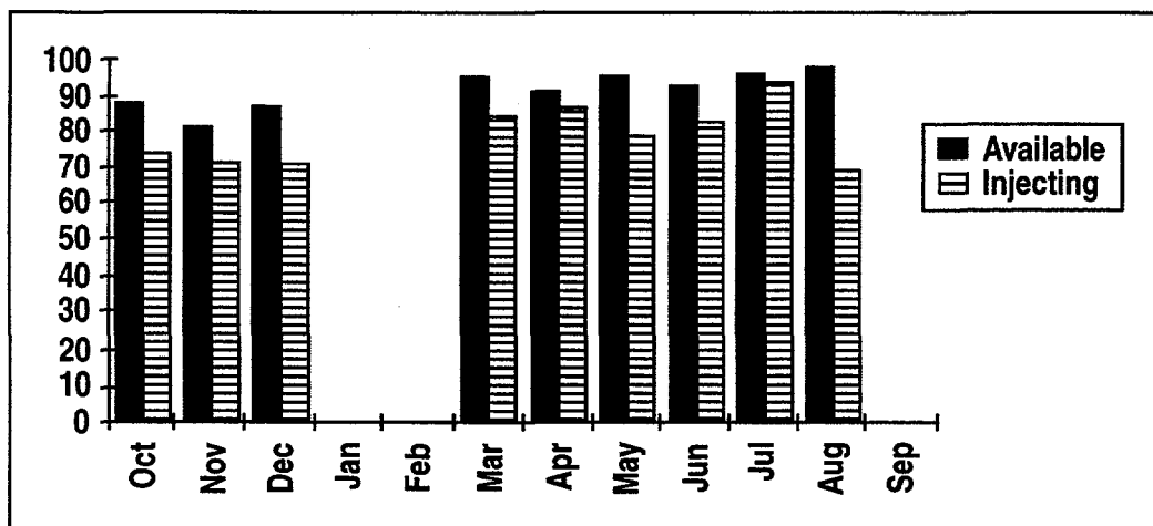
Fig. 5.3-1. NB availability by month.
