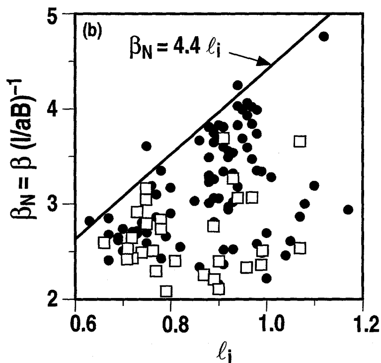
Fig. 3.1-2. Dependence of the beta limit on the current density profile as parameterized by the internal inductance \ell_i , for double-null NCS discharges with H-mode edge and weak or positive shear (circles) or strong negative shear (squares).
