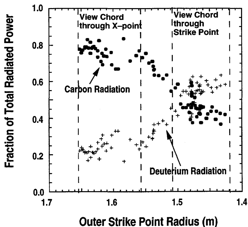
Fig. 2.1-2. Spectroscopically determined radiation fractions due to carbon and deuterium along the viewchord of the Divertor SPRED spectrometer. The radiation from each species is plotted as a fraction of the total chord integrated radiation along a bolometer chord with a similar view.
