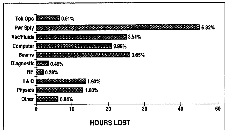
Fig.5.2-2. Downtime for FY96.
