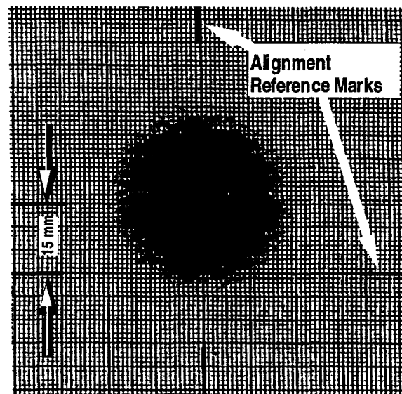
Fig. 6.1-2. RF burn pattern 1724 mm from gyrotron window.
