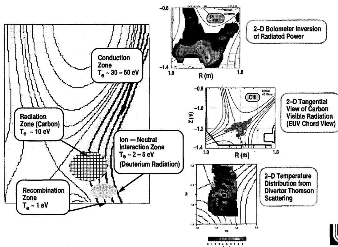
Fig. 8.2-1. We are developing a physics model of the detached divertor plasma with new 2-D diagnostic data.
