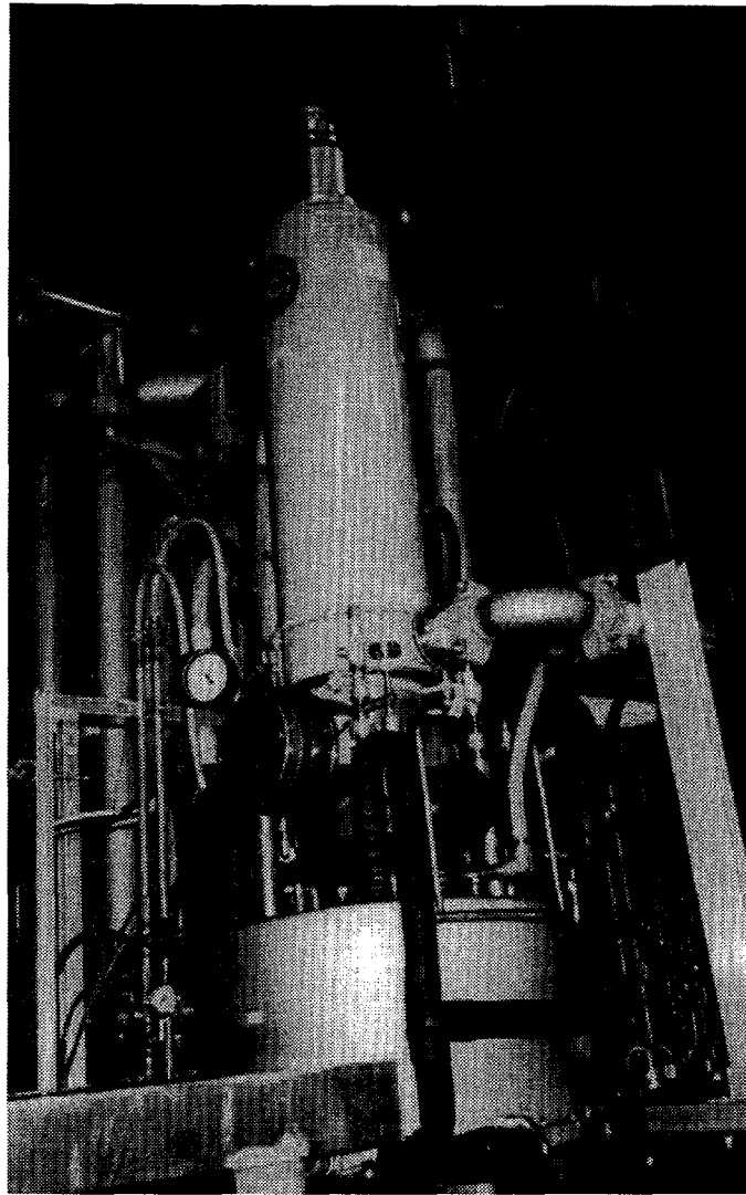
Fig. 6.1-1. 110 GHz GYCOM gyrotron installed in DIII-D ECH vault.
