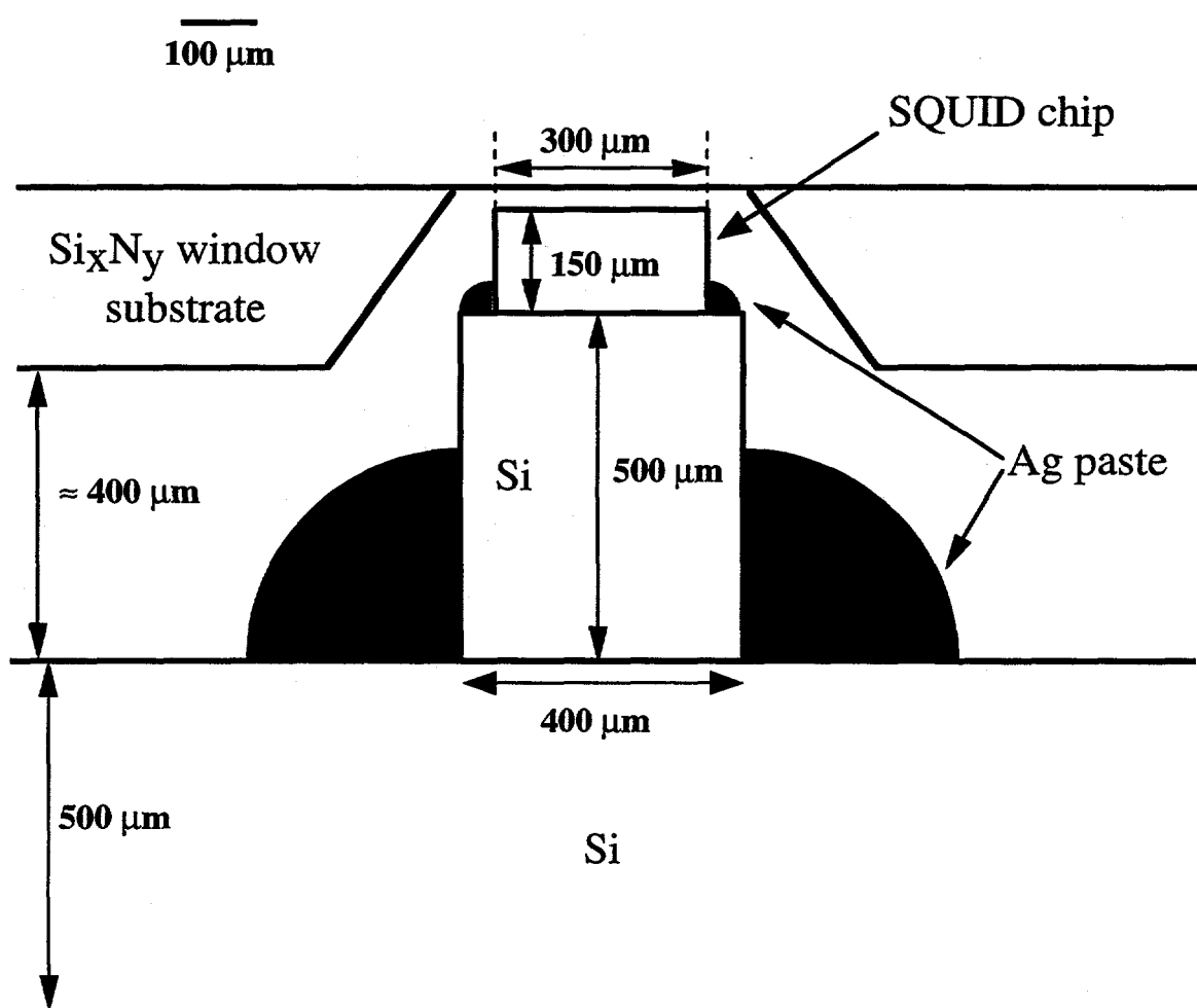
Figure 7.7: Silicon basepiece with a SQUID chip mounted.
