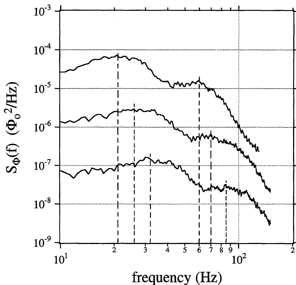
Figure 9.7: Expanded-view of the motile-bacteria spectra of Figure 9.6 with the 1/f^{\alpha} -backgrounds (dotted lines in Figure 9.6) subtracted away. The lower, middle, and upper curves correspond to t = 0, 15 and 75 min, respectively. The vertical dotted lines represent the estimated peak positions. The middle and upper curves are multiplied by factors of 10 and 100, respectively, to shift them upwards for the sake of clarity.
