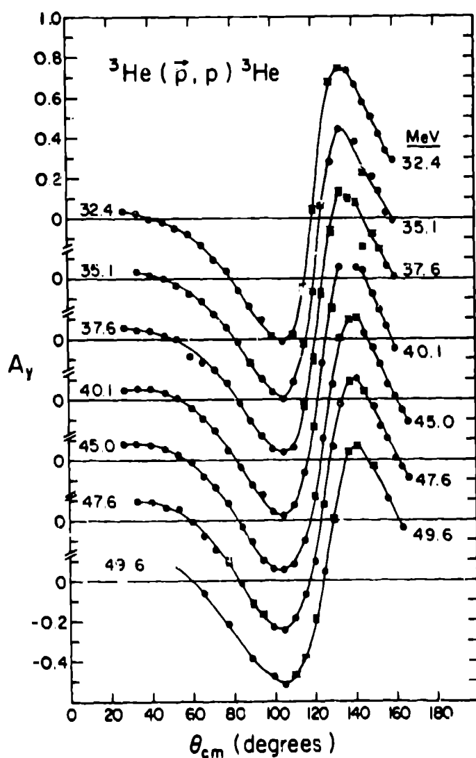
Fig. 1 Analyzing powers A_y for {}^3\text{He}(\vec{p}, p){}^3\text{He} between 30 and 50 MeV. The curves are to guide the eye.
