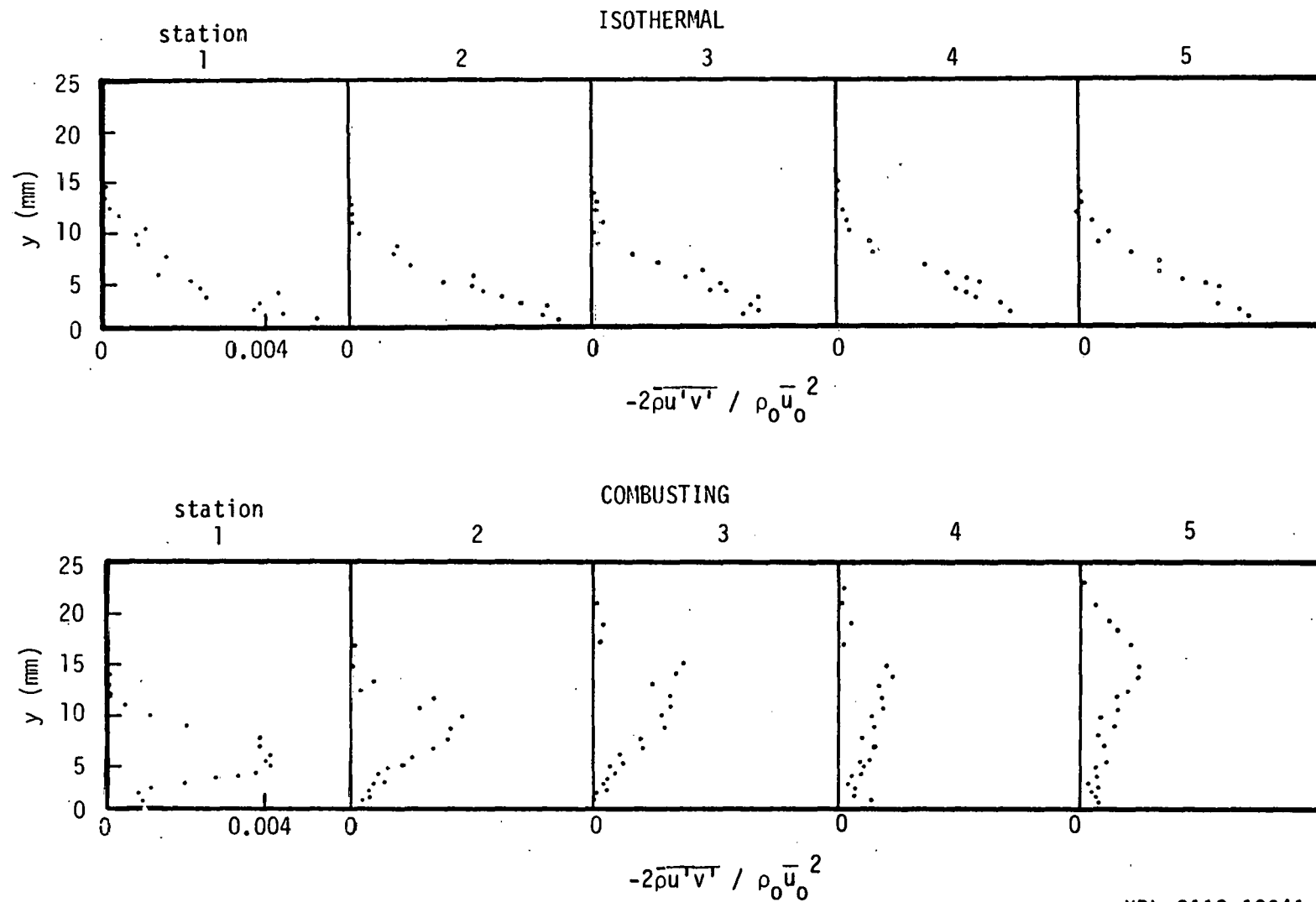
Fig. 9 Reynolds stress profiles of the isothermal and the reacting boundary layer at several axial stations.
