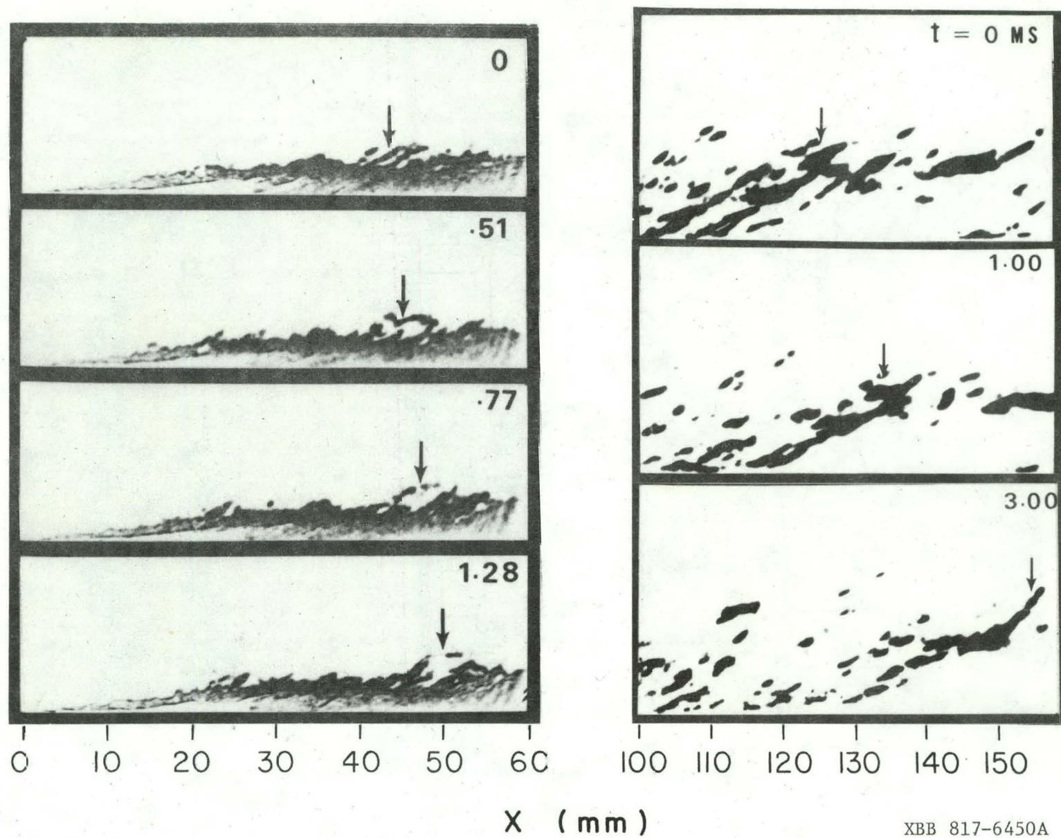
Fig. 2 Schlieren records of the reacting boundary layer.
