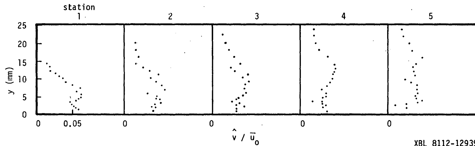
Fig. 7 Rms velocity fluctuation profiles of the reacting boundary layer at several axial stations.
