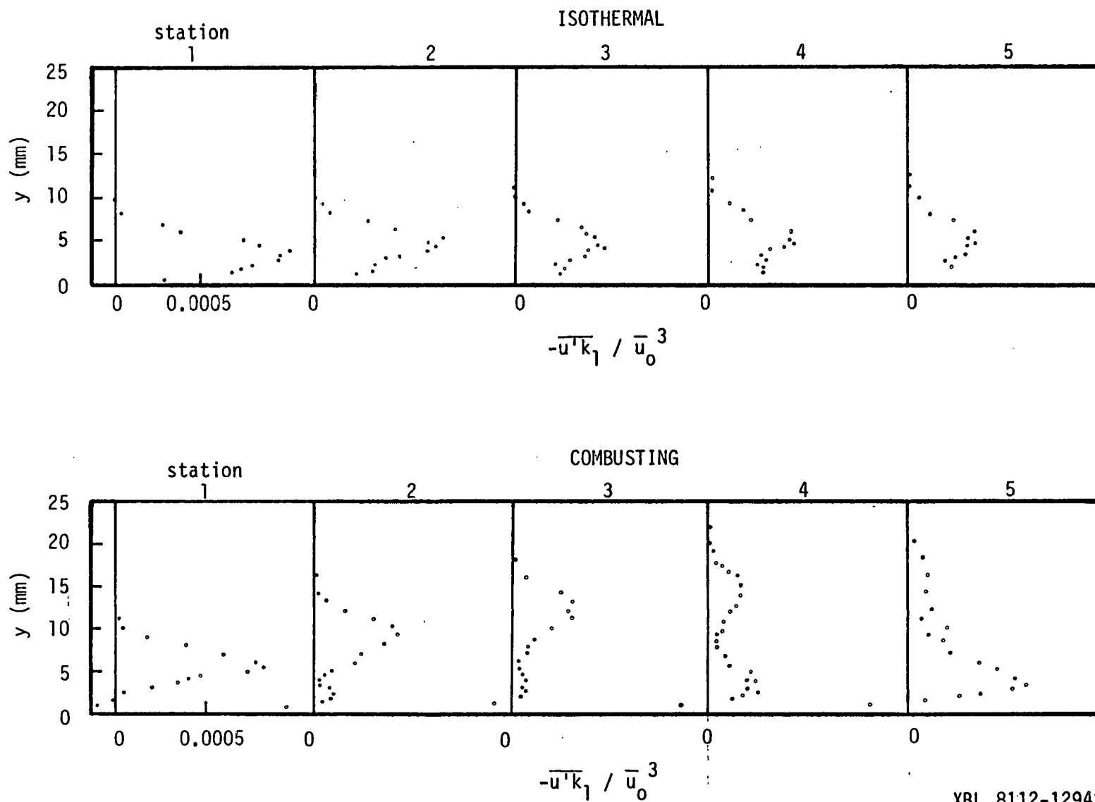
Fig. 10 Streamwise turbulent kinetic energy diffusion of the isothermal and the reacting boundary layer at several axial stations.
