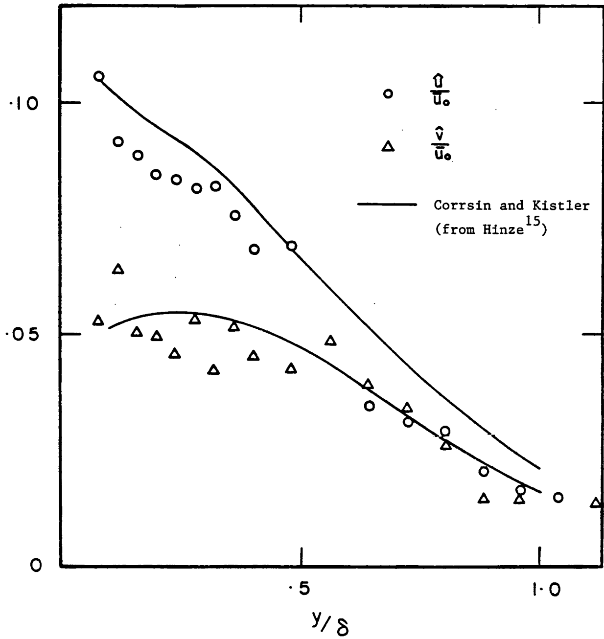
Fig. 6 Rms velocity fluctuation profiles of the isothermal boundary layer at station 5.
