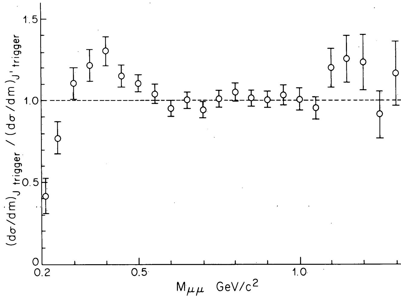
FIGURE 4-16. THE RATIO OF \frac{d\sigma}{dm} AS CALCULATED FROM DATA TAKEN WITH THE J TRIGGER TO THAT TAKEN WITH THE J' TRIGGER IS SHOWN AS A FUNCTION OF MASS. THIS TESTS OUR UNDERSTANDING OF THE ACCEPTANCE WITH THE J TRIGGER REQUIREMENT AS WELL AS THE EFFICIENCY OF THE J TRIGGER.
