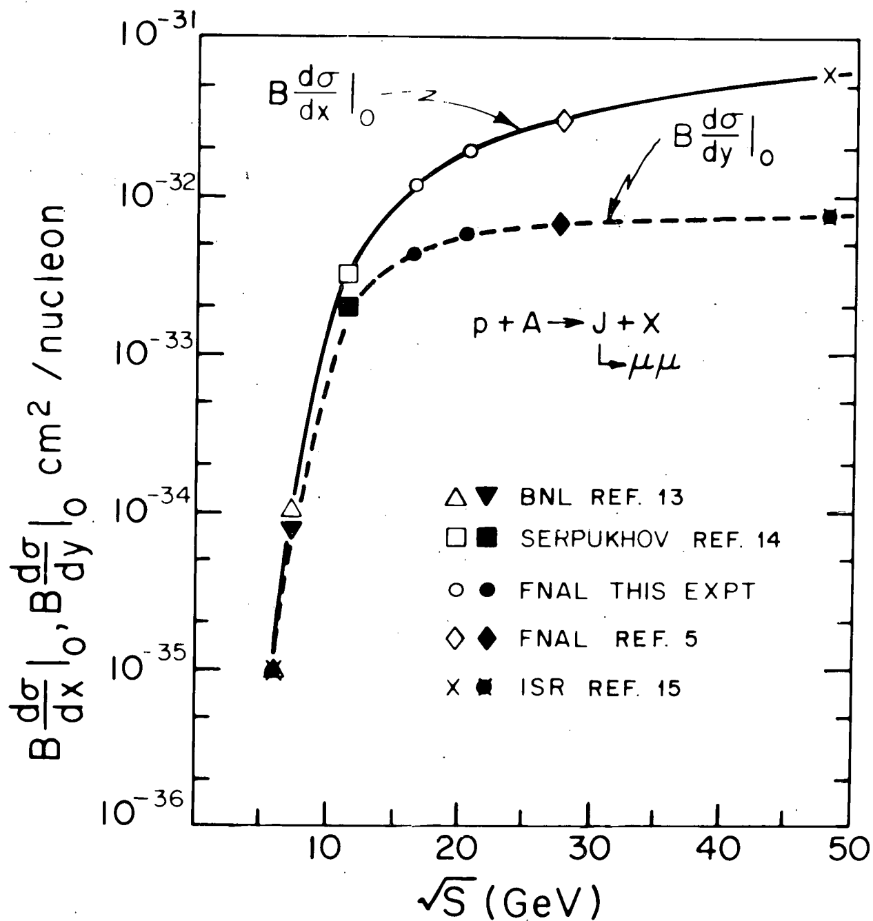
FIGURE 5-35. DEPENDENCE OF J PRODUCTION ON \sqrt{S} .
