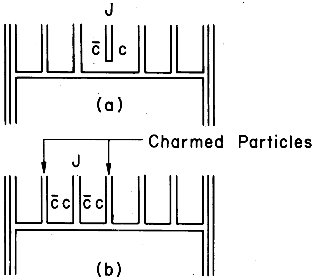
FIGURE 1-1. TWO QUARK-LINE DIAGRAMS FOR J PRODUCTION. (A) THIS DIAGRAM IS NOT ALLOWED BY THE OZI RULE BECAUSE THERE IS A DISCONNECTED QUARK-LINE. (B) THIS IS AN OZI ALLOWED DIAGRAM. A PAIR OF CHARMED PARTICLES IS PRODUCED IN ASSOCIATION WITH THE J ALLOWING ALL QUARK-LINES TO BE CONNECTED.
