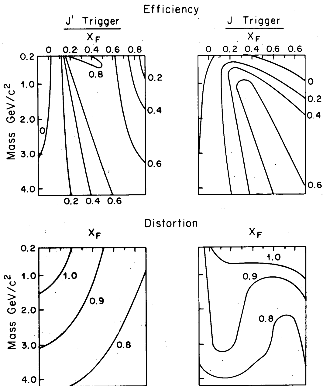
FIGURE 4-9. CONTOUR PLOTS OF EFFICIENCY AND DISTORTION USED TO CALCULATE \frac{d^2\sigma}{dm dx_F} VERSUS X_F AND MASS.
