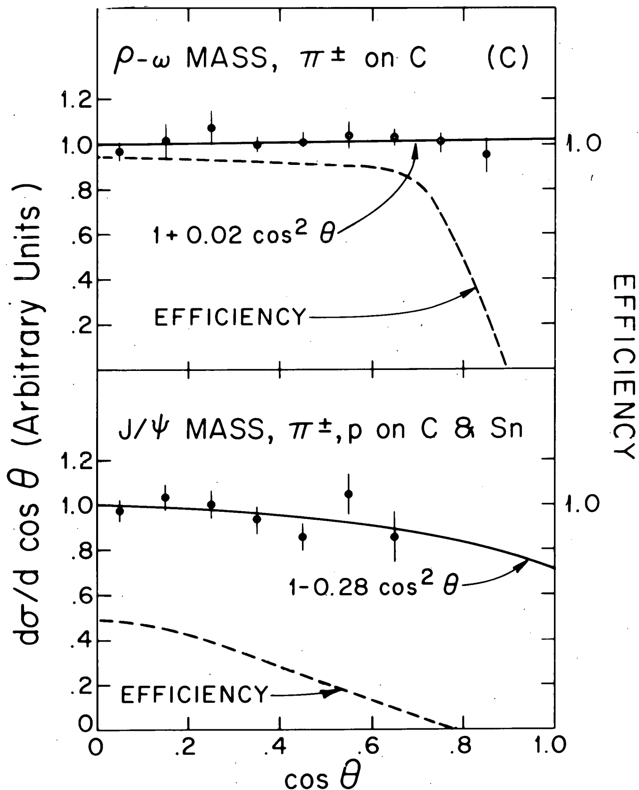
FIGURE 5-34. ANGULAR DISTRIBUTION OF J DECAY TO \mu^+ \mu^- IN THE HELICITY FRAME.
