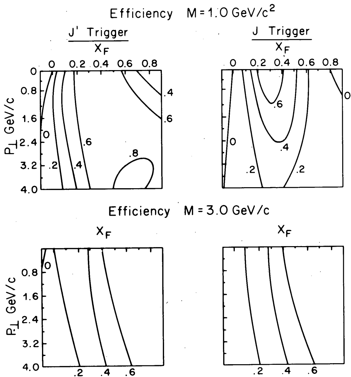
FIGURE 4-11. CONTOUR PLOTS OF EFFICIENCY AND DISTORTION VERSUS X_F AND P_{\perp} , USED TO CALCULATE E \frac{d^3\sigma}{dx_F dP_{\perp}^2}
