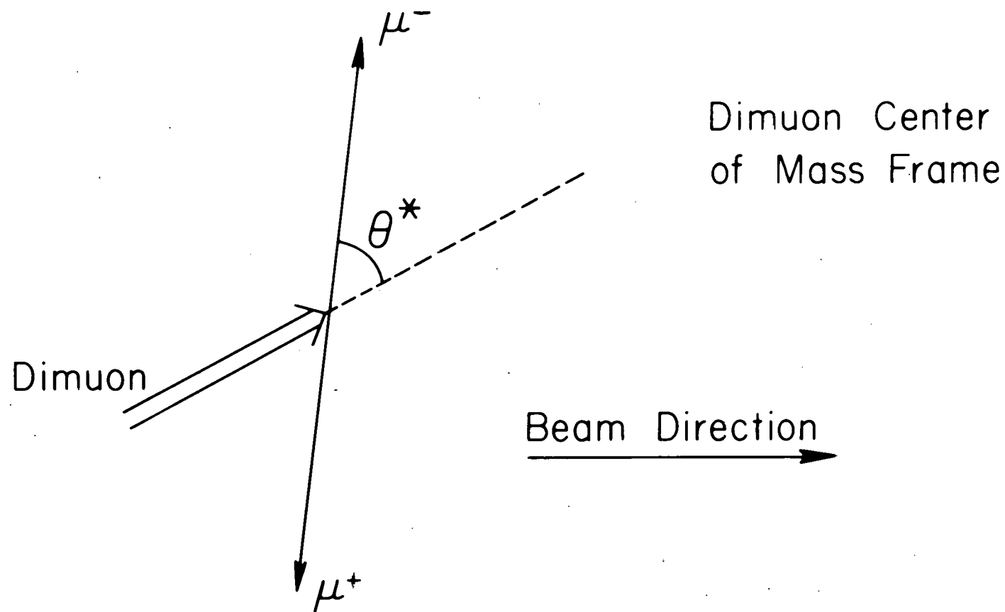
FIGURE 1-3. \theta^* IS DEFINED AS THE ANGLE BETWEEN THE \mu^- AND THE DIMUON DIRECTION IN THE FRAME IN WHICH THE DIMUON IS AT REST.
