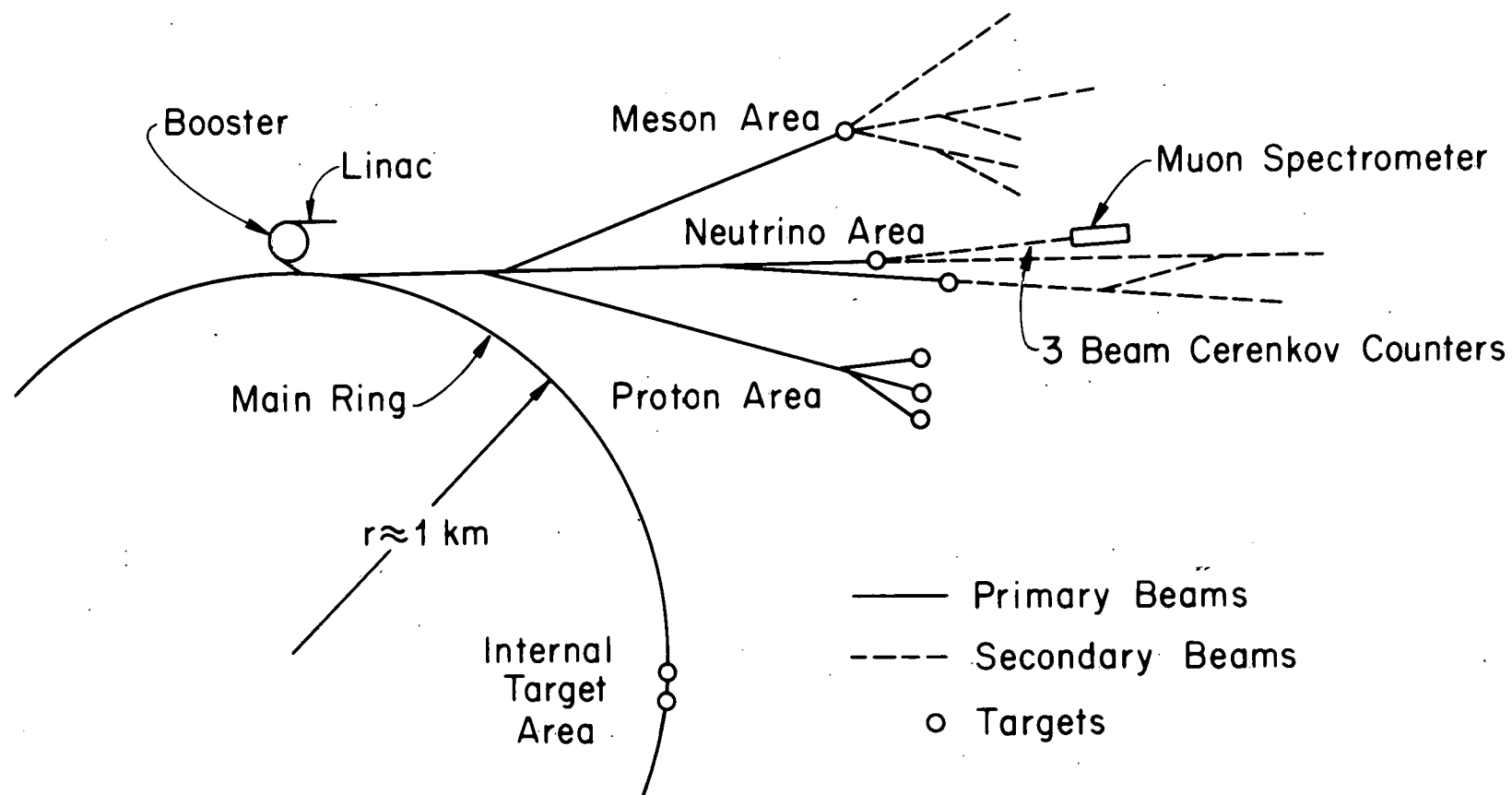
FIGURE 2-1. THE ACCELERATOR AND BEAM LINE LAYOUT AT THE FERMI NATIONAL ACCELERATOR LABORATORY. OUR EXPERIMENT WAS PERFORMED IN THE BUILDING LABELED MUON SPECTROMETER.
