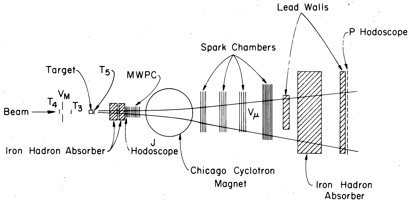
FIGURE 2-2. DIAGRAM OF APPARATUS IN THE MUON LABORATORY.
