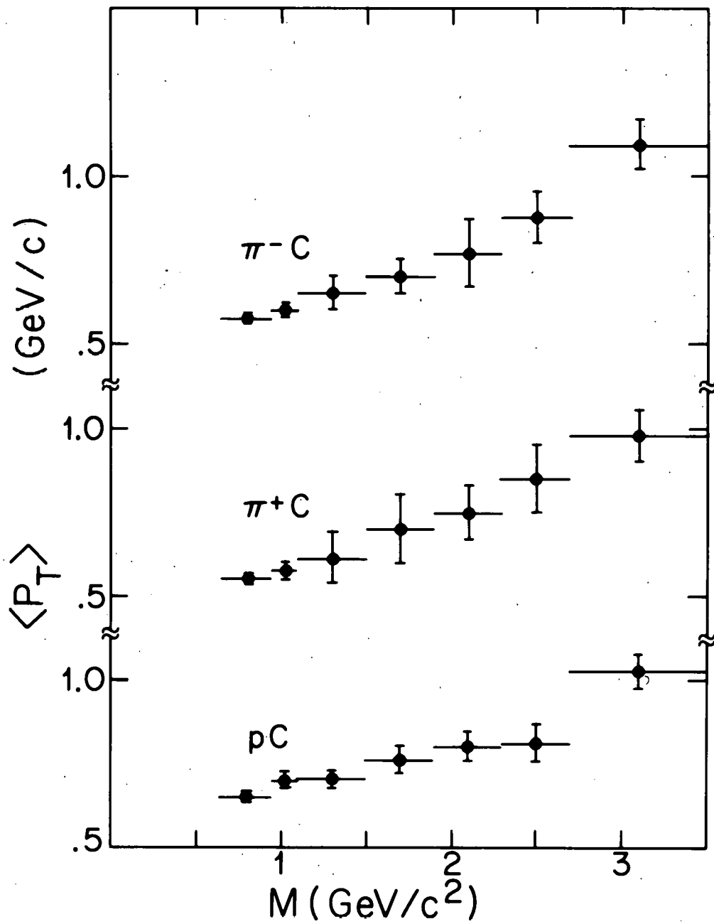
FIGURE 5-32. PLOTS OF \langle P_T \rangle VERSUS MASS FOR \pi^+ , \pi^- AND PROTONS INCIDENT ON CARBON.
