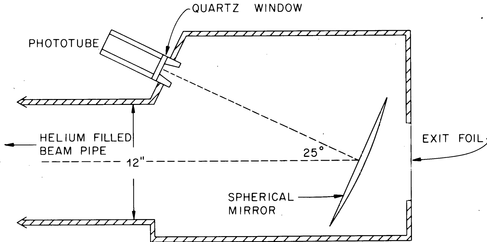
FIGURE 2-4. SIMPLIFIED DRAWING OF A BEAM CERENKOV COUNTER. LIGHT EMITTED BY THE GASEOUS HELIUM RADIATOR IS FOCUSED ON THE PHOTOCATHODE OF AN RCA 31000M PHOTOMULTIPLIER TUBE BY THE ALUMINIZED SURFACE OF A SPHERICAL LUCITE MIRROR. BEAM PARTICLES PASS THROUGH THE 1/8 INCH THICK MIRROR AND A TUNGSTEN EXIT FOIL.
