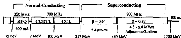
Figure 1. APT Accelerator Schematic.
