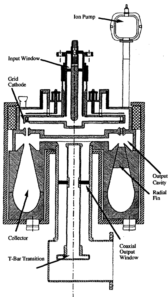
Figure 3. Cross-sectional view of HOM-IOT.
