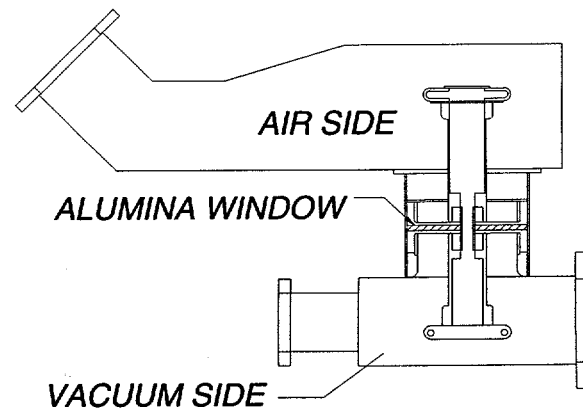
Figure 5. 350 MHz RF coaxial window .
