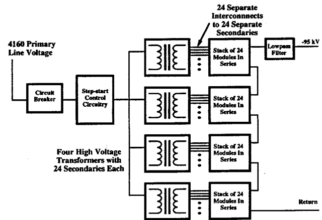
Figure 4. Solid state power supply topology.
