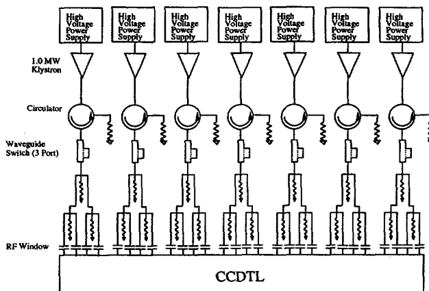
Figure 2. RF Supermodule
