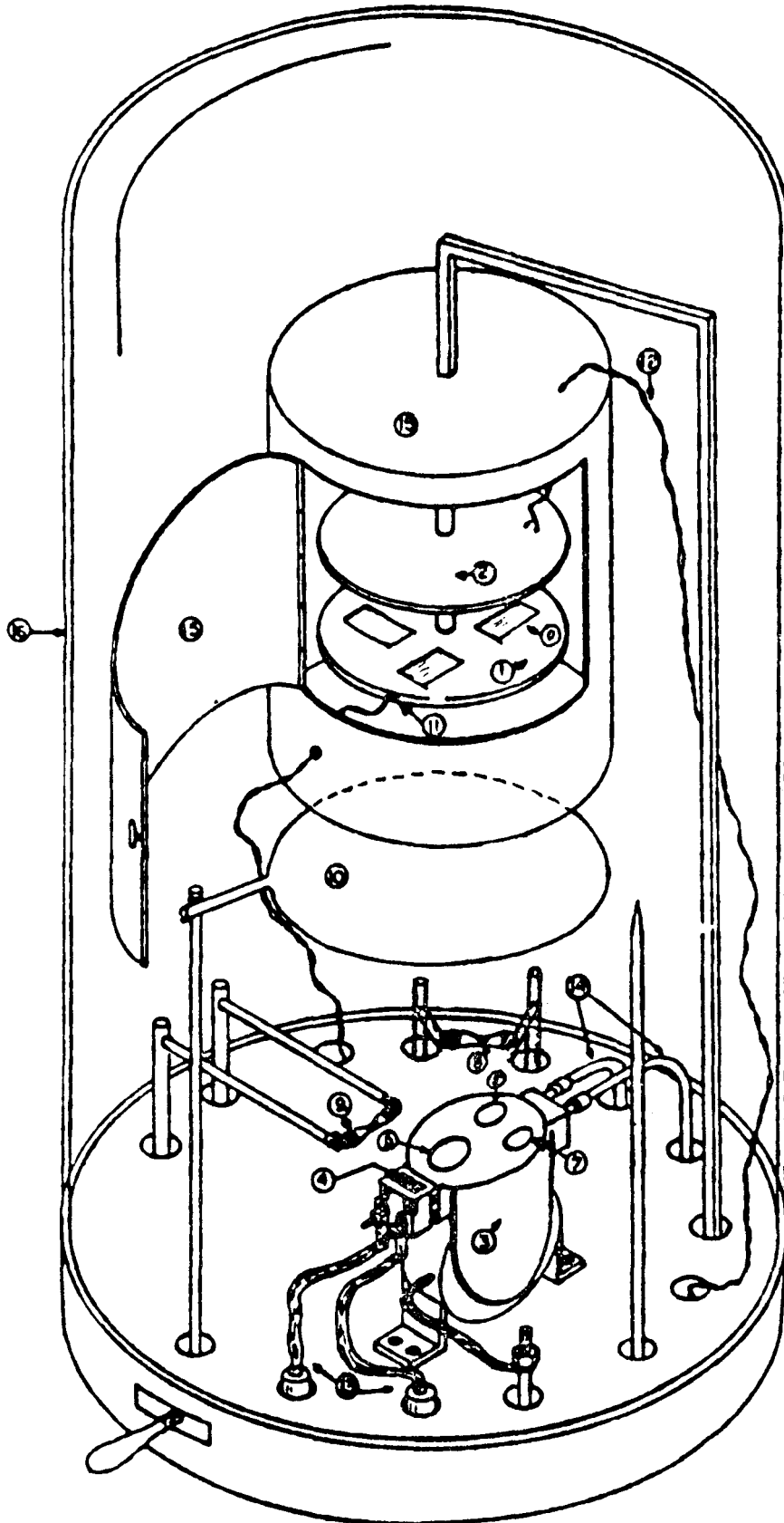
FIGURE 3 EVAPORATION ASSEMBLY
