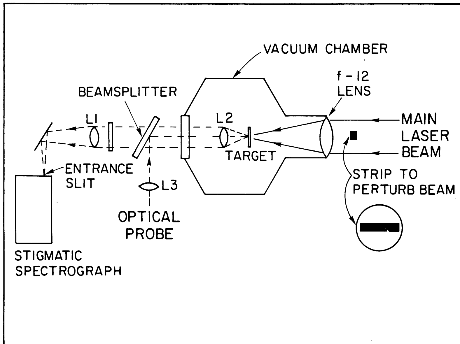
Fig. 1 — Experimental arrangement for determining the velocity profiles of ablatively accelerated targets from doppler shifts of reflected optical probe light. These measurements have a velocity resolution of 10^5 cm/sec and a spatial resolution of 20\text{ }\mu\text{m} . For some experiments, the main laser uniformity is perturbed by placing strips of opaque material in front of the focusing lens.
