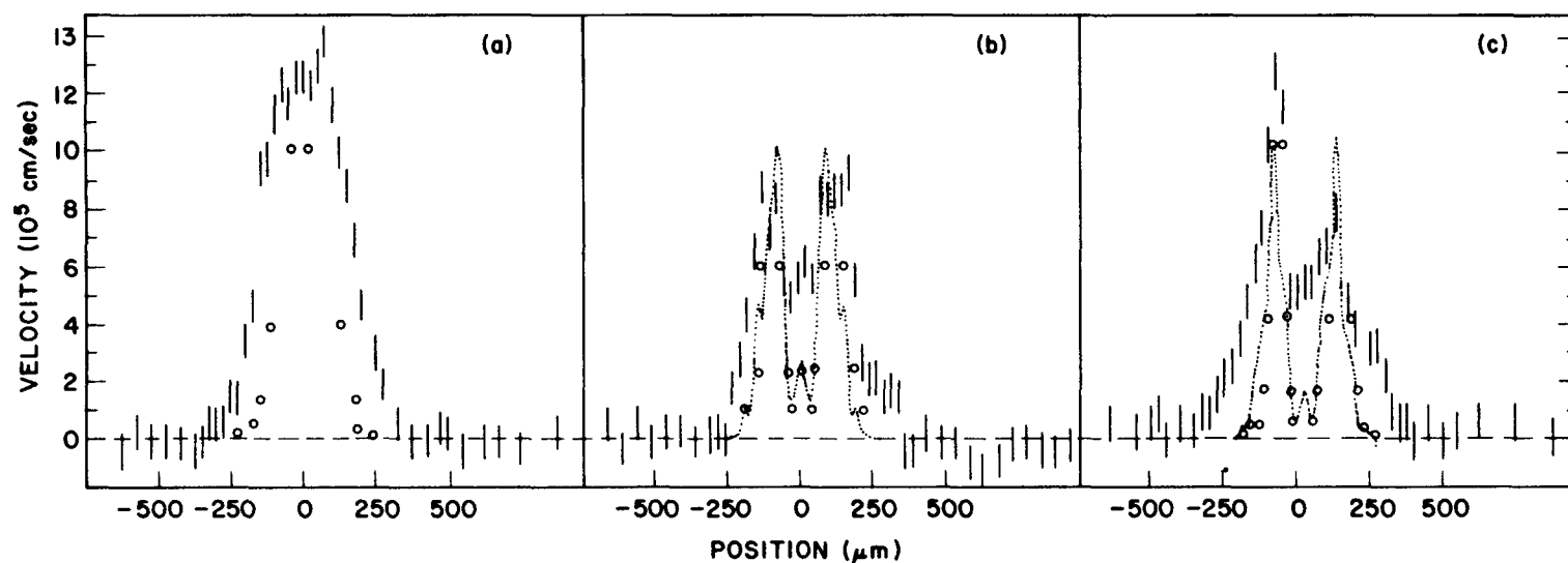
Fig. 2 — Doppler shift determined velocity profiles (vertical bars) for ablatively accelerated carbon targets at times near (within 300 psec) the peak of the main laser beam. The focused laser intensity profile measured at the target plane of an equivalent lens is given by the open circles, while the computed laser profile is given by the dotted lines. Case (a) corresponds to an unperturbed main laser beam, whereas in cases (b) and (c) 1 and 1.5 cm strips of opaque material were placed across the 10 cm diameter laser beam at the lens.
