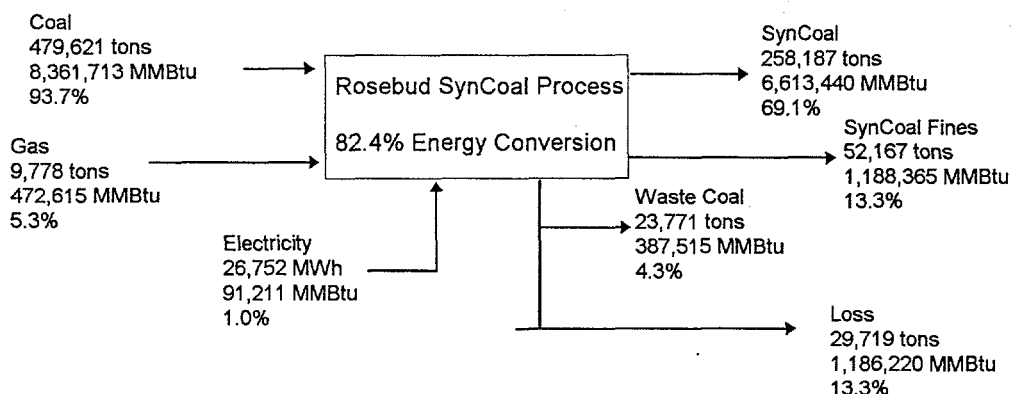
Figure 4.2 Yearly Summary of Material and Energy Balance
