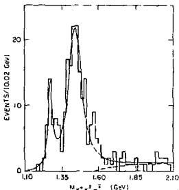
Fig. 17. K_S K^+ \pi^- invariant mass distribution with M_{K^+ K^-} < 1.04 GeV. Solid curve shows fit to mass spectrum. Dashed curve shows background distribution determined from fit. Data is from Ref. 40.
