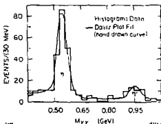
Fig. 4. Low-mass \gamma\gamma invariant mass combinations for \psi + 3\gamma events. (Crystal Ball)
