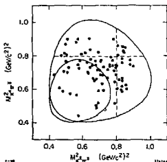
Fig. 10. Dalitz plot for events with 1.375 \leq M_{K\bar{K}\pi} < 1.500 GeV. Curves show low-mass and high-mass kinematic boundaries. Dashed lines show nominal K^* mass values. (Mark II)
