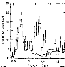
Fig. 7. \pi^+\pi^- invariant mass distribution for events satisfying (3). Histogram shows the expected feeddown from the \pi^+\pi^-\pi^0 final state as determined by Monte Carlo. (Mark II)
