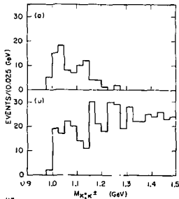
Fig. 11. K_S K^+ invariant mass distributions for events (a) in the signal region and (b) outside of the signal region. (Mark II)
