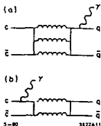
Fig. 2. Leading-order diagrams for radiative transitions from the \psi with (a) photon emission from the final-state quark line and (b) photon emission from the initial-state charmed quark line.
