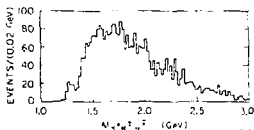
Fig. 16. K_S K^+ \pi^- invariant mass distribution for events satisfying (8). Data is from Ref. 40.
