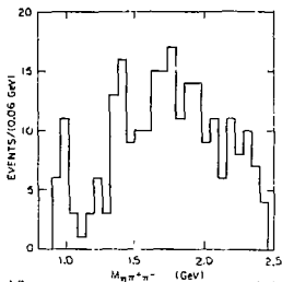
Fig. 13. n\pi^+\pi^- invariant mass distribution for events satisfying (6). (Crystal Ball)
