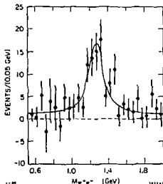
Fig. 8. \pi^+\pi^- invariant mass distribution after subtraction of \pi^+\pi^-\pi^0 feeddown. Curve is described in text. (Mark II)
