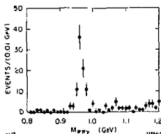
Fig. 5. \pi^+\pi^- invariant mass distribution for events satisfying (1) with \pi^0 combinations eliminated. (Mark II)
