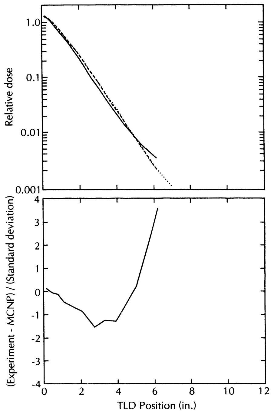
Fig. 6.8. For a Sn K-alpha source, the upper panel shows relative dose for a Hupmobile experiment as measured (solid line) and as modeled by MCNP (long dash line) and by COG (short dash line). The lower panel shows the difference between MCNP and experiment, as scaled to the total standard deviation.
