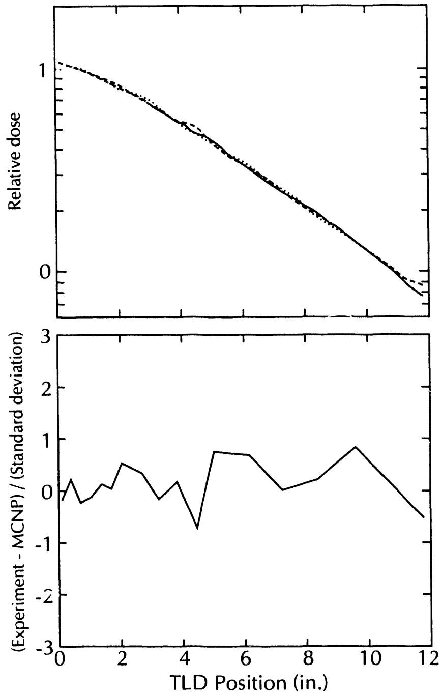
Fig. 6.3. For a ^{60}\text{Co} source, the upper panel shows relative dose for a Hupmobile experiment as measured (solid line) and as modeled by MCNP (long dash line) and by COG (short dash line). The lower panel shows the difference between MCNP and experiment, as scaled to the total standard deviation.
