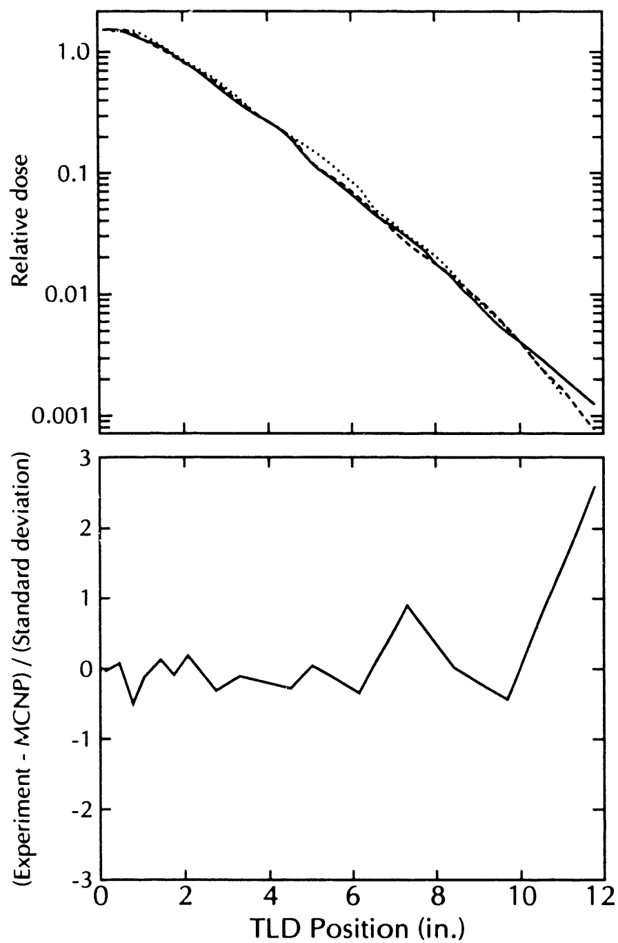
Fig. 6.6. For a ^{170}\text{Tm} source, the upper panel shows relative dose for a Hupmobile experiment as measured (solid line) and as modeled by MCNP (long dash line) and by COG (short dash line). The lower panel shows the difference between MCNP and experiment, as scaled to the total standard deviation.
