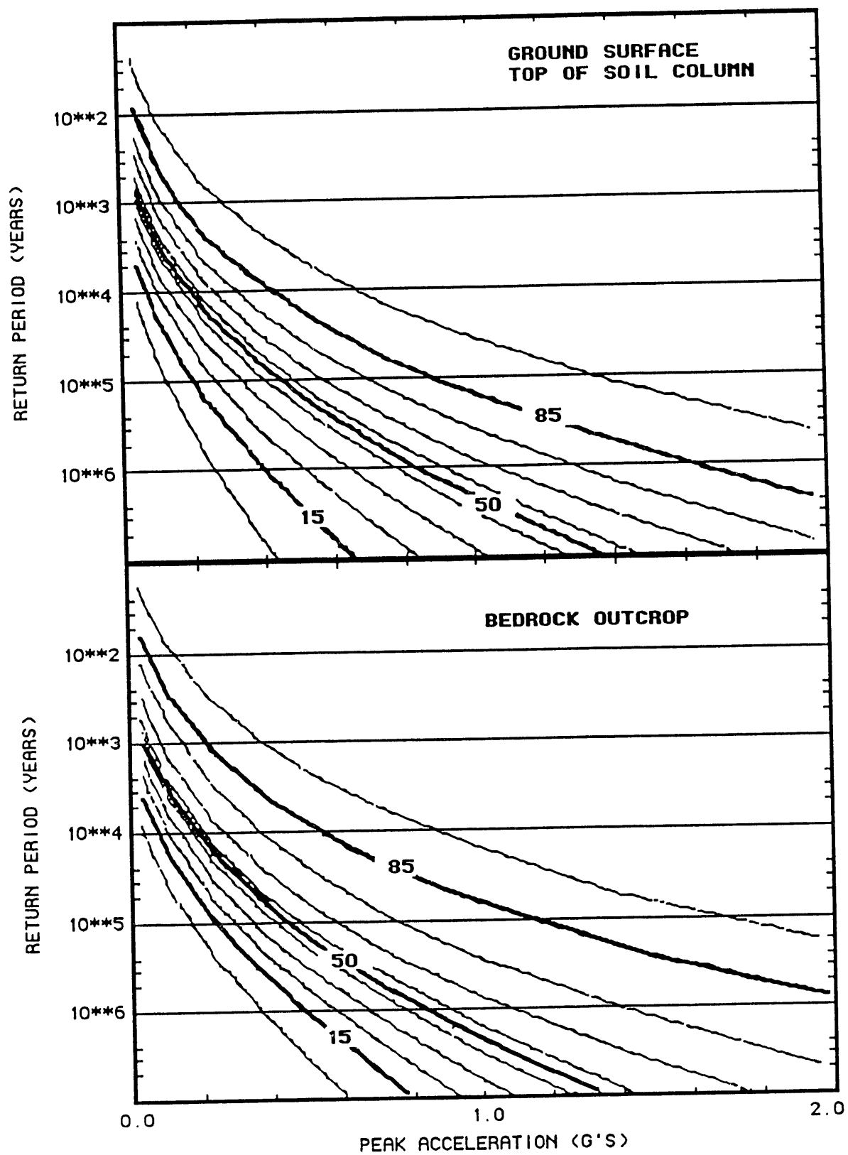
FIGURE 5 BEDROCK AND SURFACE HAZARD PREDICTION FOR HFBR SITE FROM LLNL USING 5 GM EXPERTS
