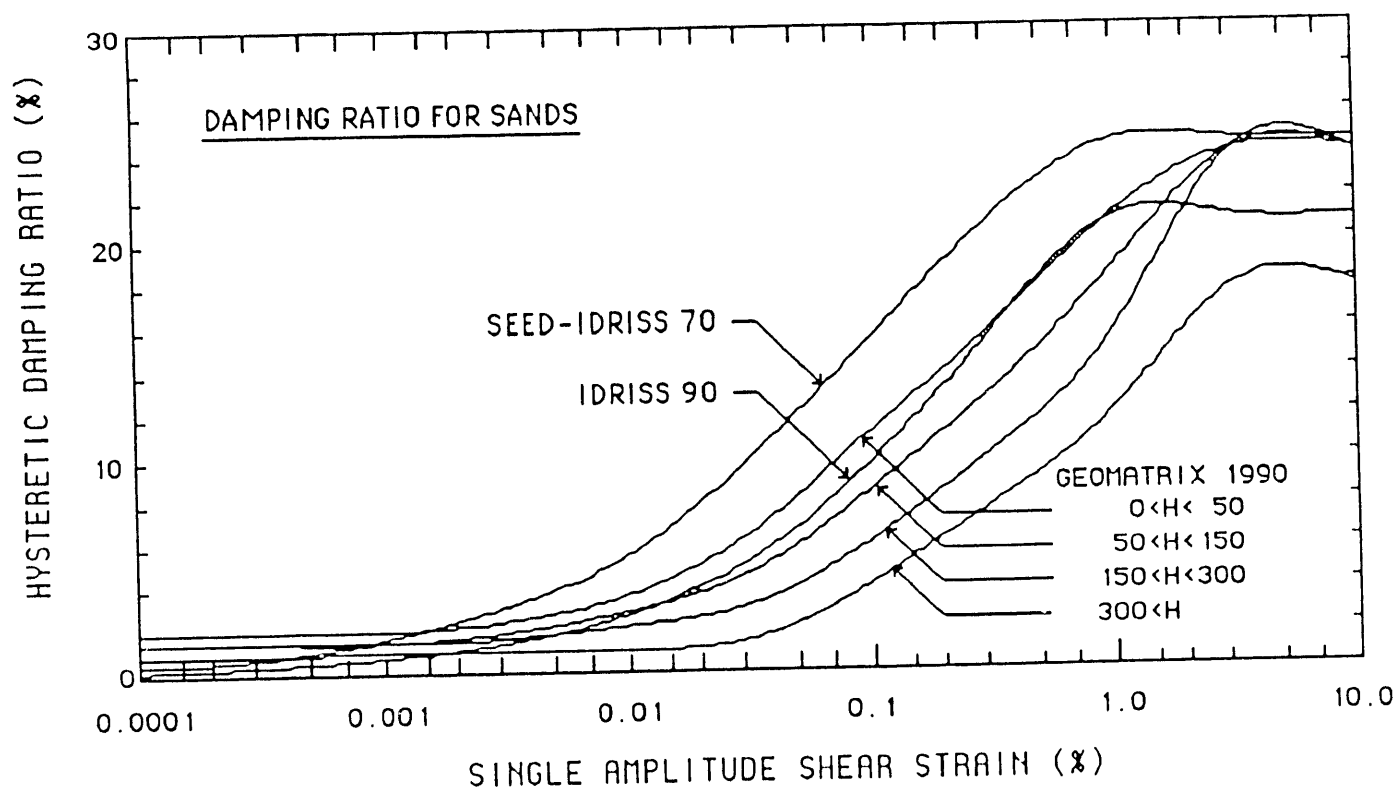
FIGURE 3 SHEAR DEGRADATION MODELS FOR SANDS
