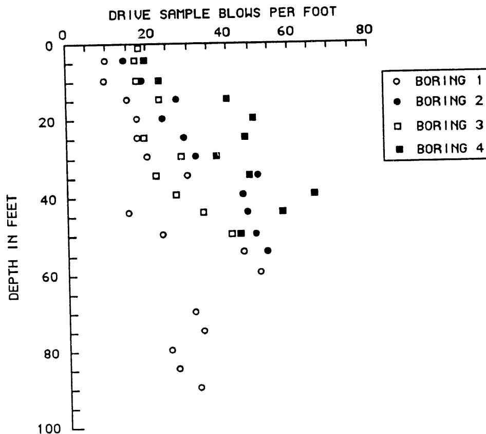
FIGURE 2 AVAILABLE DRIVE SAMPLE BLOWS PER FOOT
