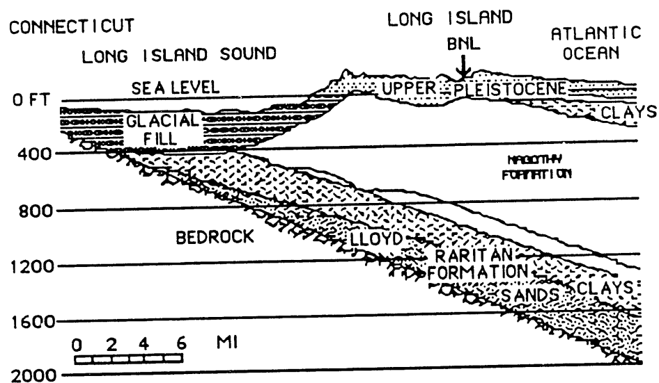
FIGURE 1 GENERALIZED CROSS-SECTION THROUGH BNL
