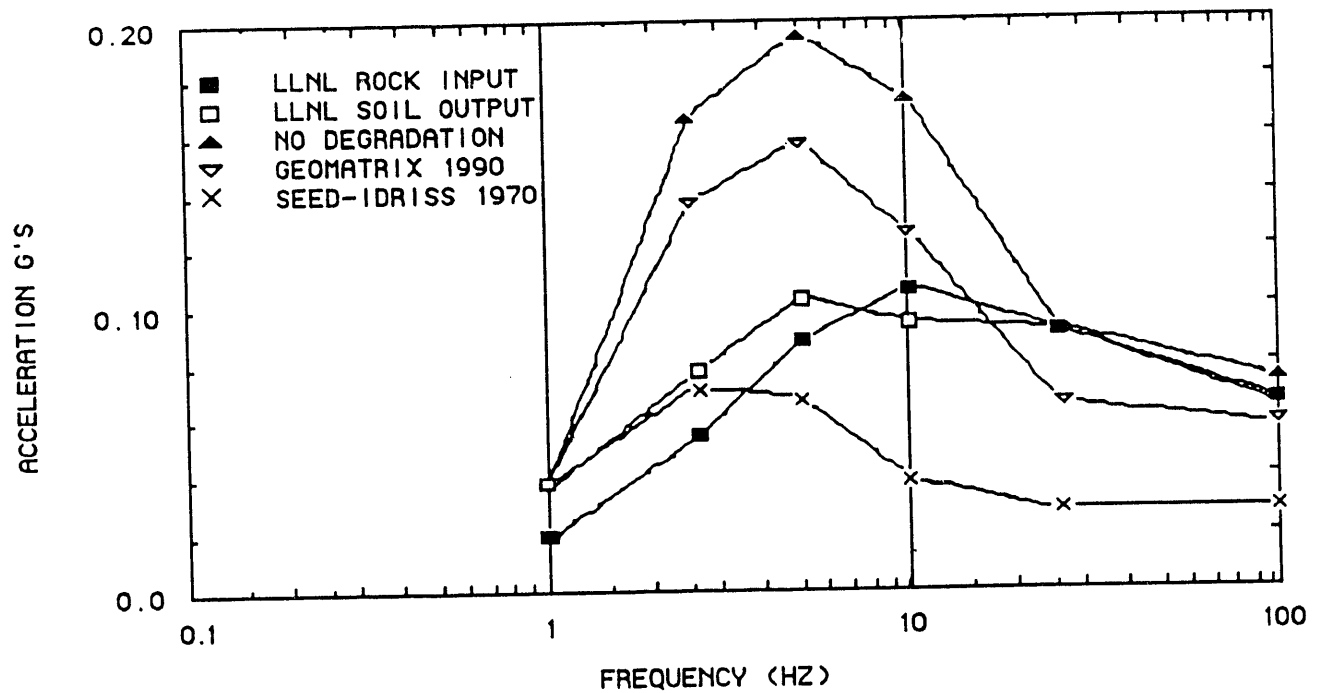
FIGURE 6 COMPUTED MEDIAN SURFACE SPECTRA FOR 1000 YEAR RETURN PERIOD AND 50TH PERCENTILE ROCK OUTCROP MOTION
