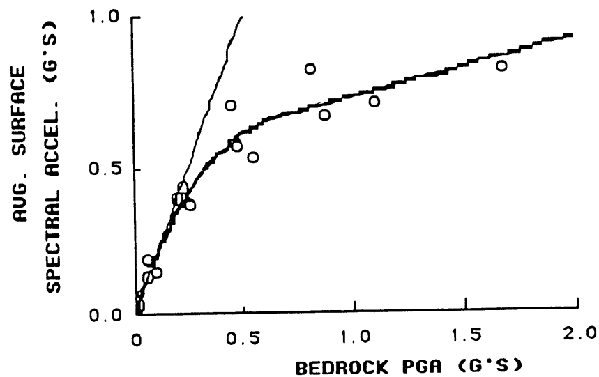
FIGURE 7 COMPUTED CONVERSION OF BEDROCK PGA TO SURFACE AVERAGE (5 TO 10 HZ) SPECTRAL ACCELERATION
