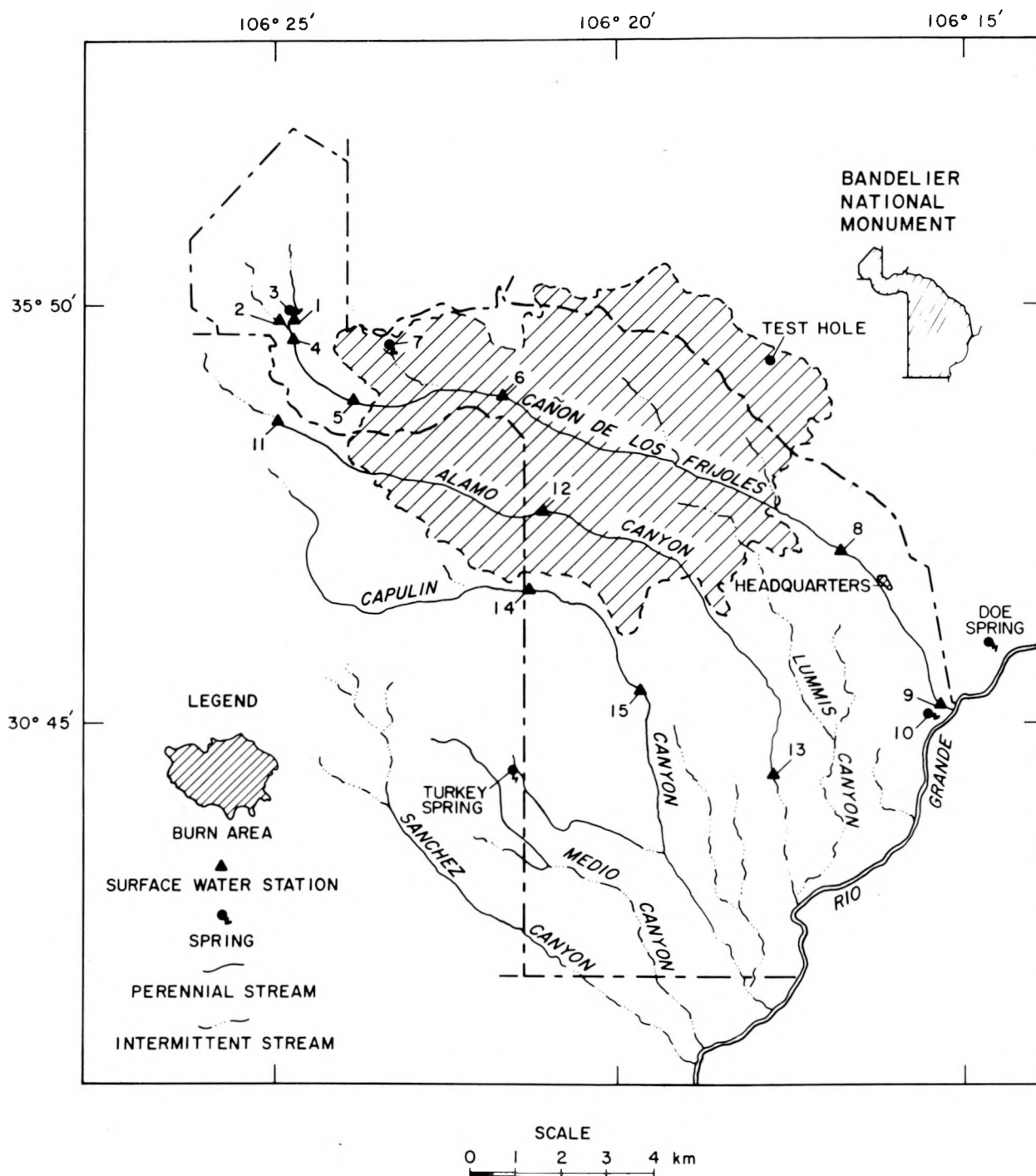
Fig. 4. Burn area and location of water sampling stations.
