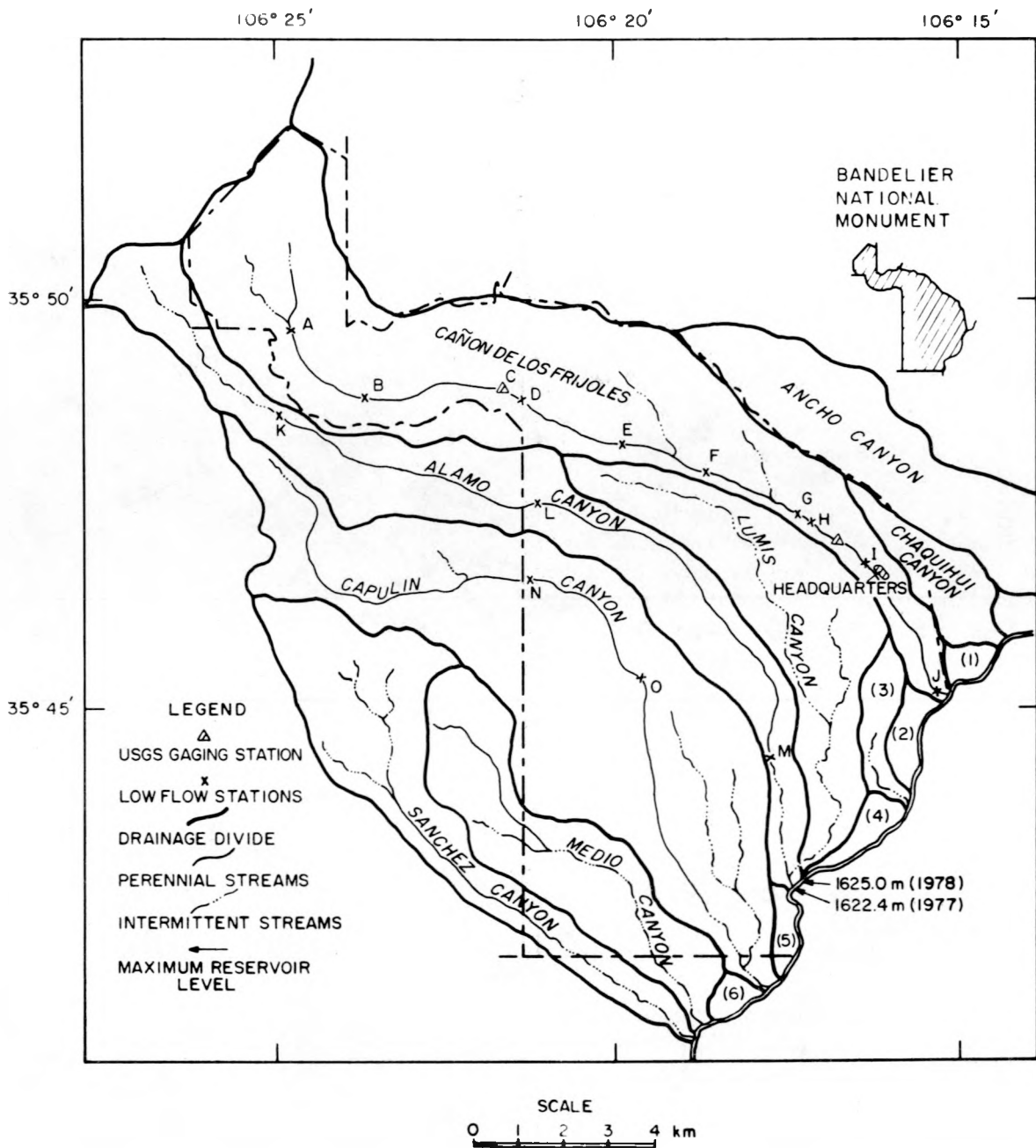
Fig. 3. Drainage area and location of hydrologic stations.
