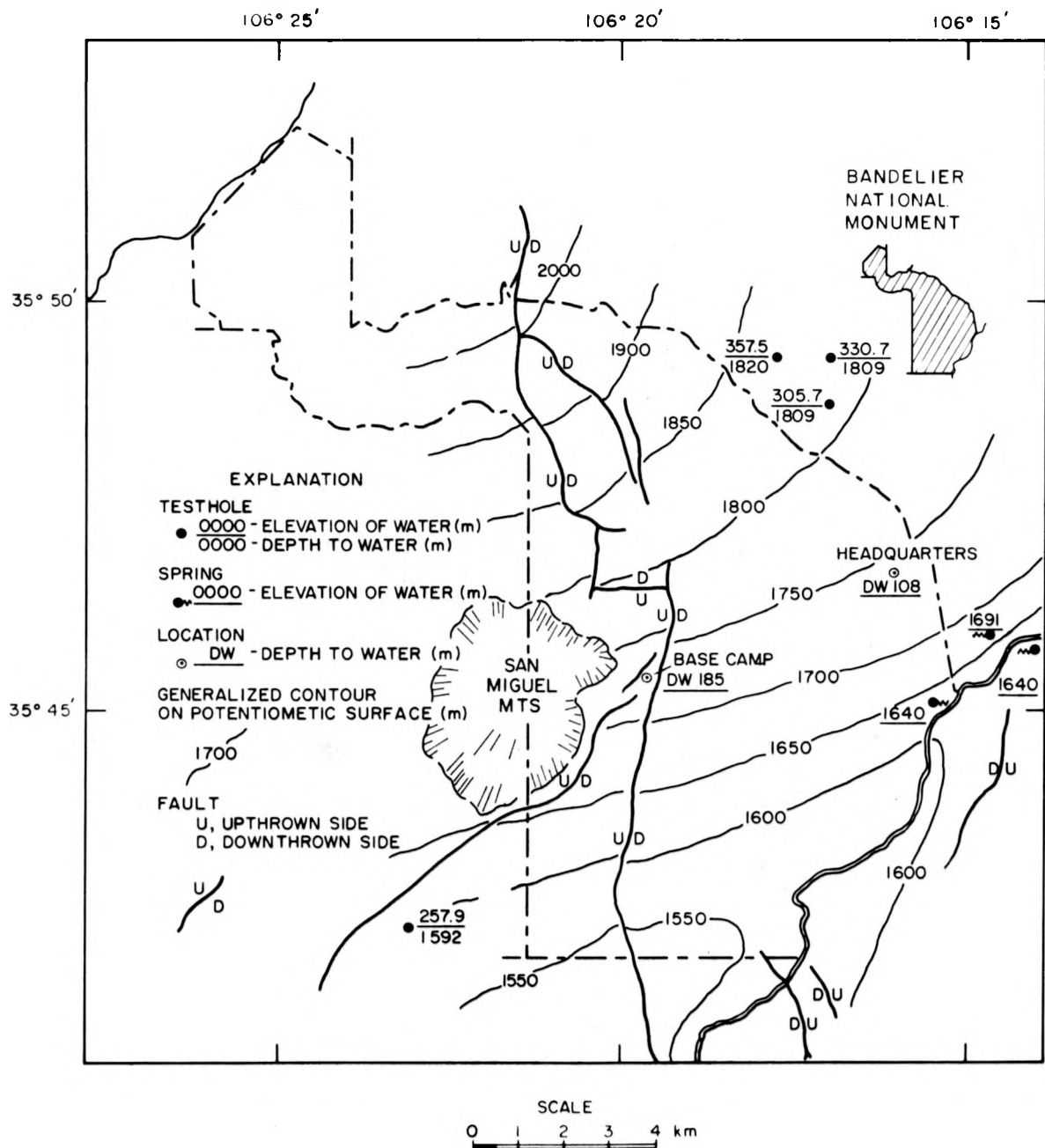
Fig. 5. Generalized contours on the potentiometric surface of the main aquifer.
