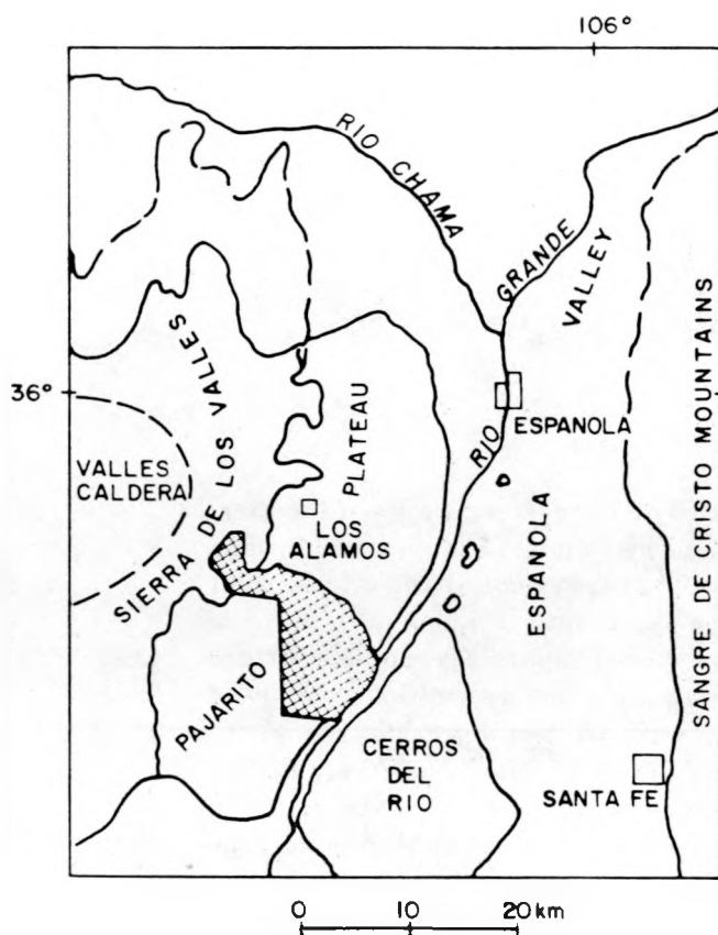
Fig. 1. Physiographic features in the vicinity of Bandelier National Monument.
