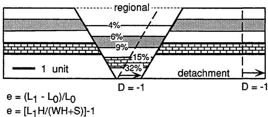
Figure 5.--Structural diagrams showing area-depth-strain relationships in extensional structures (modified from Groshong, 1994; Pashin and others, 1995).
