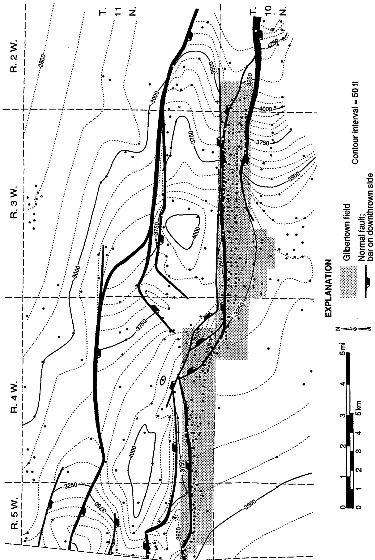
Figure 20.--Structural contour map of the top of the Eutaw Formation, Gilbertown Field and adjacent areas.
