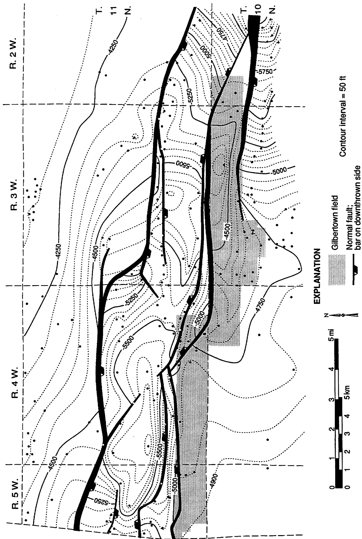
Figure 19.--Structural contour map of the top of the lower Tuscaloosa Group, Gilbertown Field and adjacent areas.
