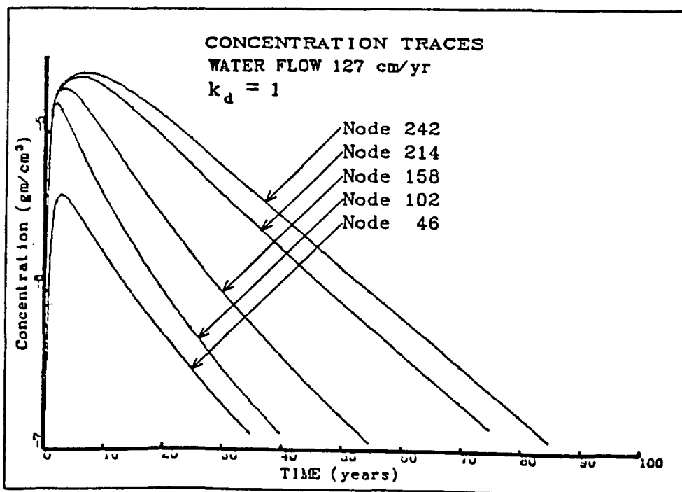
Figure 8 Plot of concentration versus time along the trench bottom for the case where the water influx is 127 cm/yr, k_d=1 , and a_1=213.0 cm.
