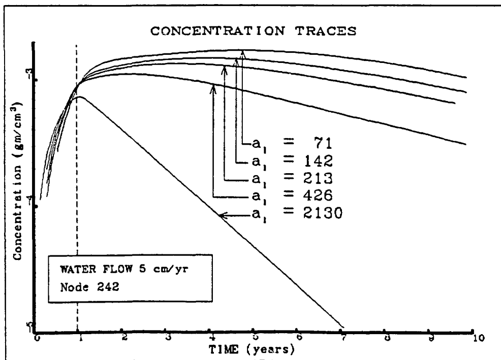
Figure 6 Plot of concentration versus time at the center of the trench, node 242, for various values of the dispersion coefficient.
