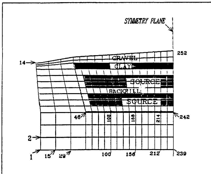
Figure 1 Finite element nodalization scheme used by FEMWASTE-1 in the radionuclide transport studies. Numbers in the figure refer to node numbers. The bottom of the trench begins at node 46 and ends at node 242.
