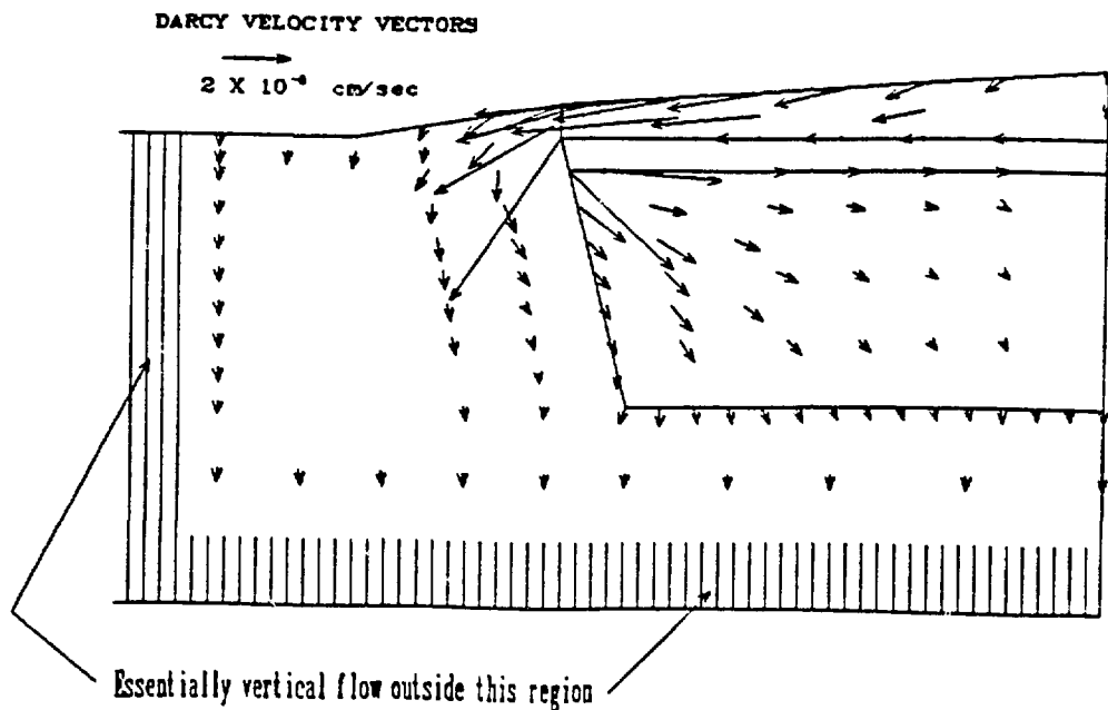
Figure 2 Darcy Velocity vectors for the 127 cm/yr water influx case.
