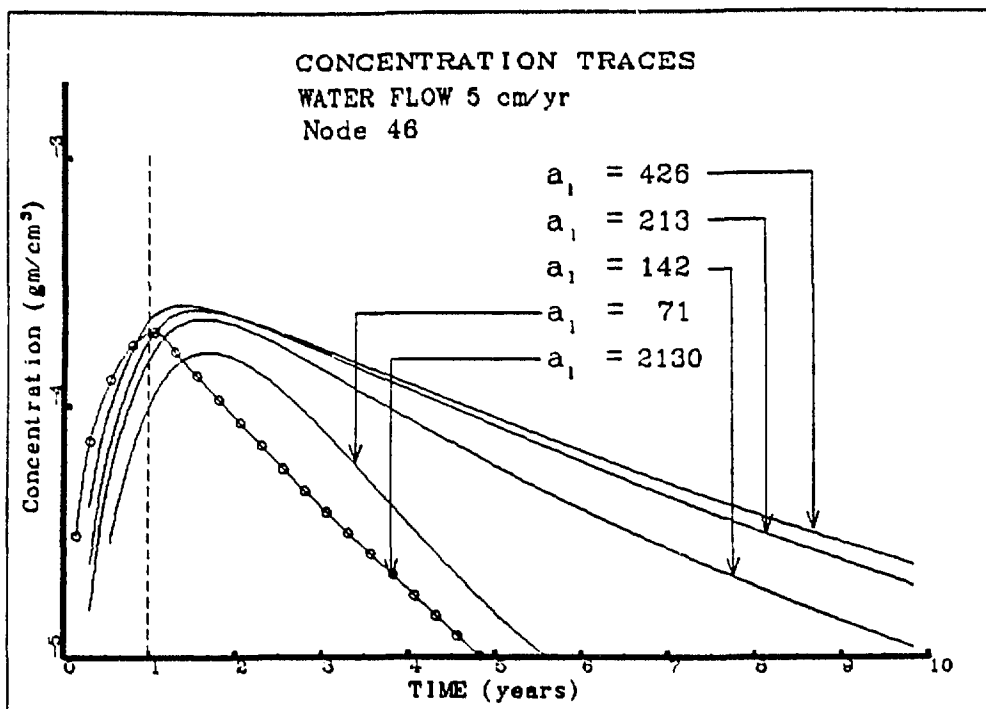
Figure 5 Plot of concentration versus time at the lower left corner of the trench, node 46, for various values of the dispersion coefficient.
