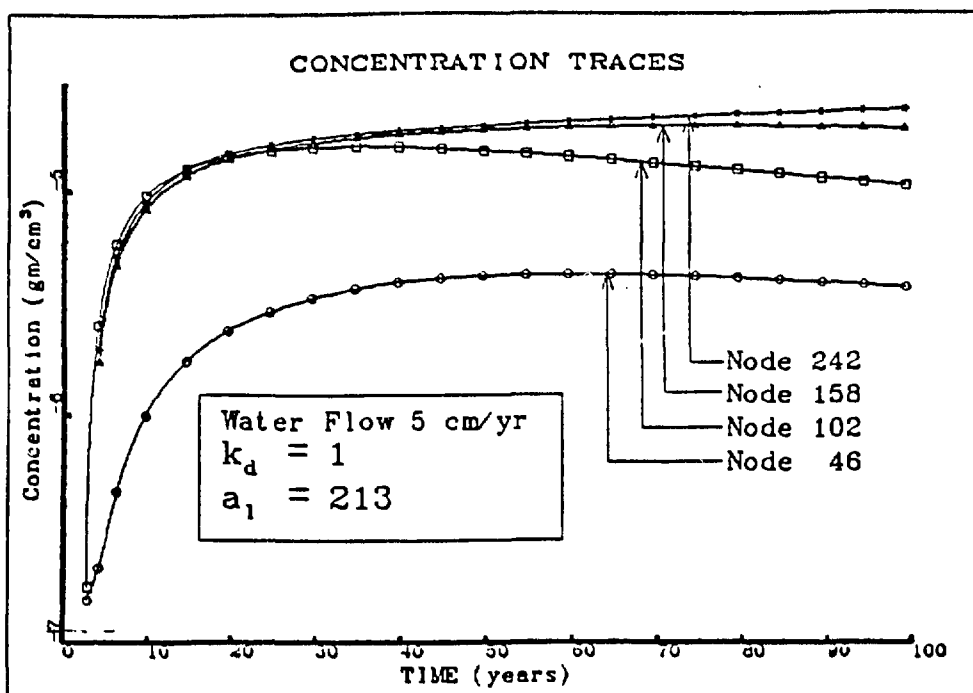
Figure 7 Plot of concentration versus time along the trench bottom for the case where the water influx is 5 cm/yr, k_d=1 , and a_1=213.0 cm.
