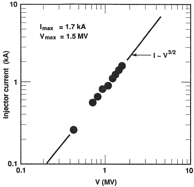
Figure 4. Injector current vs voltage for the 8.9-cm-diam cathode.
