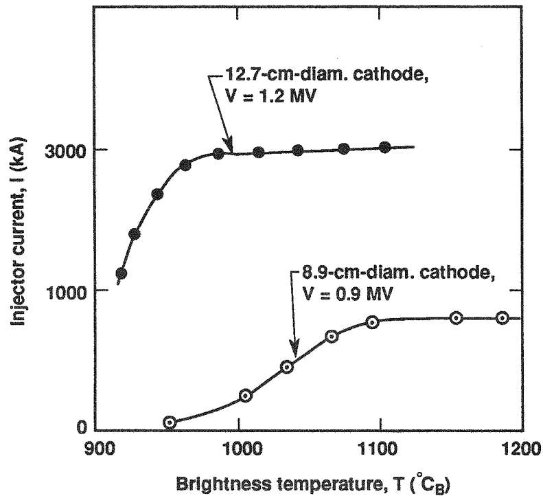
Figure 3. Emission current vs temperature for the (a) 8.9-cm- and (b) 12.7-cm-diam cathodes.
