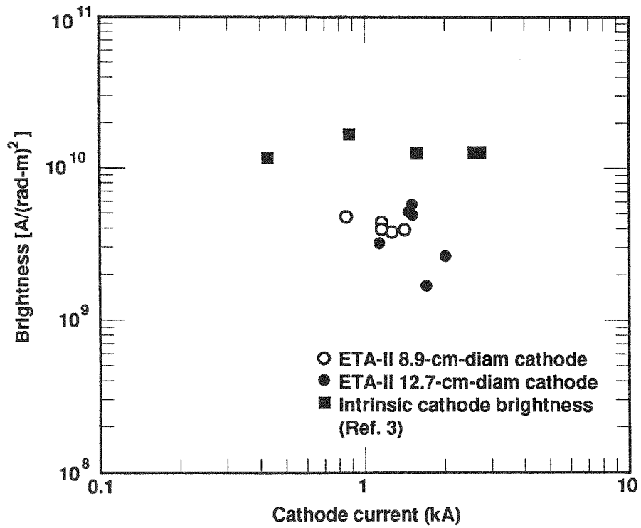
Figure 5. Brightness vs accelerator current.
