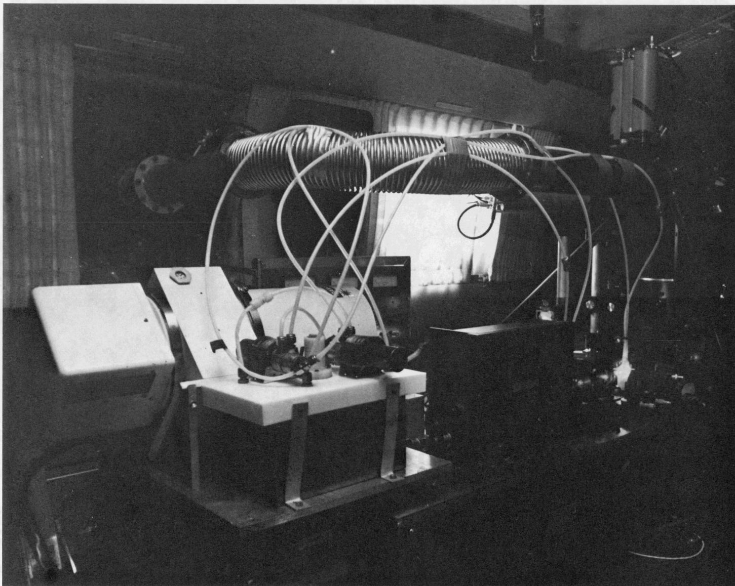
Figure 4. Georgia Tech OH Laser Probe mounted on the NCAR Electra
