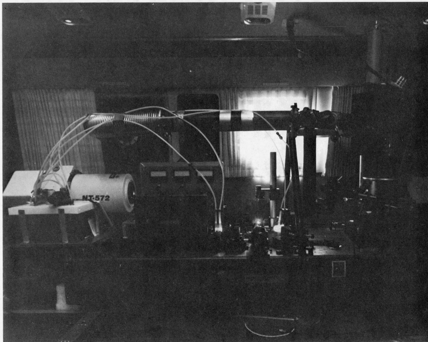
Figure 3. Georgia Tech OH Laser Probe Mounted on the NCAR Electra
