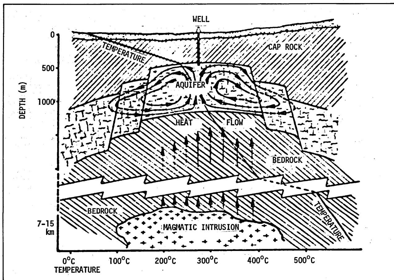
Fig. 1. Basic model of a steam field. (Facca, 1973)
