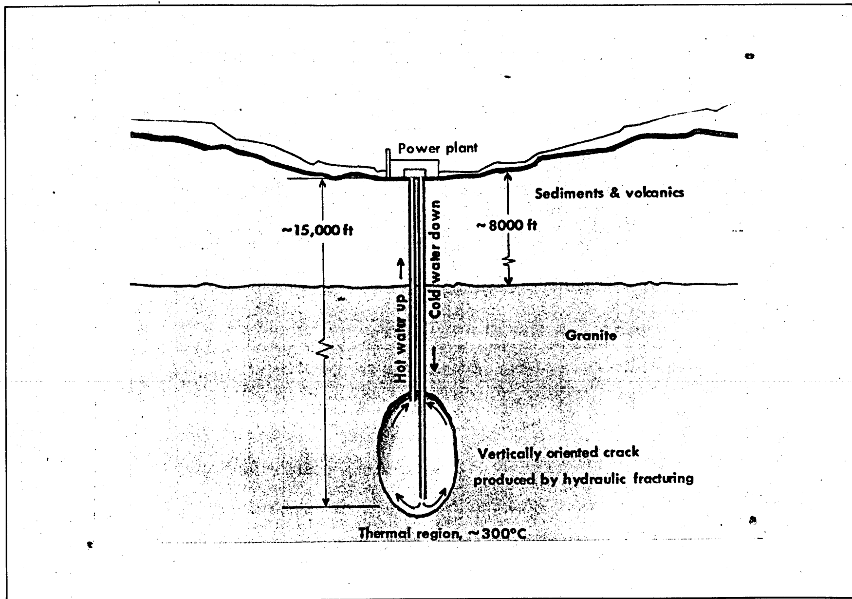
II Fig. 5. Typical pressurized-water circulation loop for energy extraction in the western United States. (Smith, 1974)
