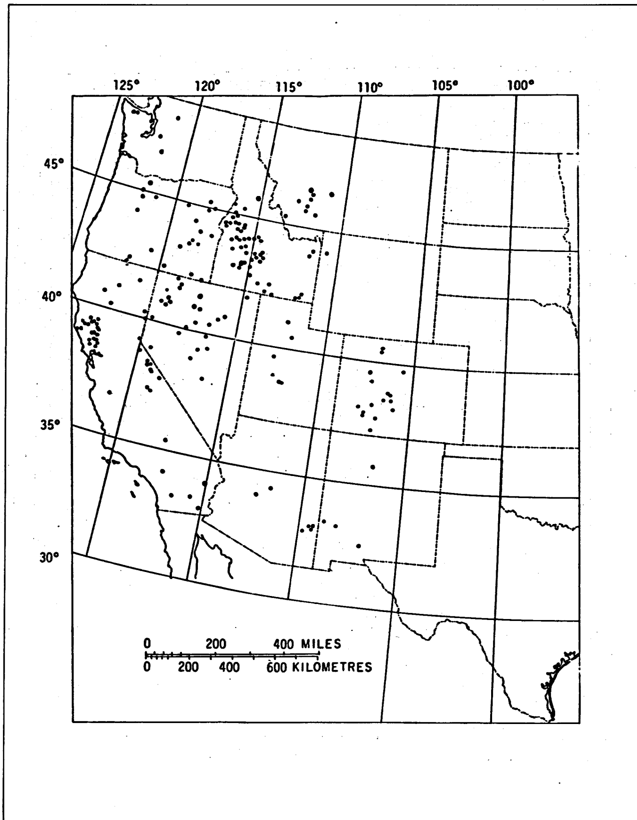
Fig. 4. Location of hydrothermal convection systems in the conterminous United States with indicated subsurface temperatures between 90^{\circ} and 150^{\circ}\text{C} . (White and Williams, 1975)
