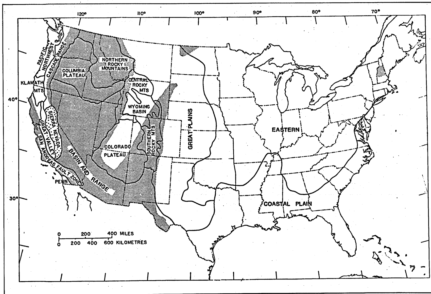
Fig. 8. Map showing probable extent of hot (stippled), normal (white), and cold (dotted) crustal regions of the United States based on data in Figs. 9 and 10. Physiographic provinces (largely generalized from Fenneman (1946)) do not necessarily represent heat-flow provinces. (White and Williams, 1975)
