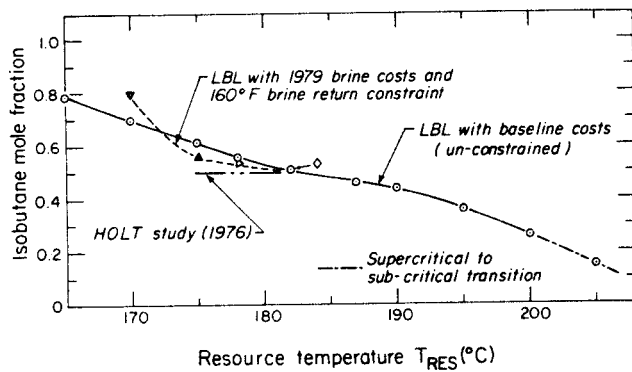
FIG. 1 Computed optimum iC_4 mole fraction as a function of resource temperature. The optimum composition also depends on turbine constraints (not shown).
