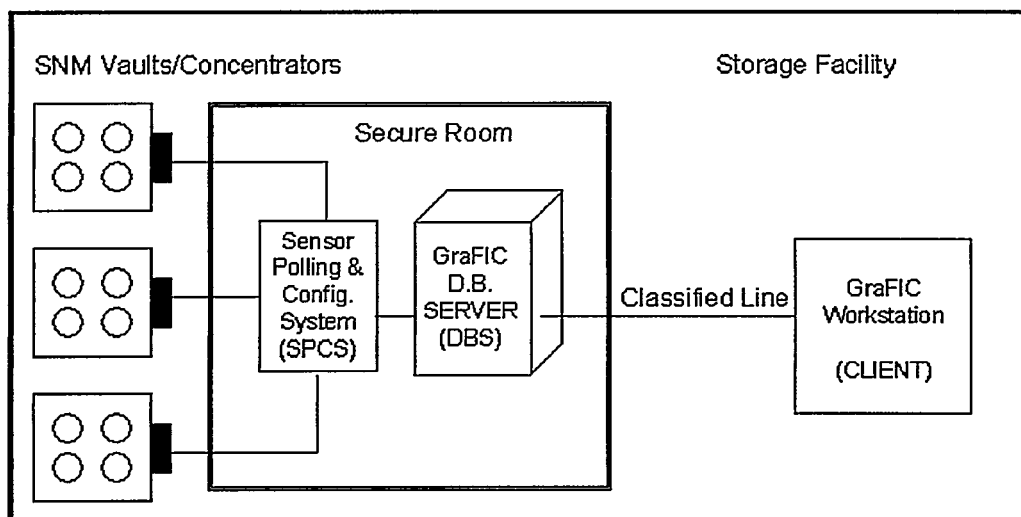
Figure 2 - Example GraFIC™ System Layout
