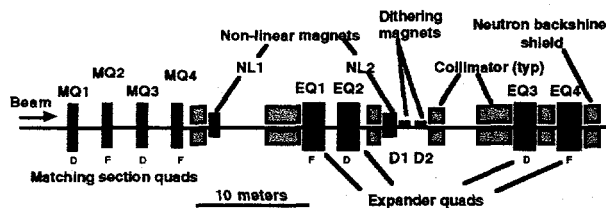
Fig. 2. Beam expander optics.
