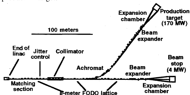
Fig. 1. The overall layout of the APT beam delivery system.
