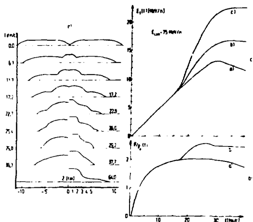
Fig. 22. (a) The density distribution of various stages of a central collision of two equal nuclei E_{lab}=75 MeV/n. The left-hand shows \rho(z) for a normal equation of state K_0=300 MeV): the second central region quickly expands again. The right-hand side shows the strong density increase in the case of a density isomeric state: a large part of the system stays rather long within the abnormal phase (density isomer at \rho_c \approx 2\rho_0, \rho_1 = 2.5 \rho_0, B_1 = 0 ). (b) The central compression \rho/\rho_0(t) increases strongly above the critical density for the production of an isomeric state: compared to the normal nuclear matter (lower curve), the presence of a density isomer leads to the collapse of the nuclear matter into the abnormal superdense phase (upper curve). Thus the matter remains much longer within the strongly compressed state. (c) The gain of condensation energy leads to a strong increase of the mean thermal energy \Sigma_T(t) in the presence of a density isomer (upper curve). Lower curve: normal nuclear matter.
