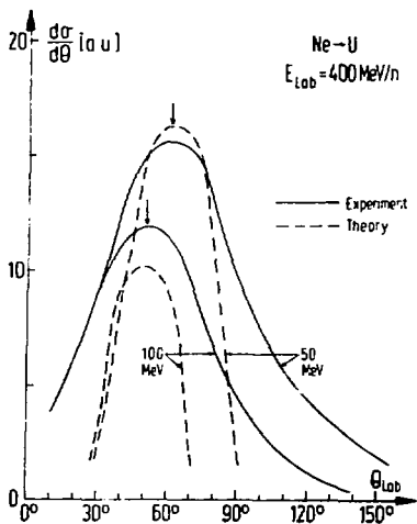
Fig.29. The experimental angular distributions (full curves) are compared to the theoretical obtained curves (dashed).
