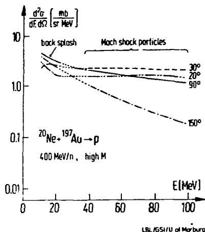
Fig. 30. The experimentally obtained double differential cross section d^2\sigma/d\Omega dE for \text{Ne}+\text{Au} at 400 MeV/n triggering for the high multiplicities as obtained by Meyer et al. (1979).
