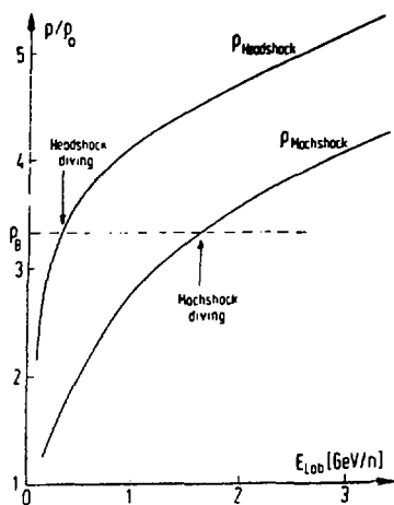
Fig. 39. The diving of head shock and Mach shock into a possible second minimum of the equation of state. The head- and Mach shock densities as a function of projectile energy. p_B indicates the position of the assumed 2nd minimum in E_c(\rho) .
