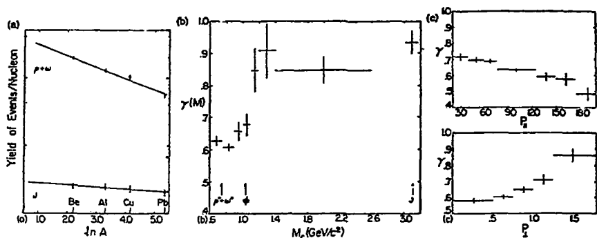
(a) A dependence of yields of p+\omega and J . Straight lines are least-squares fits to the data. Error bars are statistical only. (b) A dependence of the dilepton yield as a function of mass; cross-section per nu-
