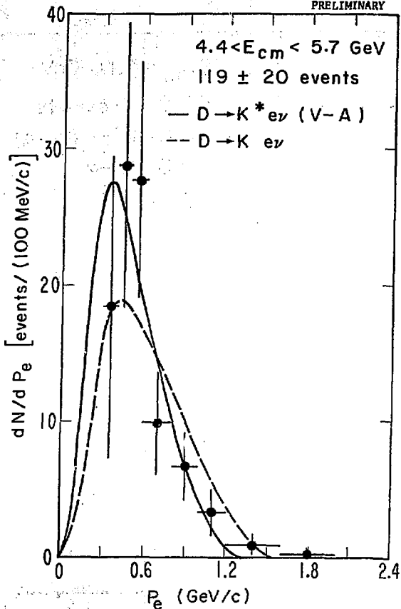
Fig. 9 The corrected momentum distribution above 300 MeV/c for the electrons in the multiprong events in the E_{c.m.} region 4.4-5.7 GeV. The ~15% heavy lepton contribution has not been subtracted. The curves show the electron momentum spectra expected from D meson production (via e^+e^- \rightarrow D^*D^* ) and decay (via D \rightarrow K e \nu and K^* e \nu (V-A)), based on the calculations of Ali and Yang. 28 The curves are normalized above 300 MeV/c to the total number of events.
