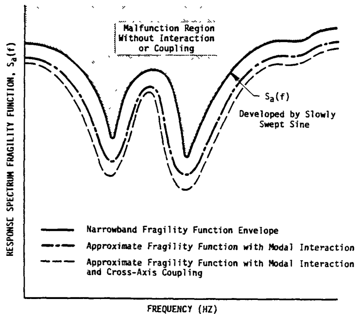
FIGURE 6. FRAGILITY FUNCTIONS FOR A COMPLEX FLEXIBLE DEVICE
