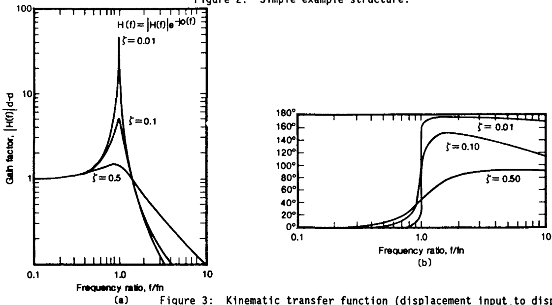
Figure 3: Kinematic transfer function (displacement input to displacement output, velocity input to velocity output, acceleration input to acceleration output) for a damped simple harmonic oscillator for damping values of 1%, 10%, and 50% of critical (a) Gain factor, (b) Phase factor.
