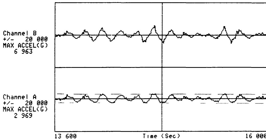
Figure 5 Unsaturated Time Signal and Saturated
