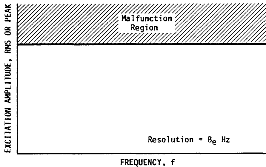
FIGURE 2. NARROWBAND FRAGILITY FUNCTION FOR RIGID THRESHOLD DEVICE
