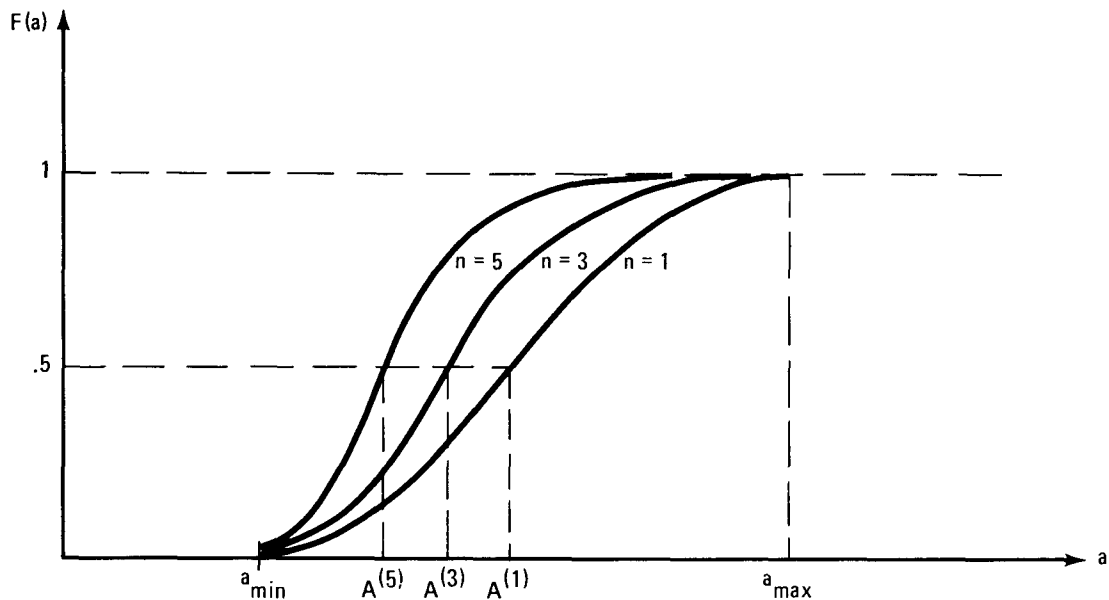
Figure 5 PLANT FRAGILITY FOR n OVERLAPPING COMPONENT FRAGILITY
