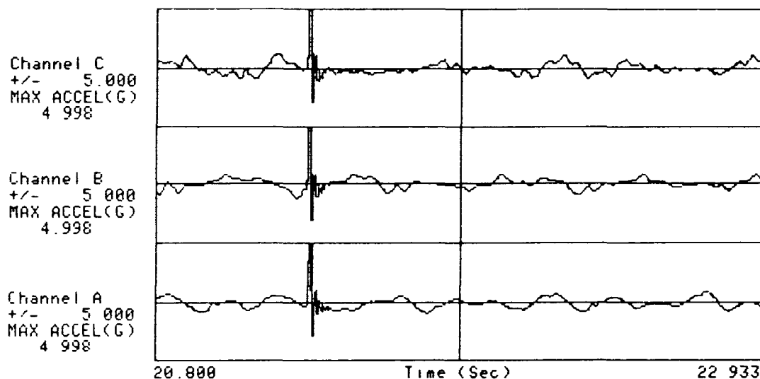
Figure 1 Sharp Impact
