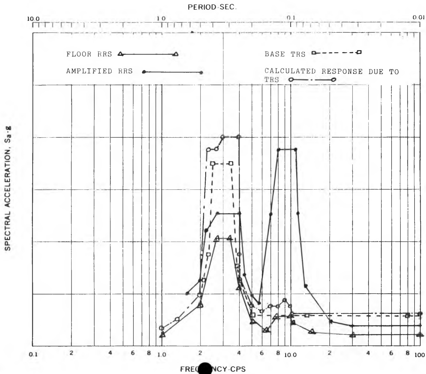
FIGURE 6 EFFECT OF BASE MOTION CHARACTERISTICS ON PANEL RESPONSE
