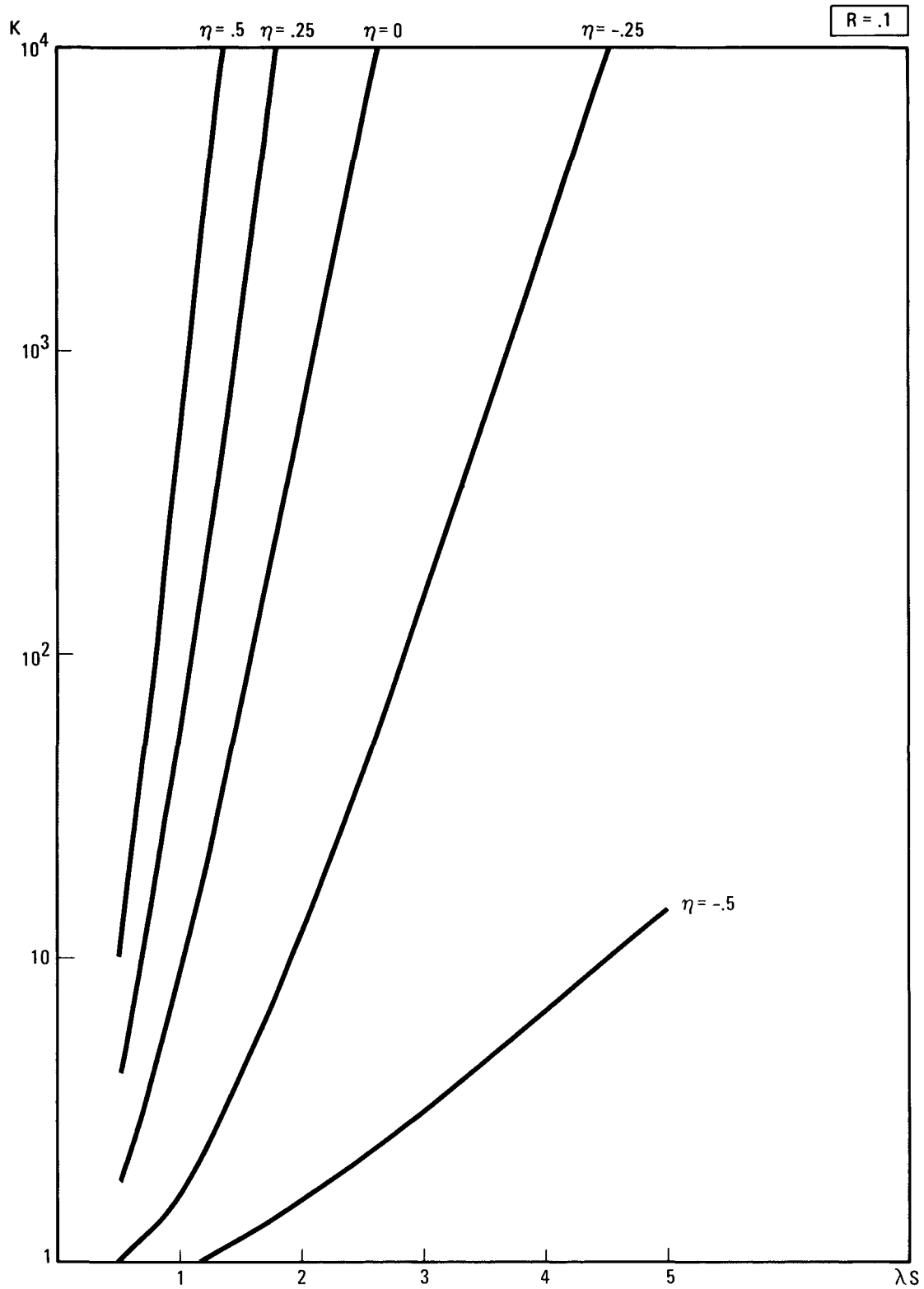
Figure 2 FRAGILITY SPREAD FACTOR FOR R = .1
