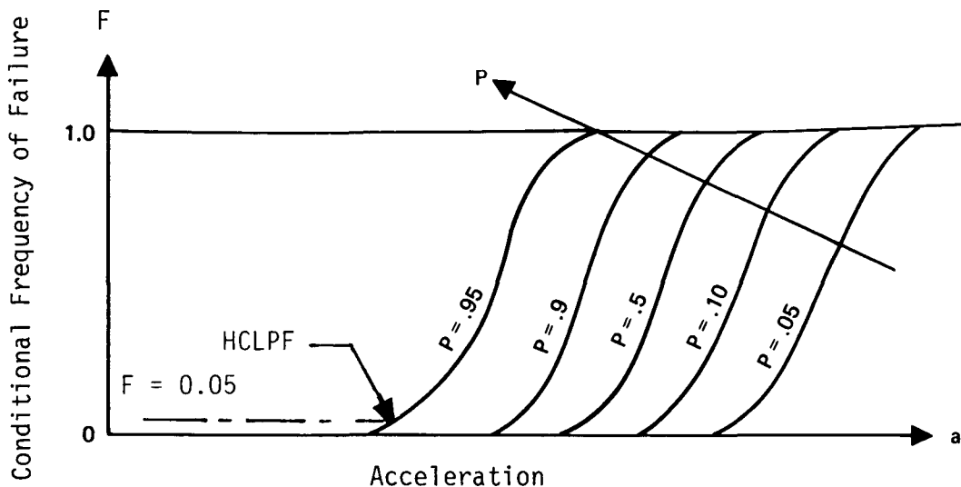
Figure 1. Fragility Curves
