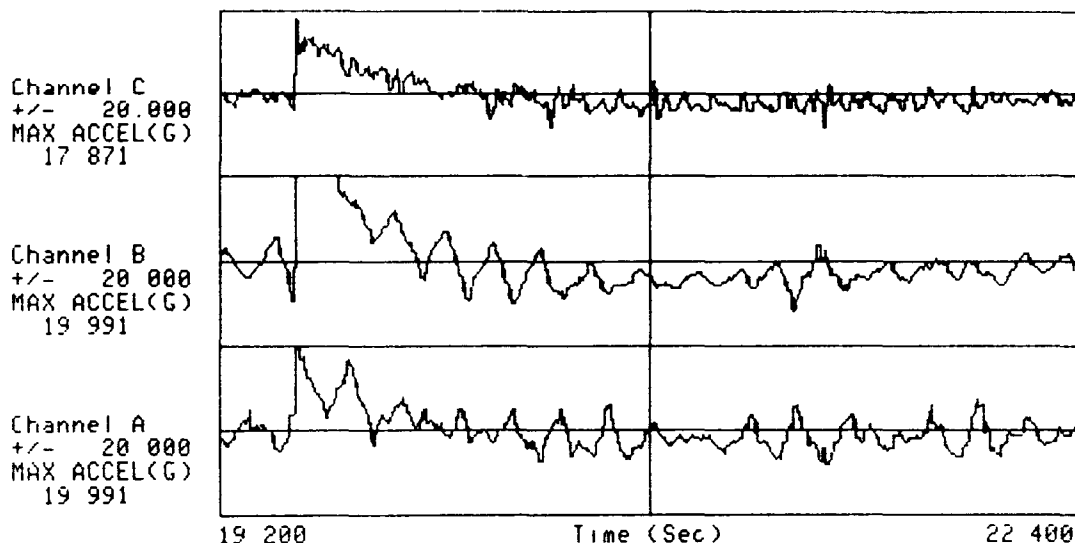
Figure 2 Impact Similar to D.C. Field Collapse or Over Ranging of an Accelerometer
