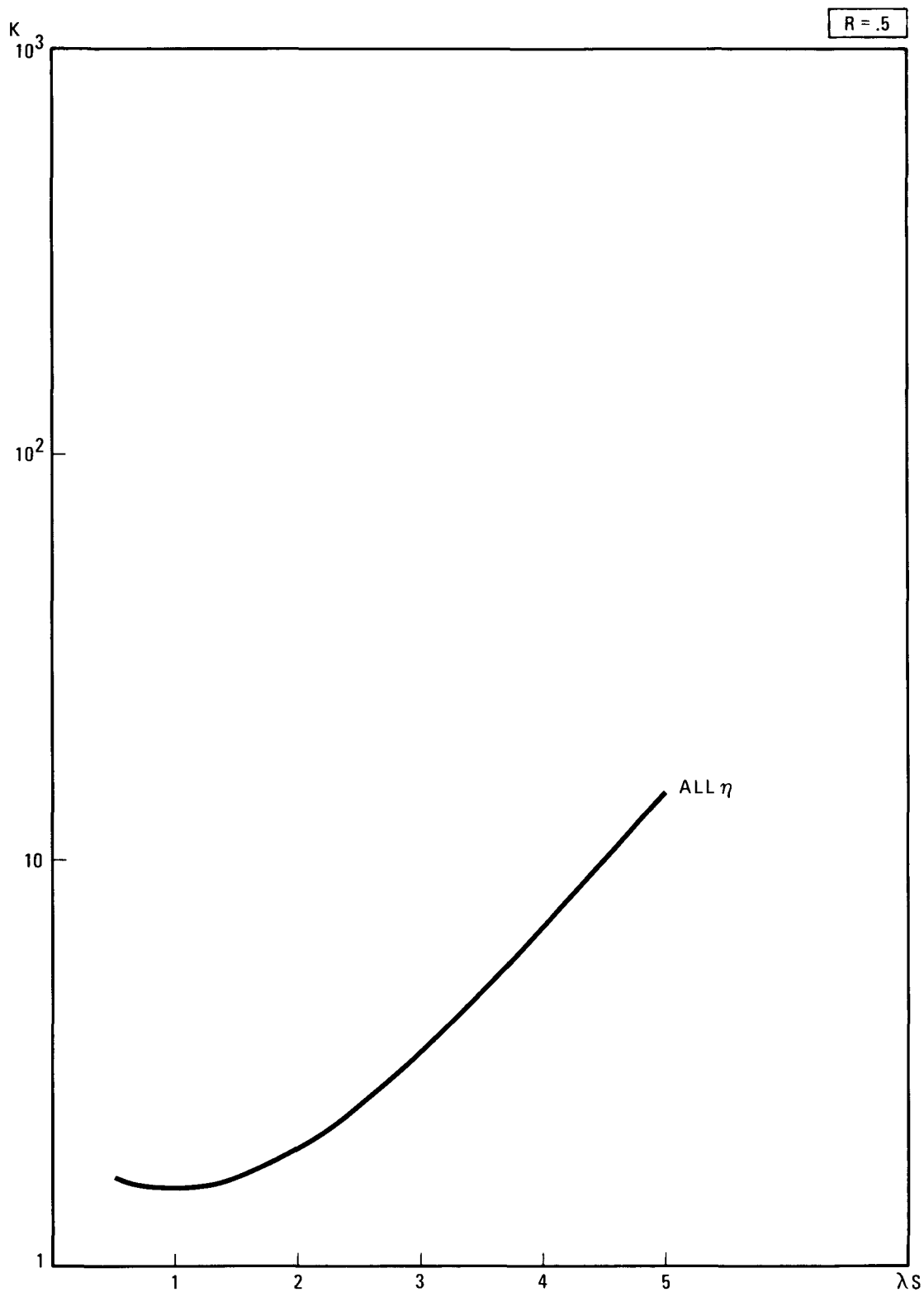
Figure 4 FRAGILITY SPREAD FACTOR FOR R = .5
