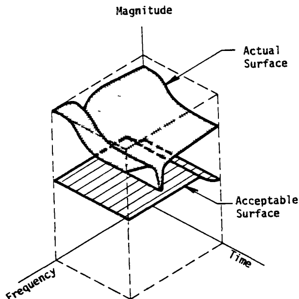
FIGURE 1. GENERALIZED DYNAMIC FRAGILITY SURFACE
