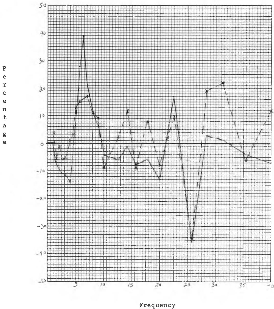
Figure 8 Normalized TRS Top Cabinet Acceleration X - X \left( \frac{\text{Vector}}{\text{Triaxial}} \right) \quad \text{---} \quad \left( \frac{\text{Biaxial}}{\text{Triaxial}} \right)
