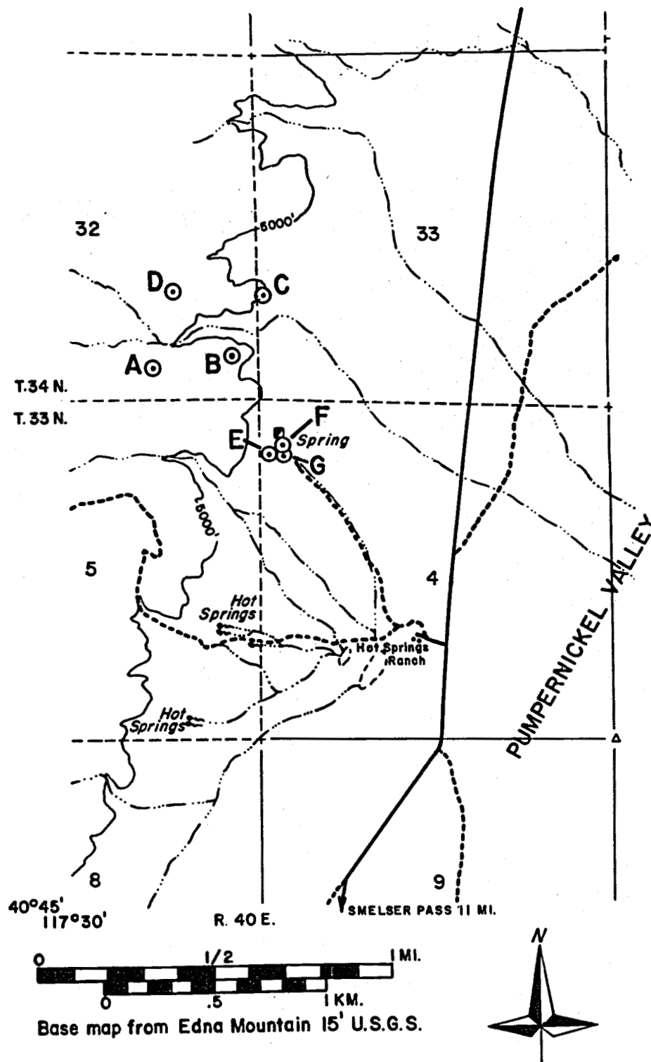
Figure A6. Location of mineral exploration wells in Pumpnickel Valley.
