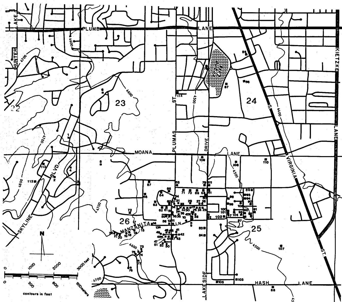
Figure C8. Location of thermal wells in the Moana area.
