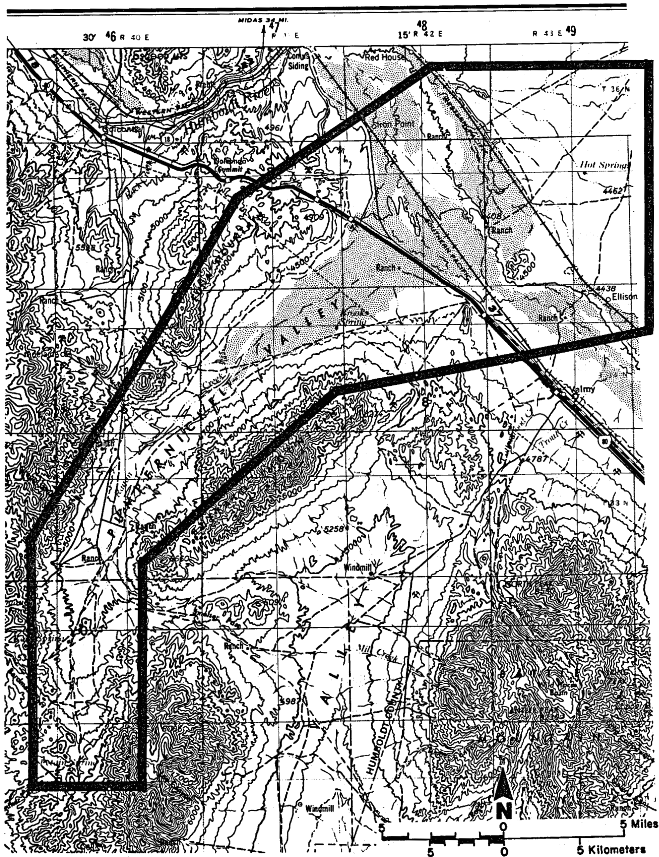
Figure A1. Pumpnickel Valley study area.
