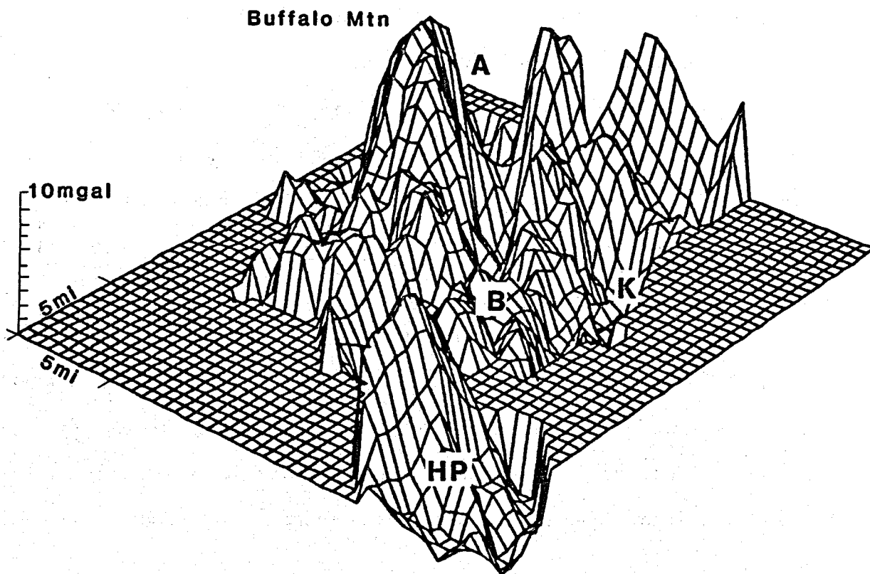
Figure A11. 3-dimension computer generated residual gravity map of Pumpnickel Valley, looking southwest: B, Brooks Spring; HP, Blossom Hot Pot; K, Kemp thermal anomaly (NCAR plot).
