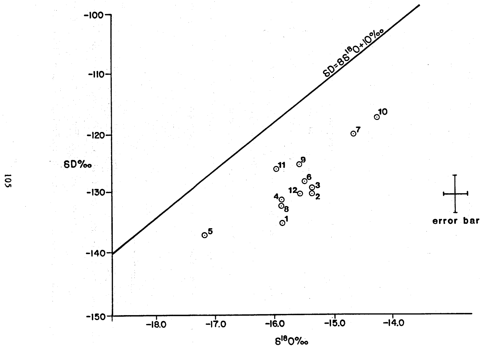
Figure B11. Stable light isotope composition of Carlin waters. Worldwide meteoric water line after Craig (1963).
