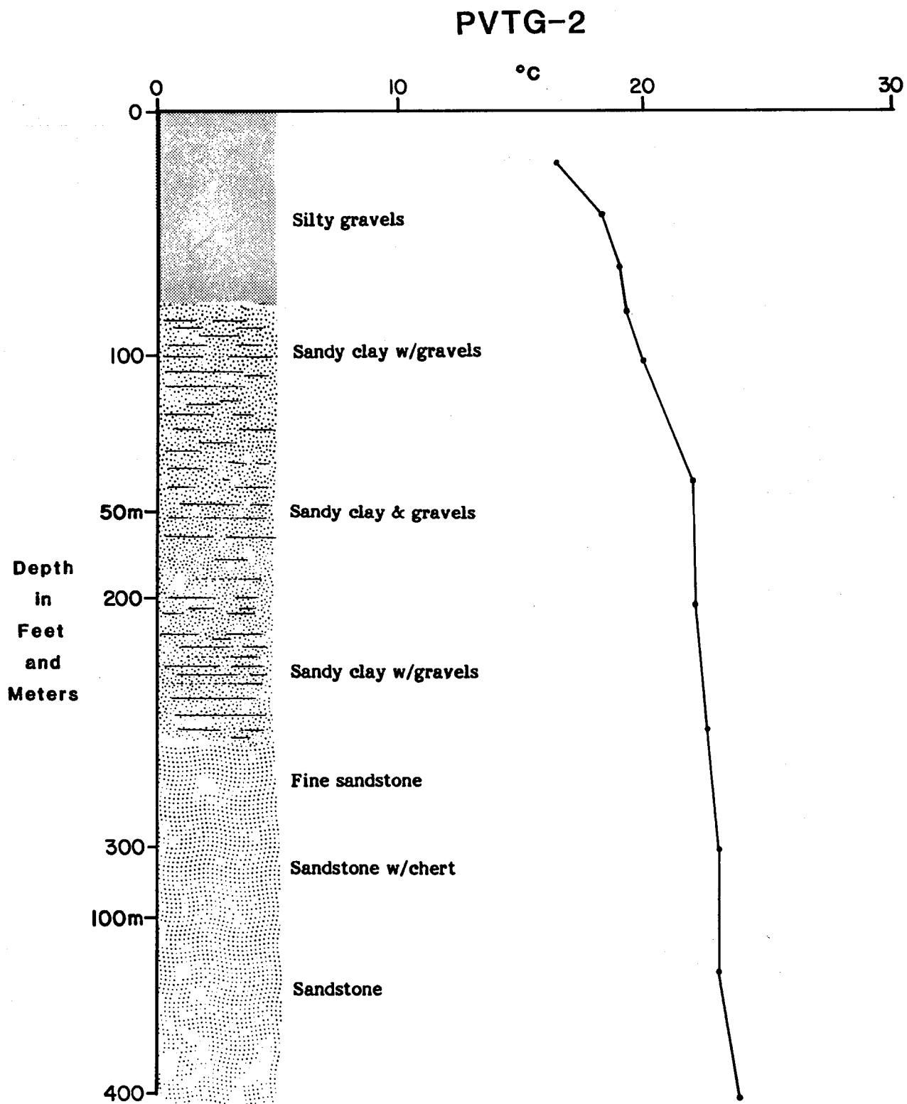
Figure A27. Lithologic log and temperature-depth profile of PVTG-2 in Pumpernickel Valley.
