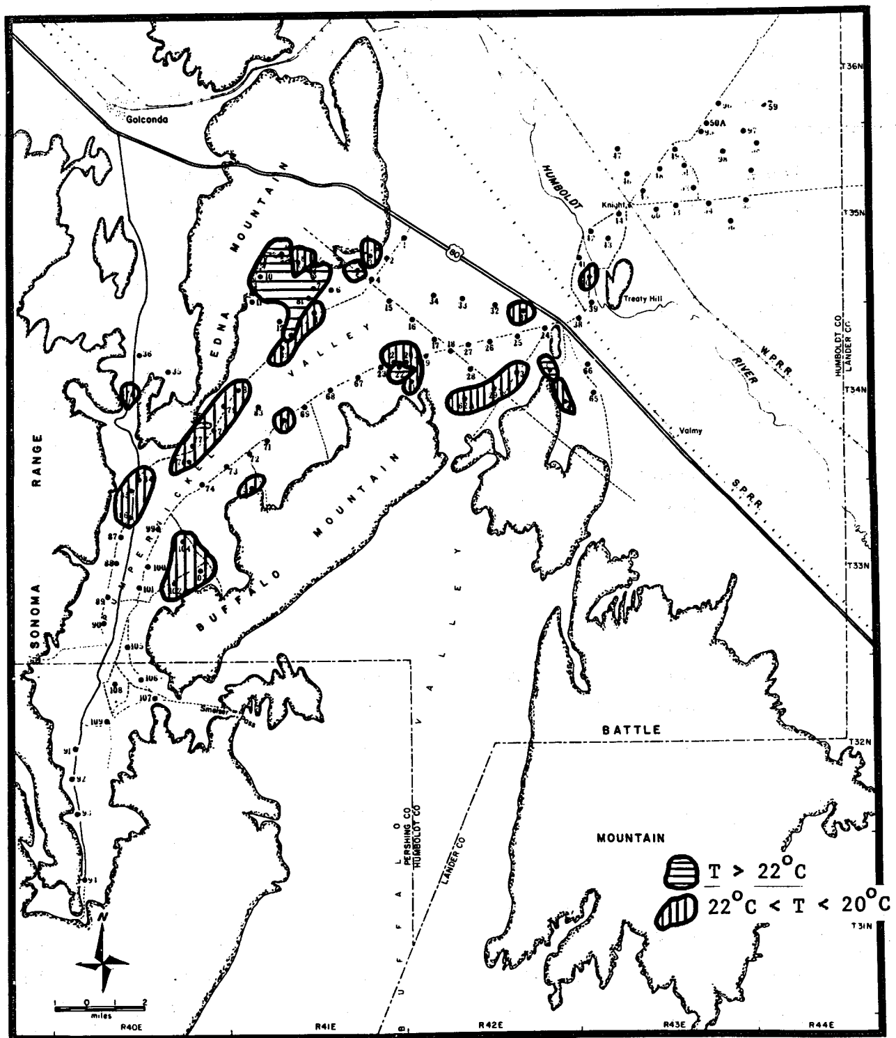
Figure A13. Locations of two-meter temperature probes in Pumpernickel Valley, showing areas of relatively higher temperatures.
