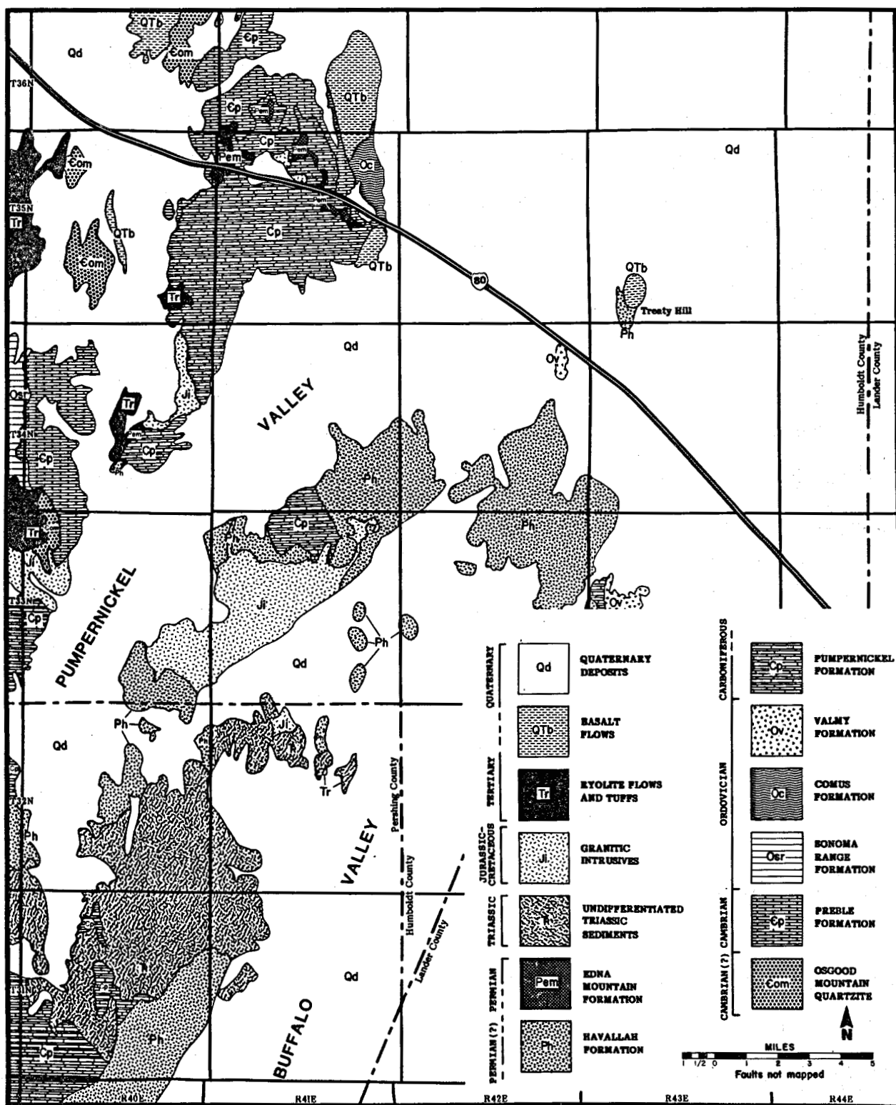
Figure A2. Generalized geologic map of Pumpnickel Valley.
