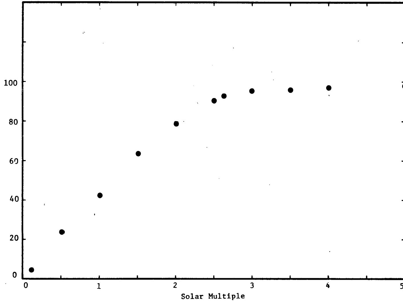
Figure 4. Plant designed for minimum busbar energy cost. Hybrid solutions such as this one will always provide somewhat less energy from the sun, but at potentially large cost benefits. The hybrid's busbar energy cost at a solar multiple of 2.63 is less than half that of the solar plant.
