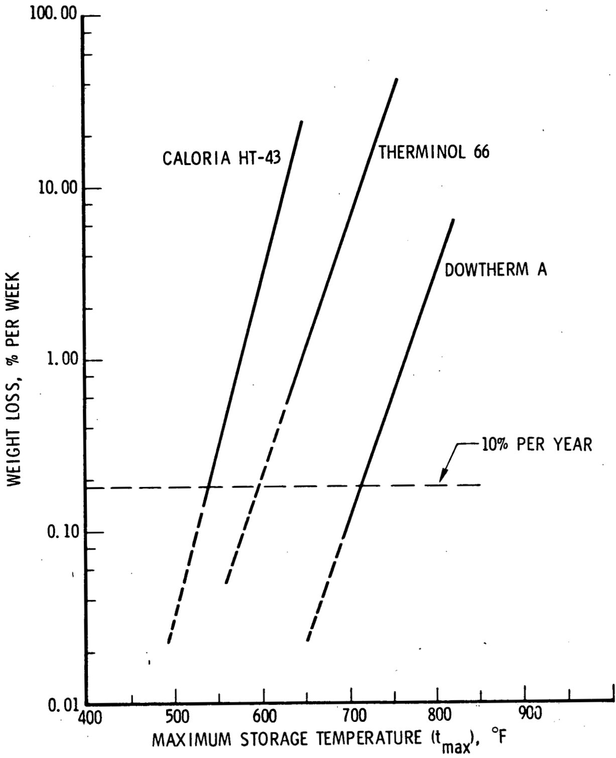
Fig. 2. Comparative Decomposition of Heat Transfer Oils versus Maximum Storage Temperature
