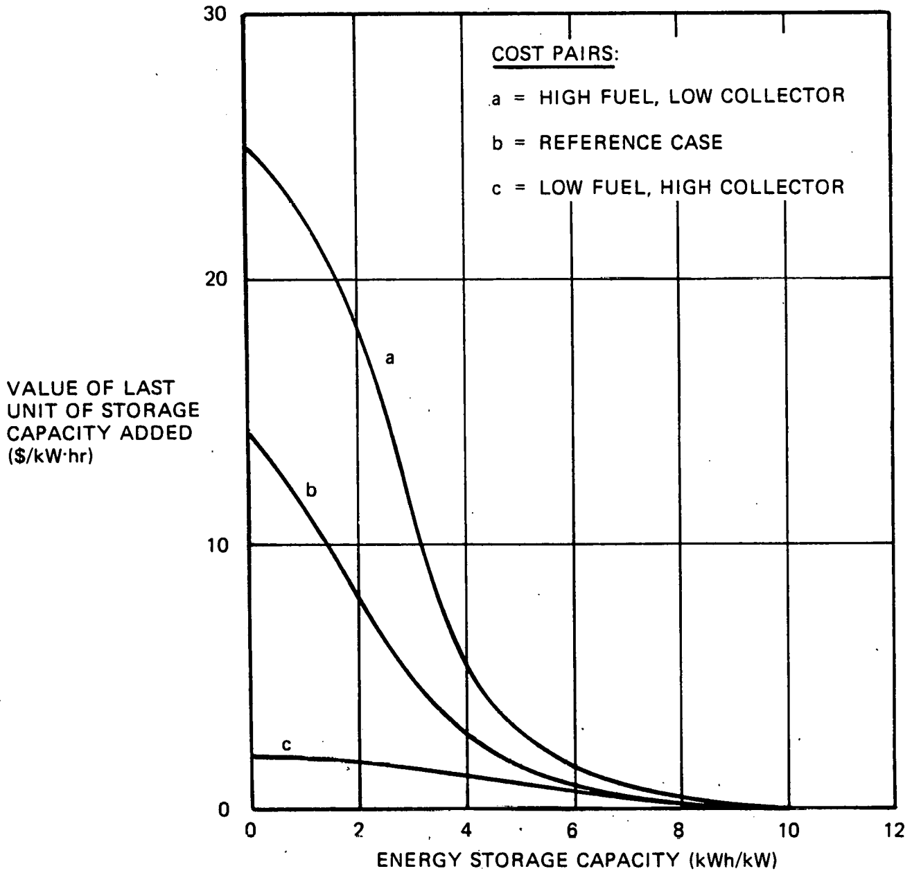
Fig. 9. Value of last unit of energy storage as a function of storage capacity for low-intermediate load power plant (25% demand factor) at Inyokern.
