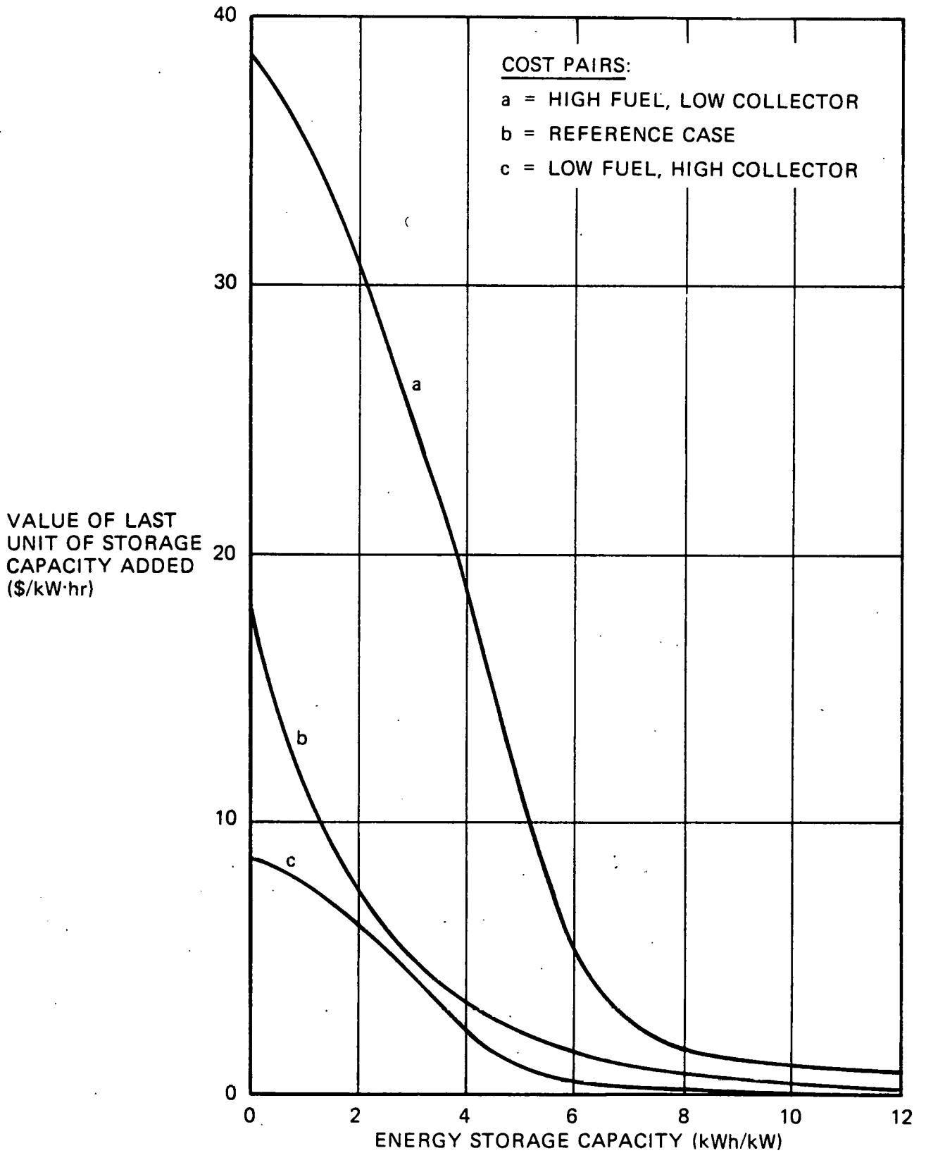
Fig. 8. Value of last unit of energy storage as a function of storage capacity for intermediate load power plant (50% demand factor) at Inyokern.
