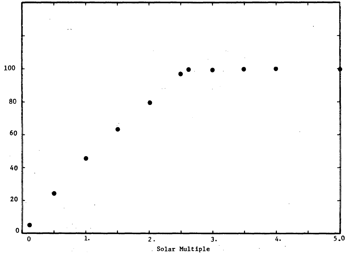
Figure 2. Solar output maximized. Note sub-linear dependence of percent solar on the solar multiple as a larger and larger fraction of the energy comes through storage with its parasitic power losses.
