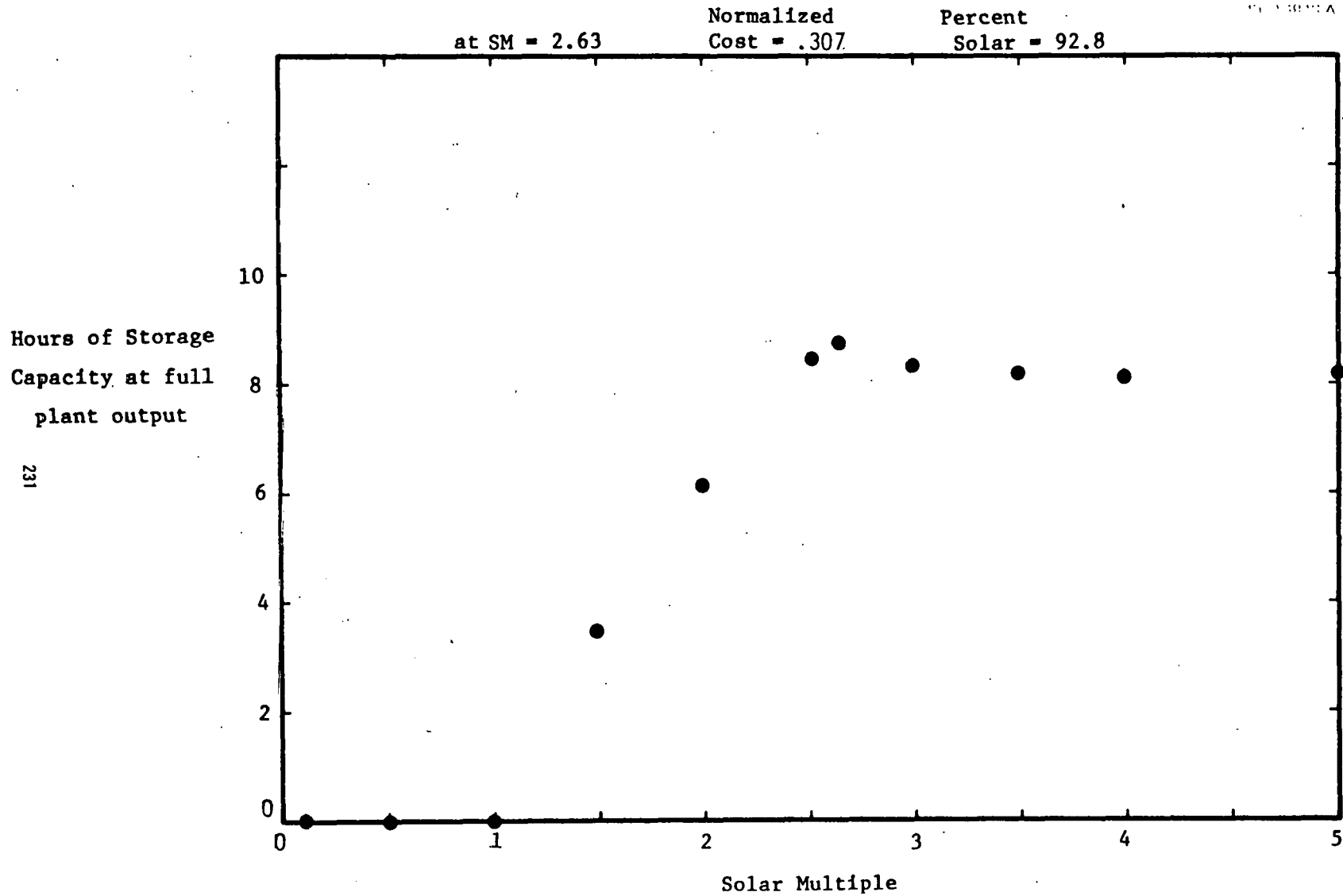
Figure 5. Plant designed for minimum busbar energy cost. While the amount of storage still peaks near the critical solar multiple of 2.63, note the dramatic change in storage requirement for a small amount of hybridization .
