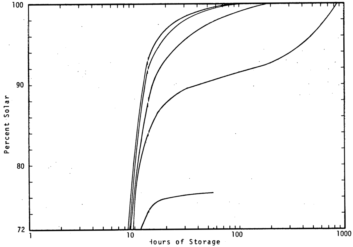
Figure 14. These are the Same Albuquerque Baseload Results as in Figure 13, But On an Expanded Performance Scale
