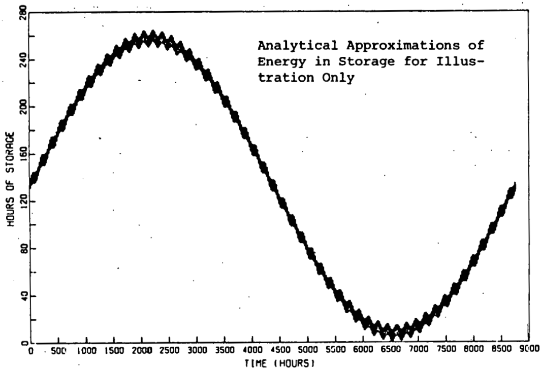
Figure 6. Although sine functions were chosen for simplicity, any periodic function could be used to represent the seasonal amount of energy in storage. The breadth in this curve is due to the lower amplitude, higher frequency components corresponding to daily and weekly variations of the energy in storage. Here we have taken the seasonal component of storage to be 250 hours, weekly 5 hours, and daily 10 hours. This plot covers an entire year (beginning in the summer) while figure 7 and 8 plot the same function for periods of roughly a month and a week.
