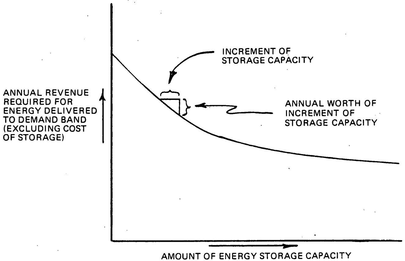
Fig. 4. Method of determining the marginal worth of energy storage.
