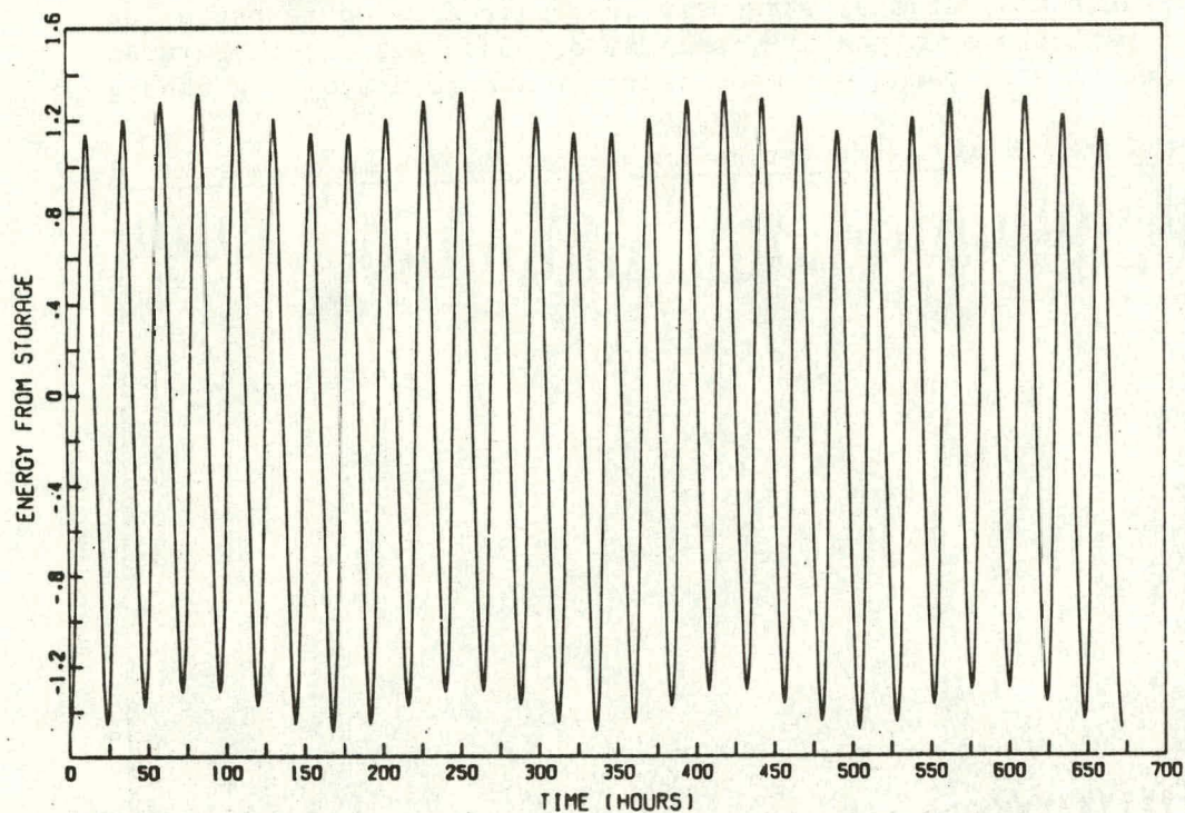
Figure 10. This is the energy from storage during the first month (July) only. Slight weekly variations are visible, but no seasonal component is obvious.
