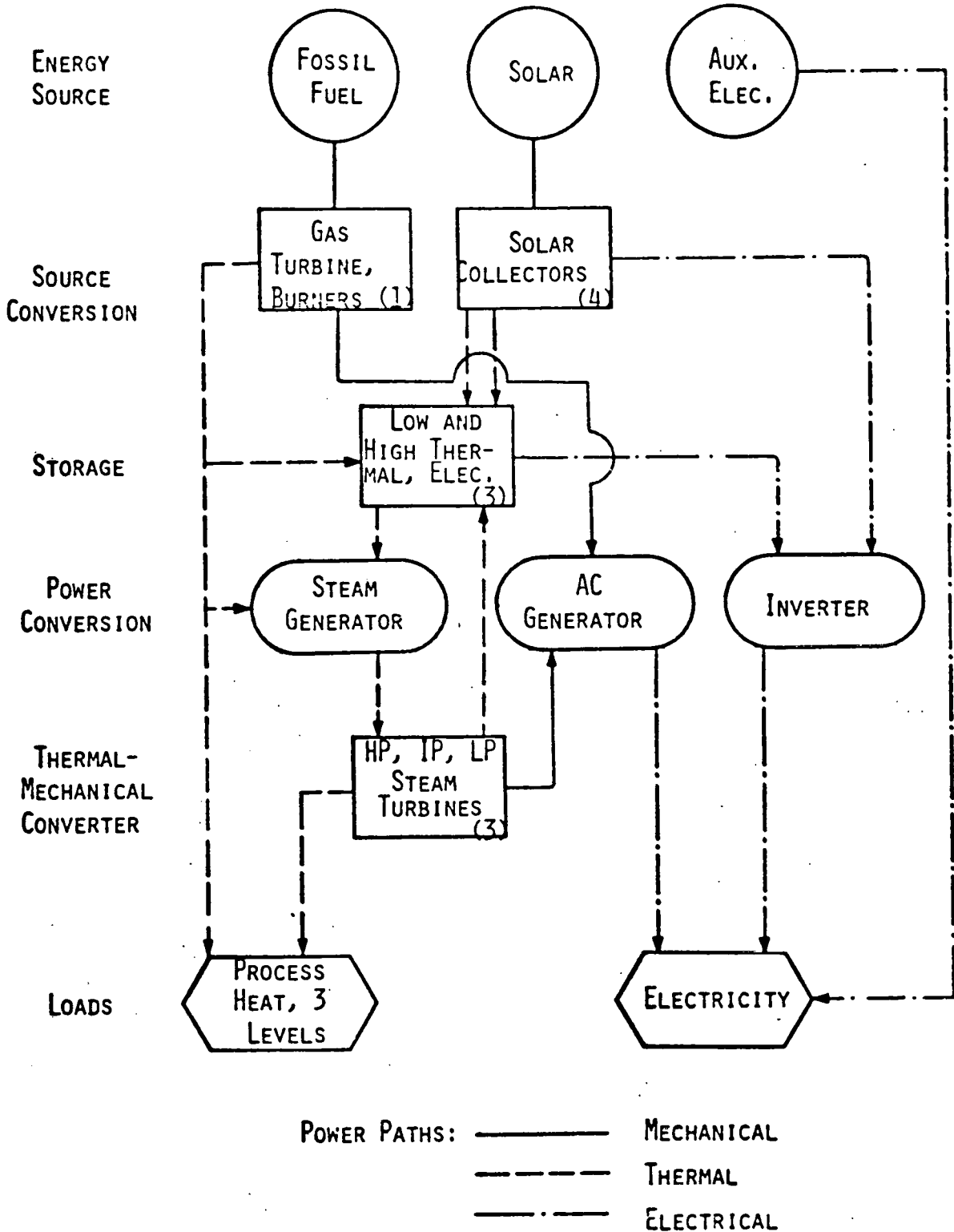
FIGURE 6. SOLAR TOTAL-ENERGY POWER FLOW LOGIC
