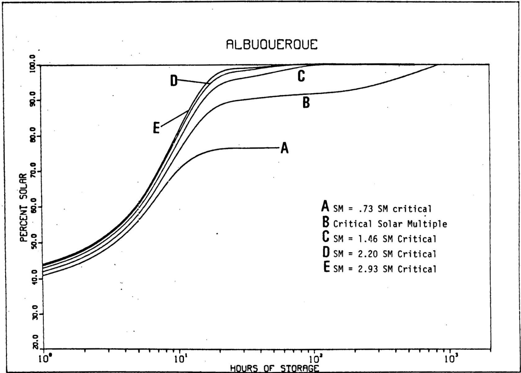
Figure 13. Percent Solar of a Constant Load versus Hours of Storage Over Three Orders of Magnitude
