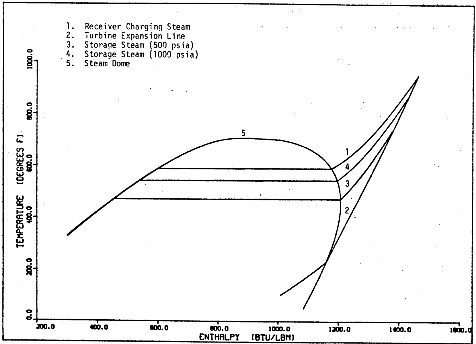
Figure 1. T-H Diagram
