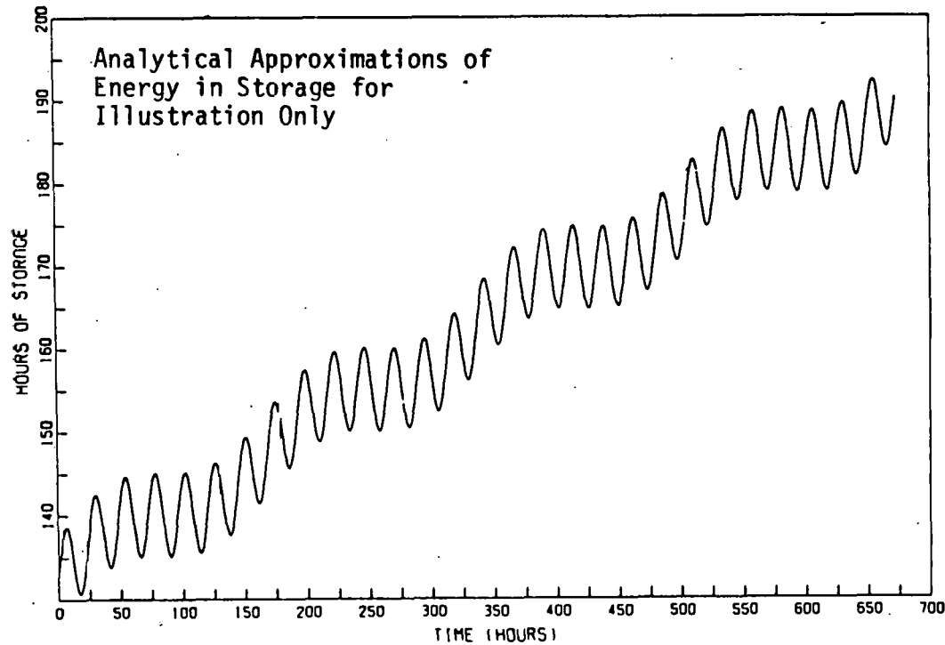
Figure 7. This is again the idealized energy in storage for a plant which stores "seasonally", but covering only the first month of this year (perhaps July). This was a favorable solar month since there is more energy in storage at the end of the month than at the beginning, despite the daily and weekly oscillations. The four weekly cycles are now clearly visible. These might be due to weekend load reductions.
