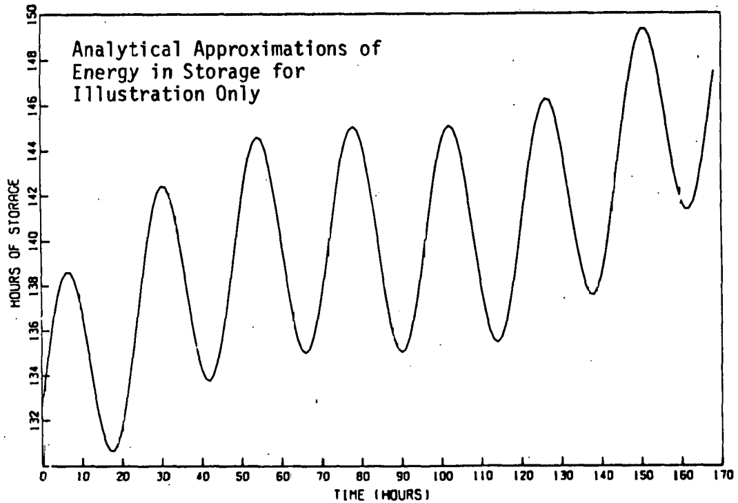
Figure 8. Once again the energy in storage but for now for the first week in July. The seasonal trend is discernable on this scale and the weekly variation is clearly seen. The main feature is the daily variation of energy in storage to provide the nightly loads.
