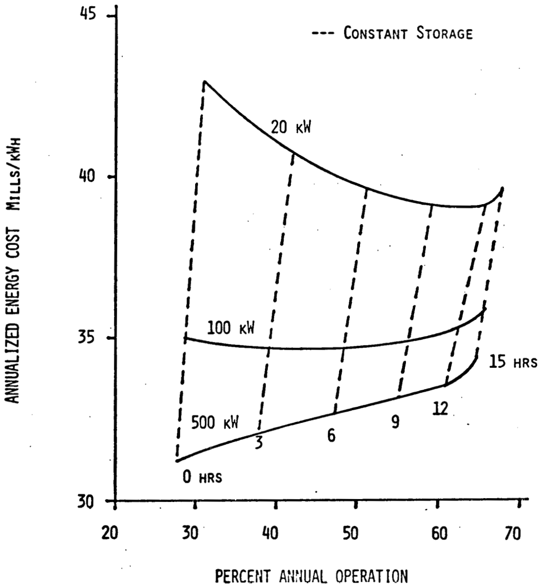
FIGURE 2. SOLAR IRRIGATION ENERGY COSTS AND LOAD FACTORS
