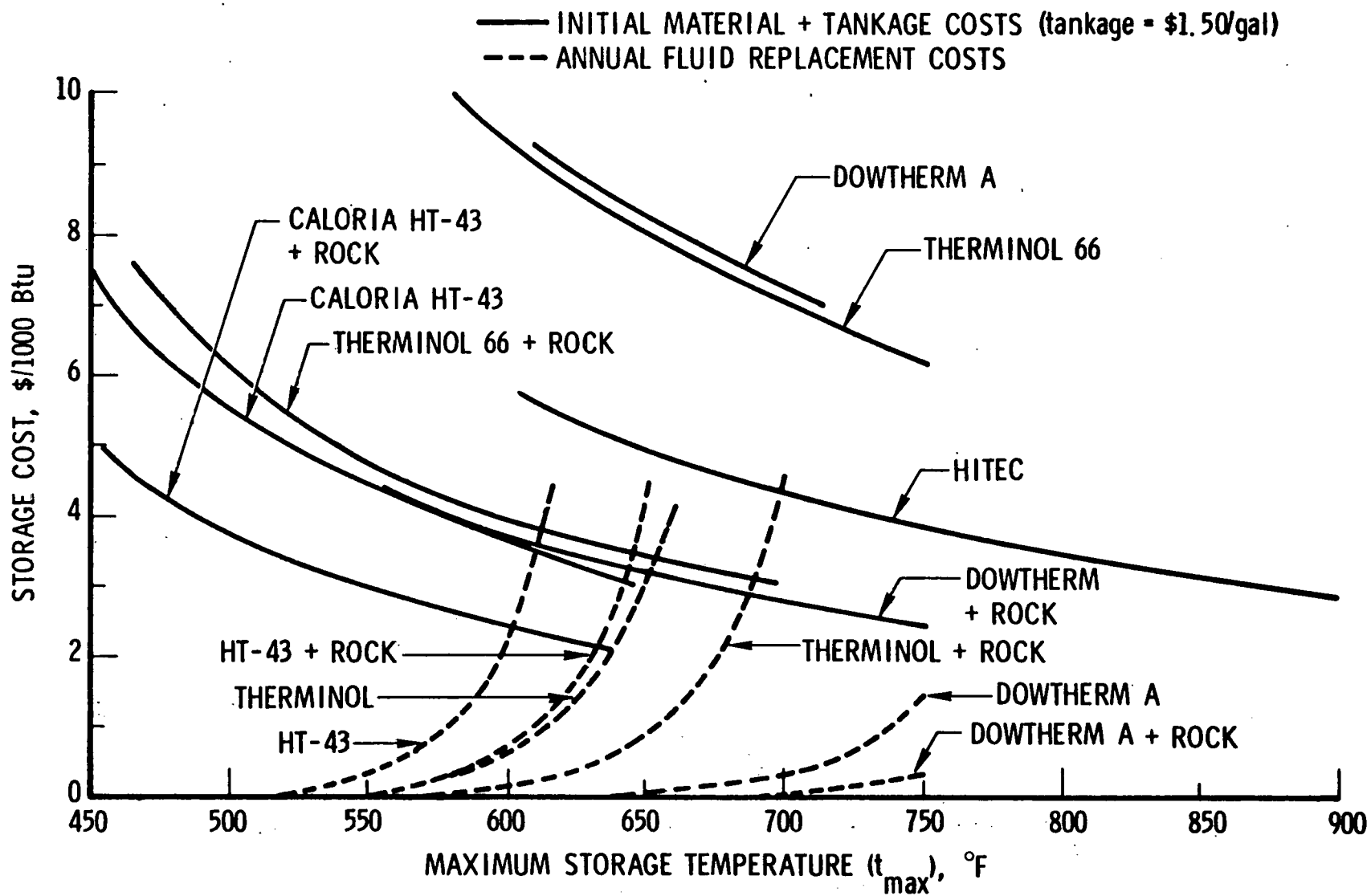
Fig. 9. High Temperature Thermal Storage Costs versus Maximum Storage Temperature
