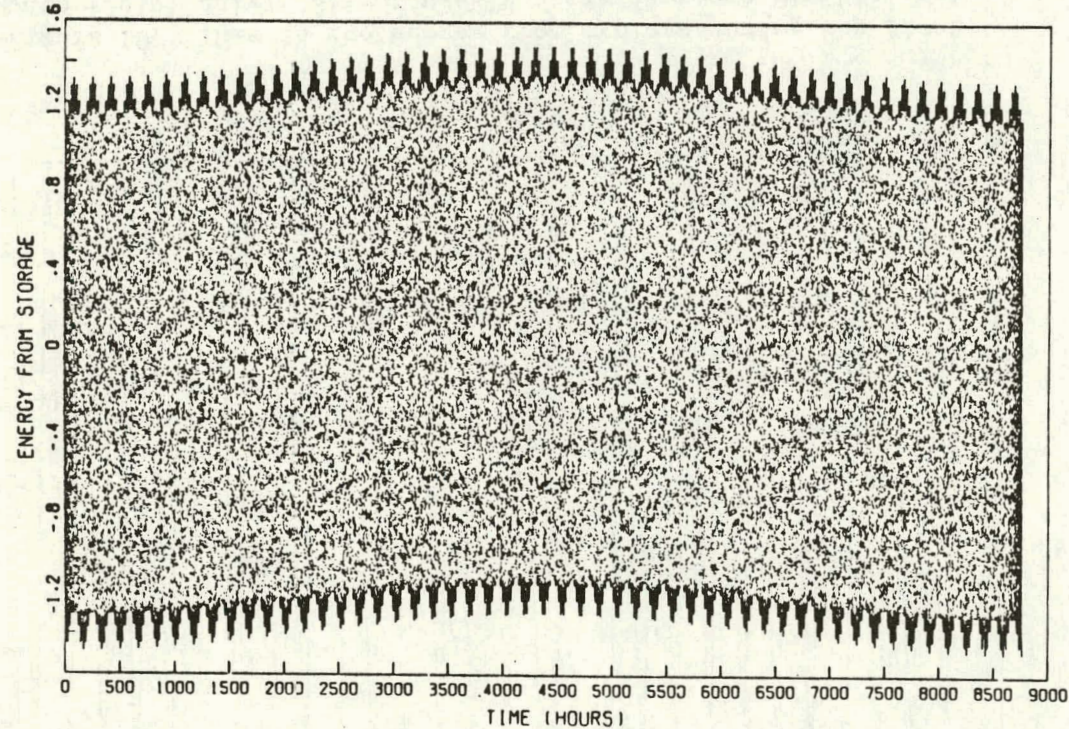
Figure 9. This plot may at first seem too broad to have any meaning, quite the opposite is true. It would be expected to be broad since many different discharge (energy from storage >0 ) and charge (energy from storage <0 ) rates are used during a year (or in fact during any one day). The most interesting feature is that the energy from storage does not peak significantly in the winter as one might expect, this is since the derivative is everywhere dominated by the highest frequency term, the daily variations.
