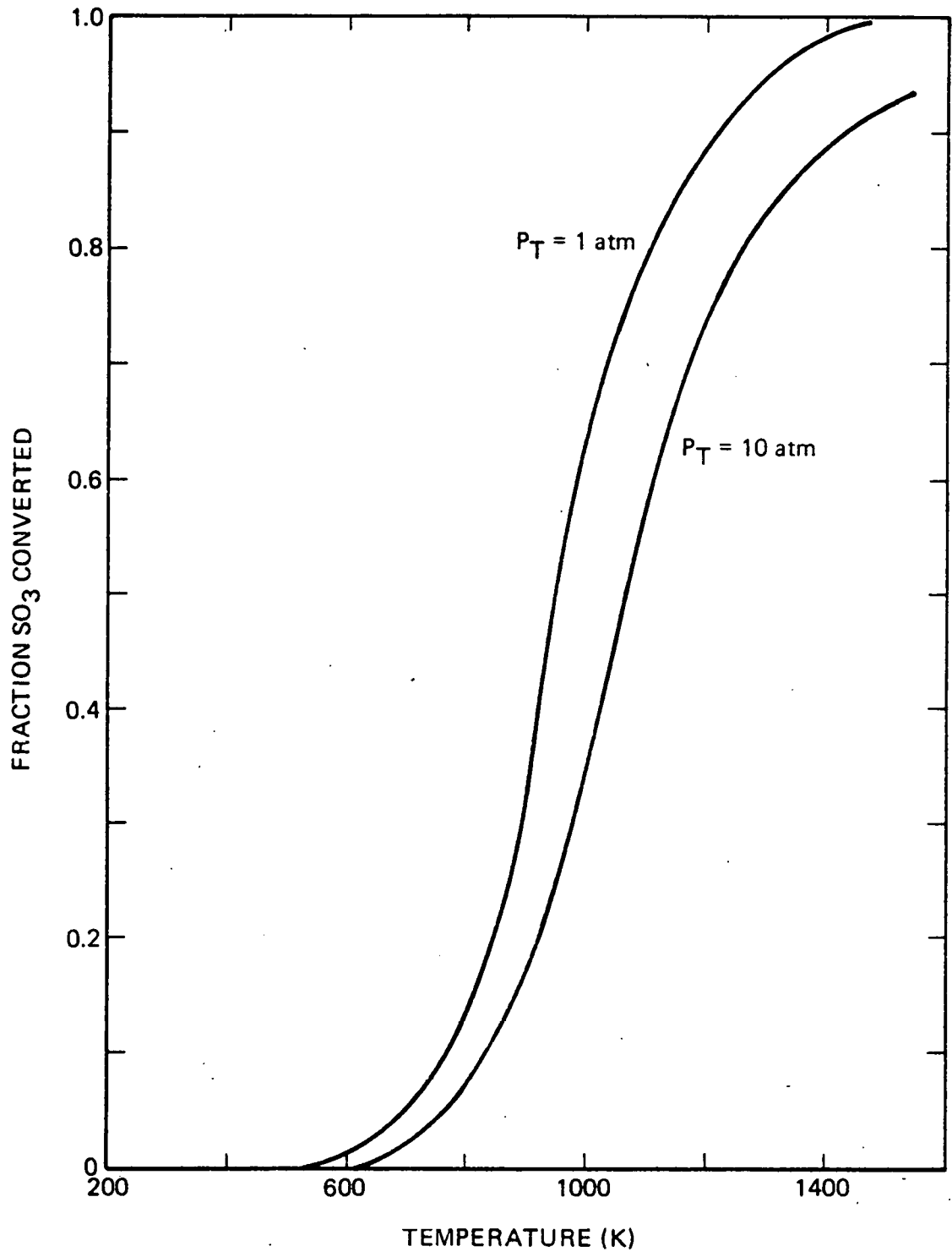
Figure 3. Equilibrium conversion of SO 3 .
