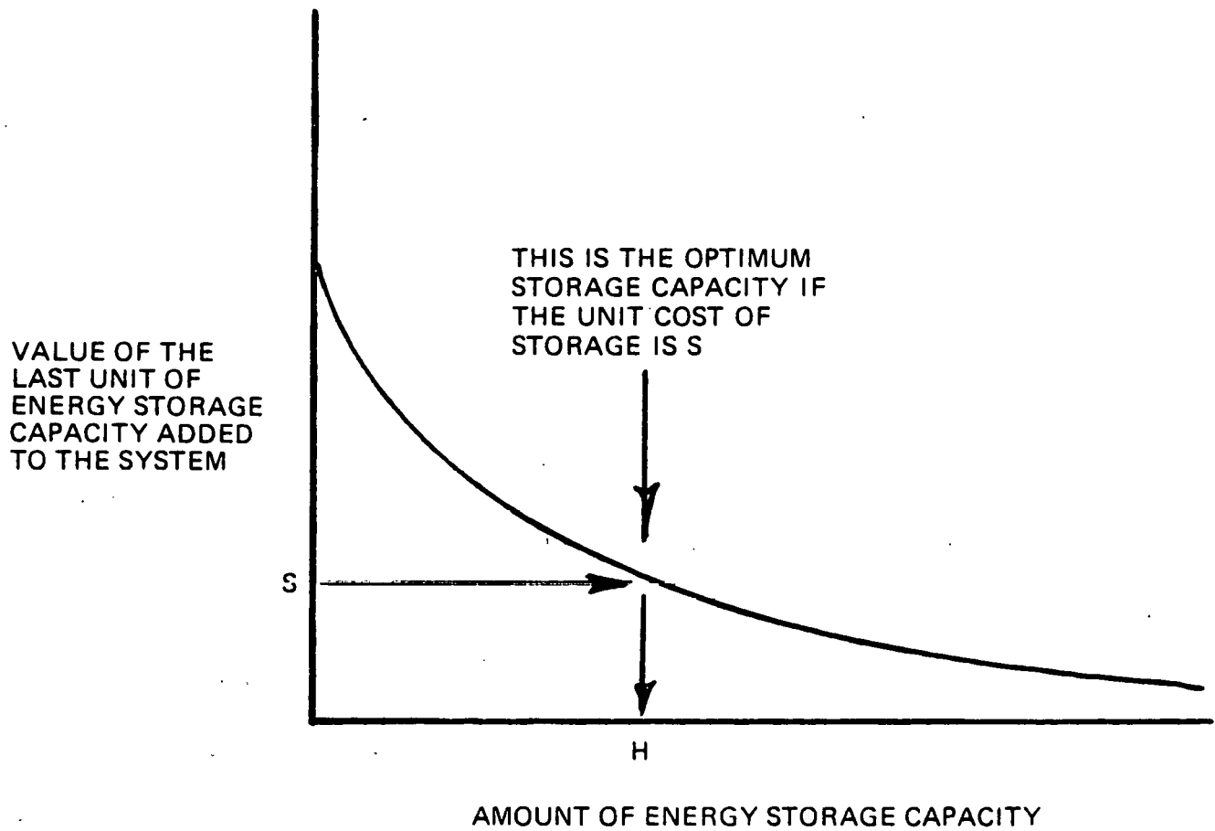
Fig. 5. General characteristics of the marginal worth of storage as a function of storage capacity.
