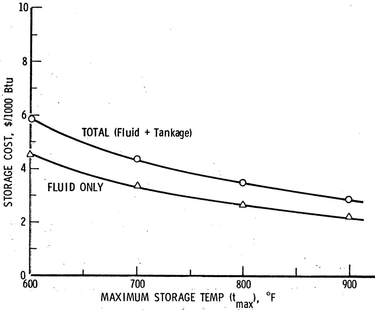
Fig. 7. Storage Cost of HITEC versus t_{max}
