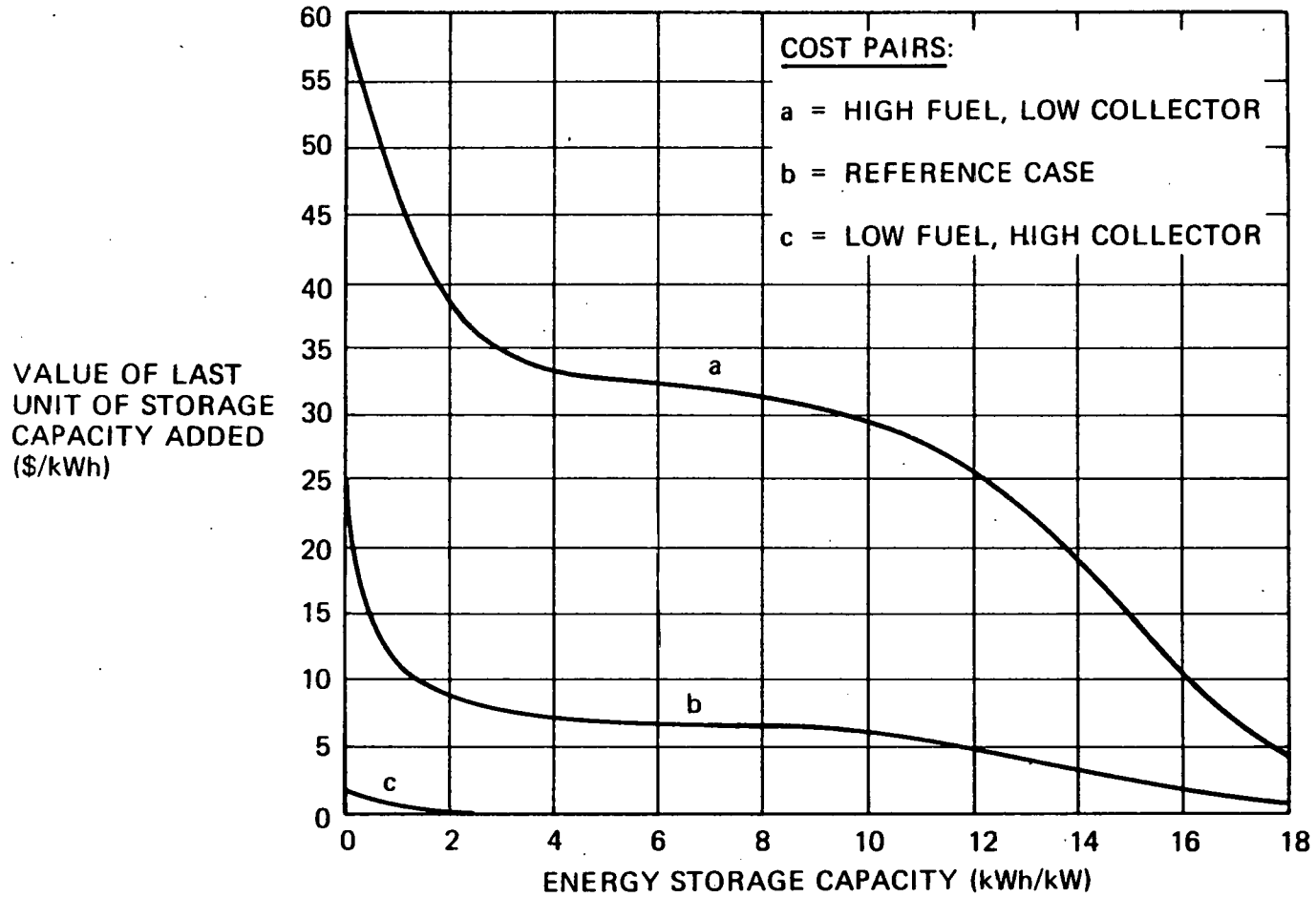
Fig. 7. Value of last unit of energy storage as a function of storage capacity for base load power plant (100% demand factor) at Inyokern.
