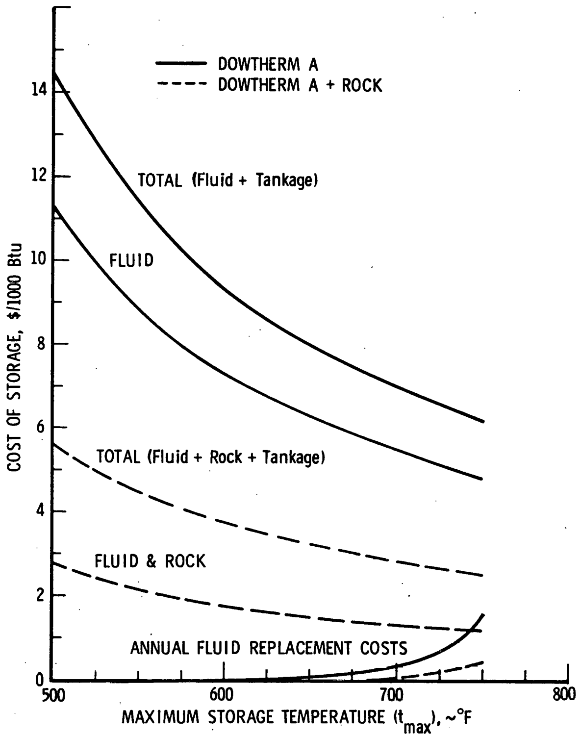
Fig. 6. Storage Cost of Dowtherm A versus t_{max}
