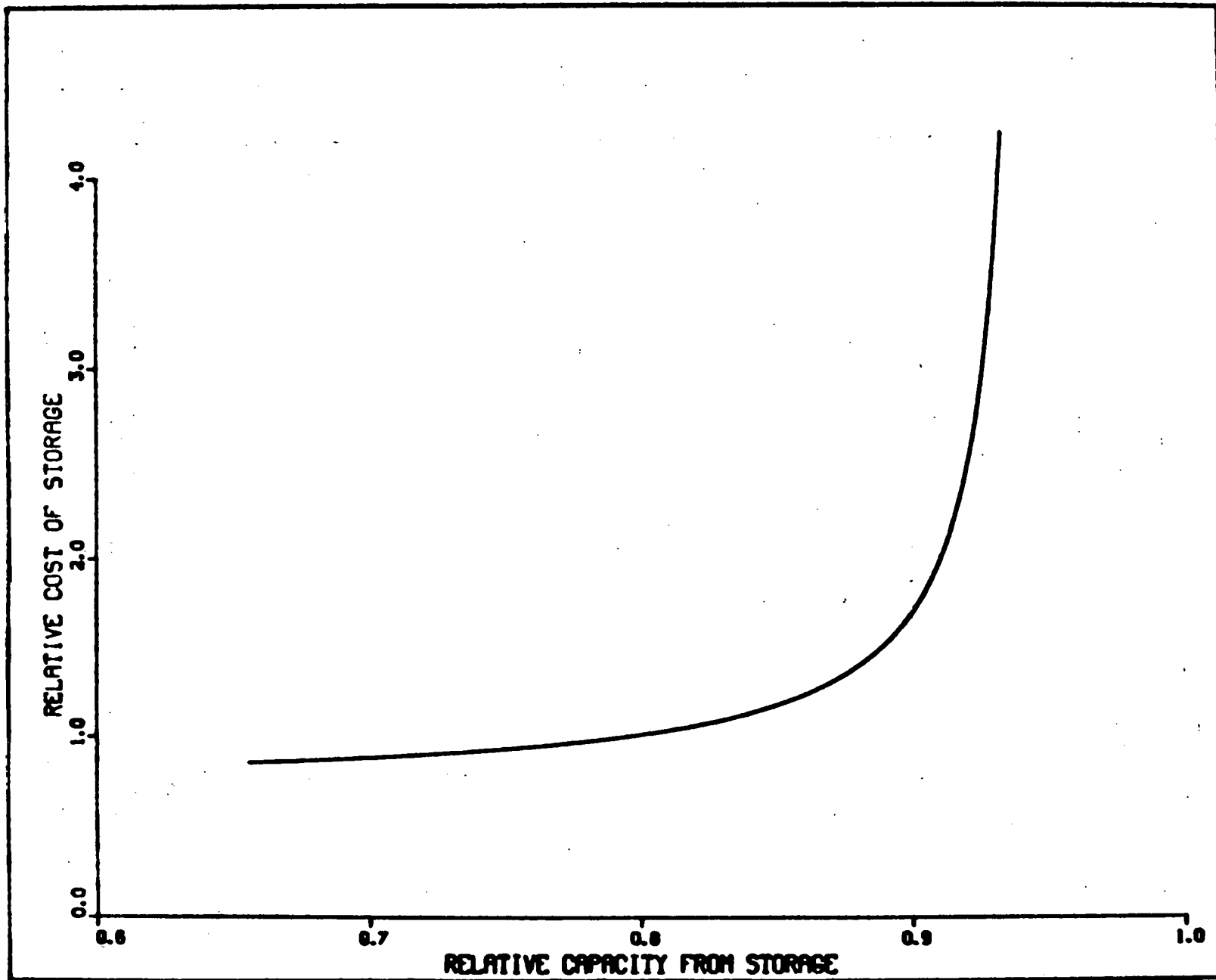
Figure 2. Relative Cost vs. Relative Capacity
