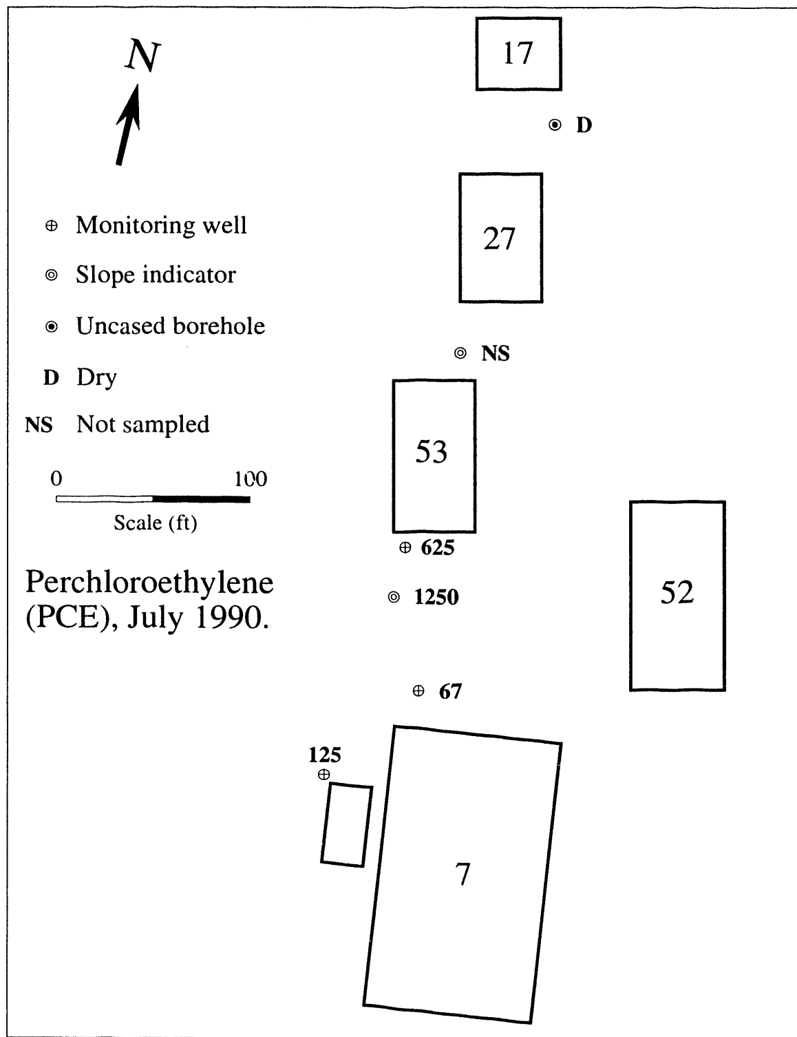
Figure 24. Perchloroethylene (PCE) concentration in ppb, measured in water samples from wells and slope indicators in July 1990.
