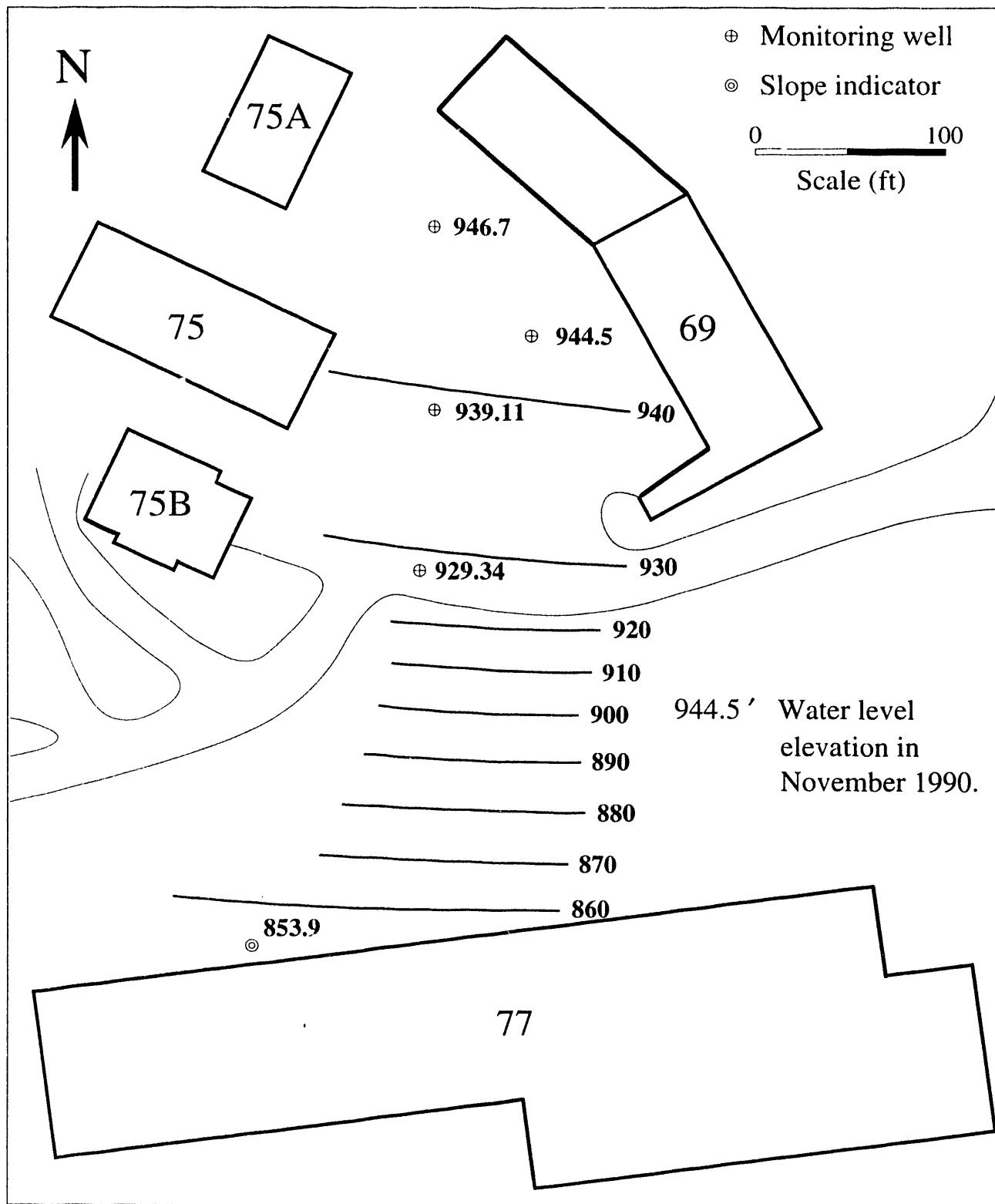
Figure 26. Piezometric map of groundwater in November 1990.
