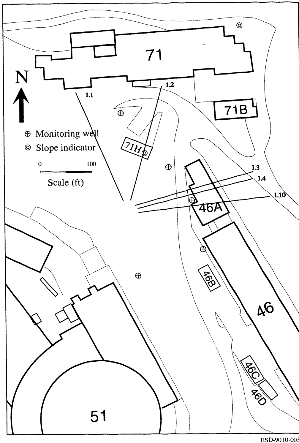
Figure 19. Approximate position of Hydraulics 1.1, 1.2, 1.3, 1.4 and 1.10 of 51 series.
