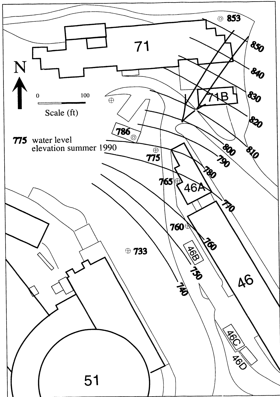
Figure 22. Piezometric map of groundwater in the vicinity of Bldgs. 46, 51 and 71, during the summer of 1990.
