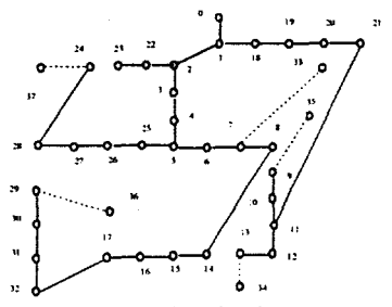
(f) 113% load level (initial configuration 2)
