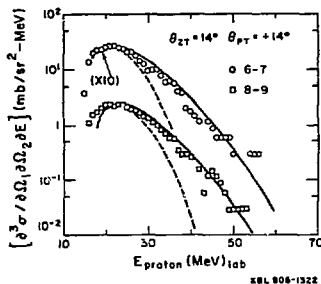
Fig. 8. Proton spectra in coincidence with deep inelastic processes for the reaction 252 \text{ MeV } ^{20}\text{Ne} + \text{natCu} . The dashed lines are evaporation calculations without fluctuations in the energy partition. The solid lines incorporate the fluctuations.
