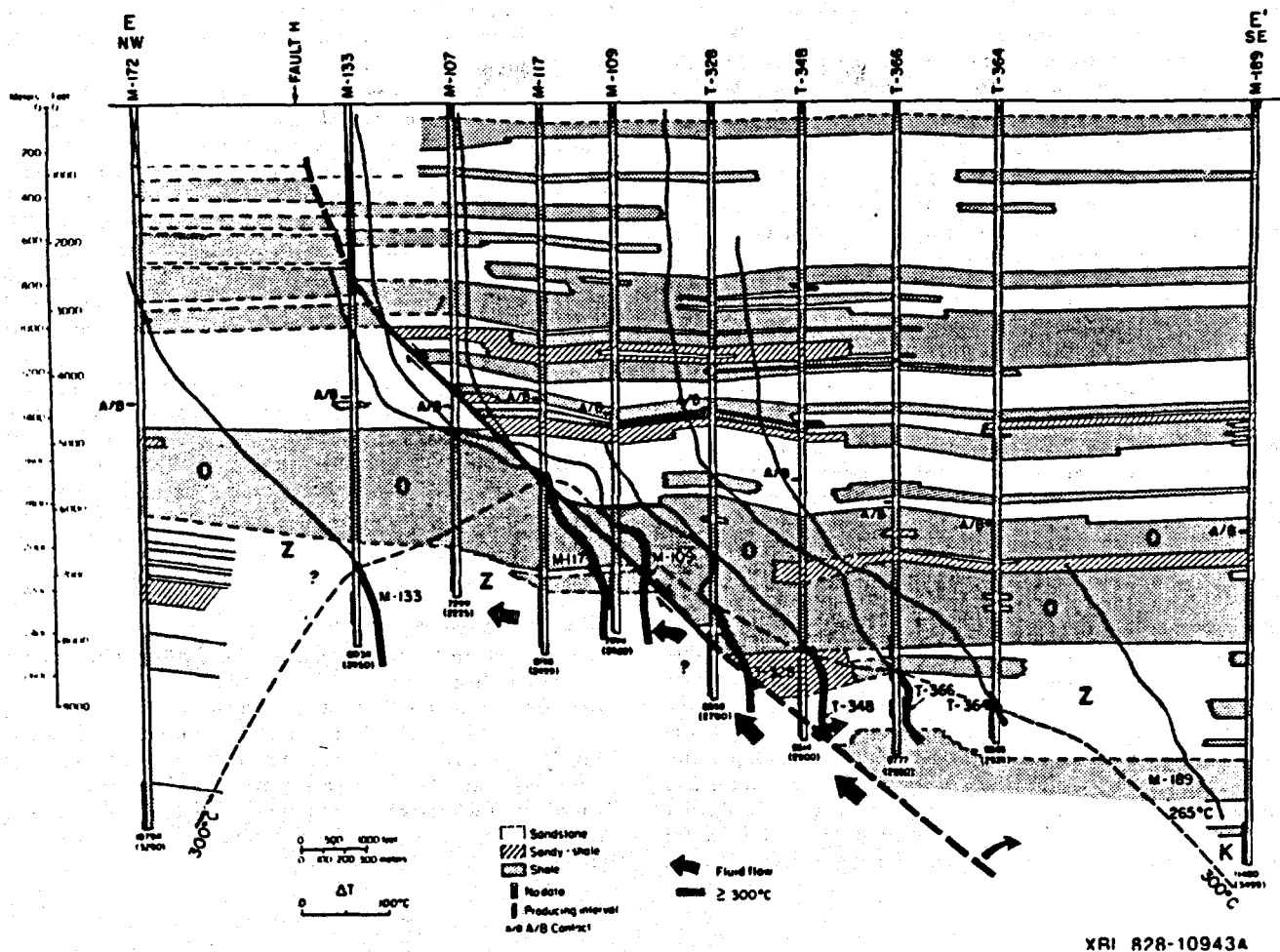
Figure 6. Lithofacies cross section E-E' showing the updated geothermal fluid flow pattern.
