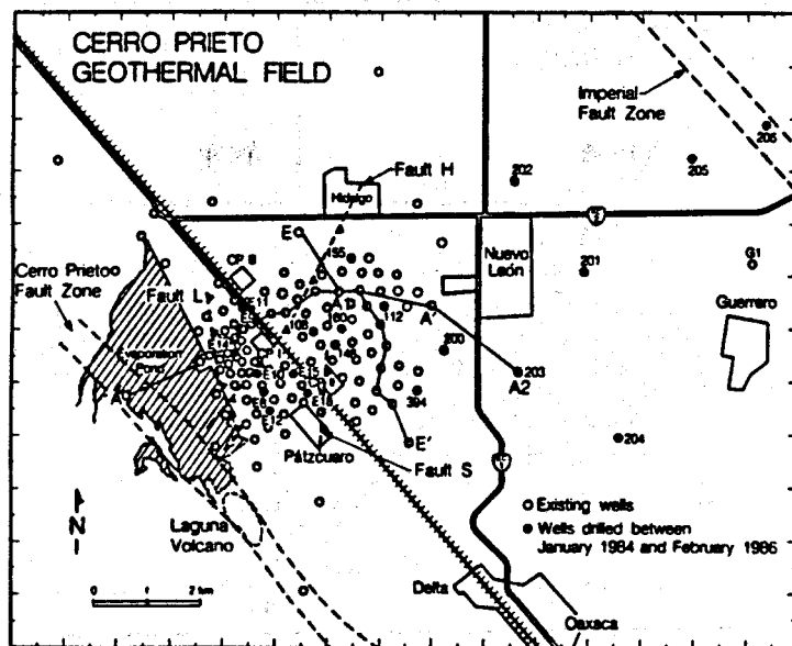
Figure 2. Location of old and new wells, principal faults, and cross sections A-A', A1-A2, and E-E'. The faults are projected to the surface.
