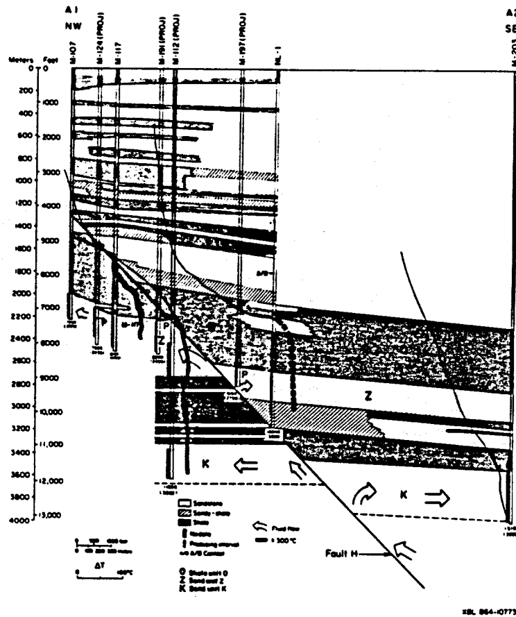
Figure 5. Lithofacies cross section A1-A2 showing the updated geothermal fluid flow pattern.
