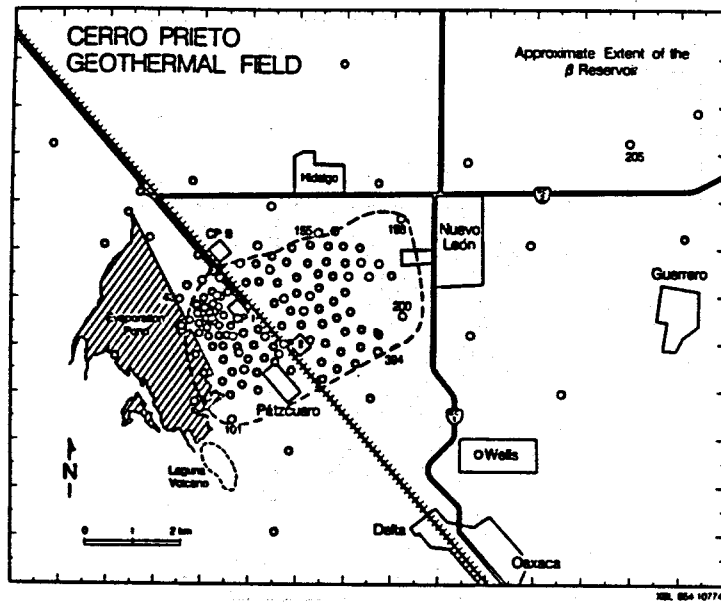
Figure 4. Approximate extent of the hot \beta geothermal reservoir as inferred from well data.
