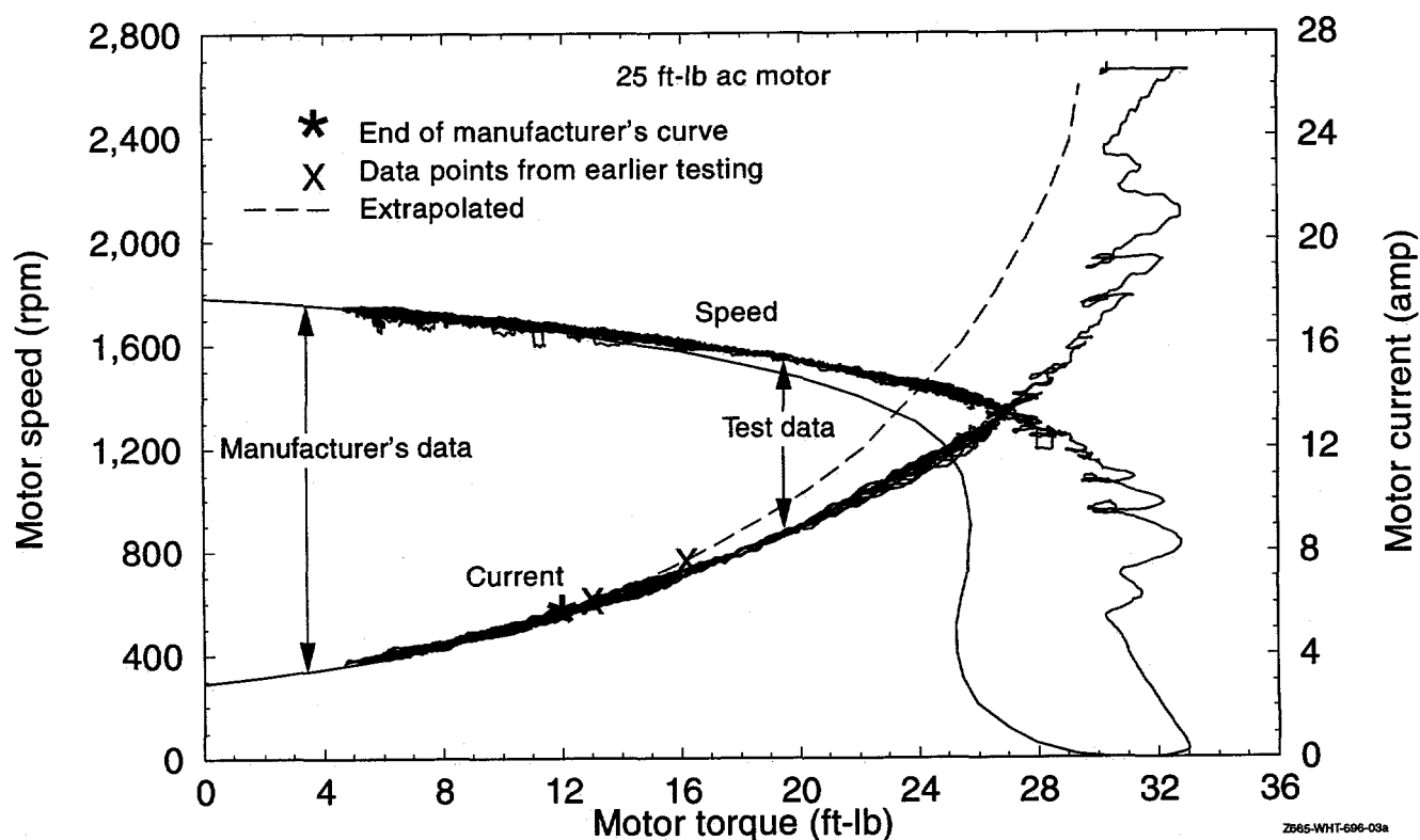
Figure 6. Motor performance curves derived from testing of the 25 ft-lb ac motor; manufacturer's published data are also shown.
