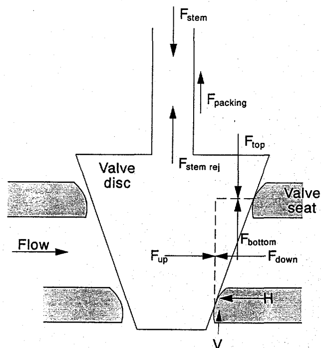
Figure 2. Sketch of the internal components of a gate valve, showing the main forces involved in a valve closure.
