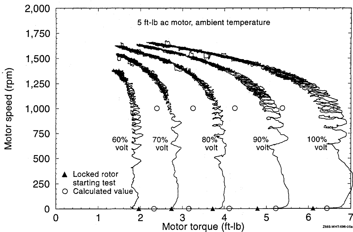
Figure 9. Motor speed versus torque, derived from testing of the 5 ft-lb motor at degraded voltage.
