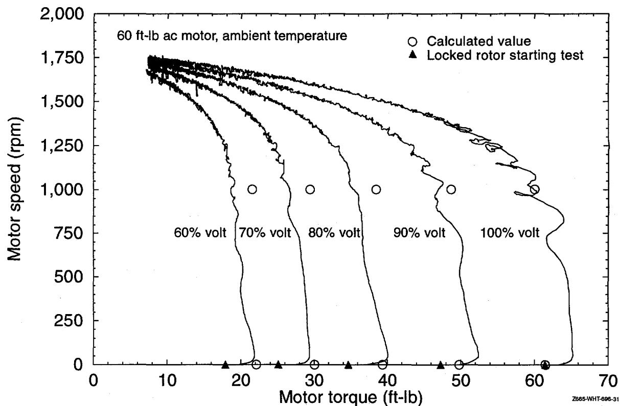
Figure 11. Motor speed versus torque, derived from testing of the 60 ft-lb motor at degraded voltage.
