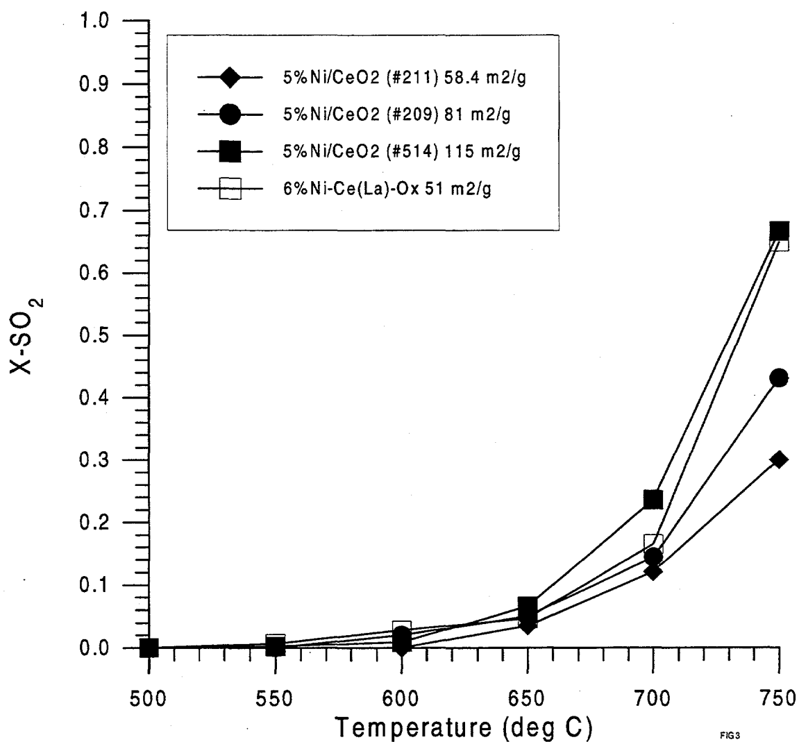
Figure 4-2: Effect of La dopant on the activity of Ni/CeO 2 (1% SO 2 , 0.5% CH 4 balance He, pre-reduced in 9.9% CO/He at 500°C for 1 hr, contact time = 0.18 gs/cc).
