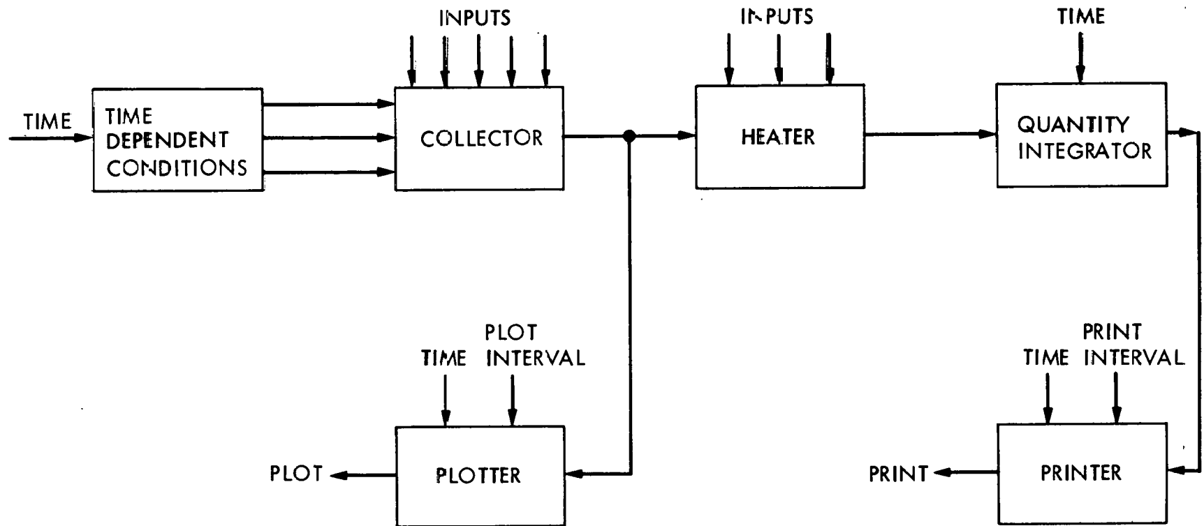
Figure 4-10. Sample Transient Simulation Program (ASJ Version) Structure (Source: Evans, et al., 1978)
