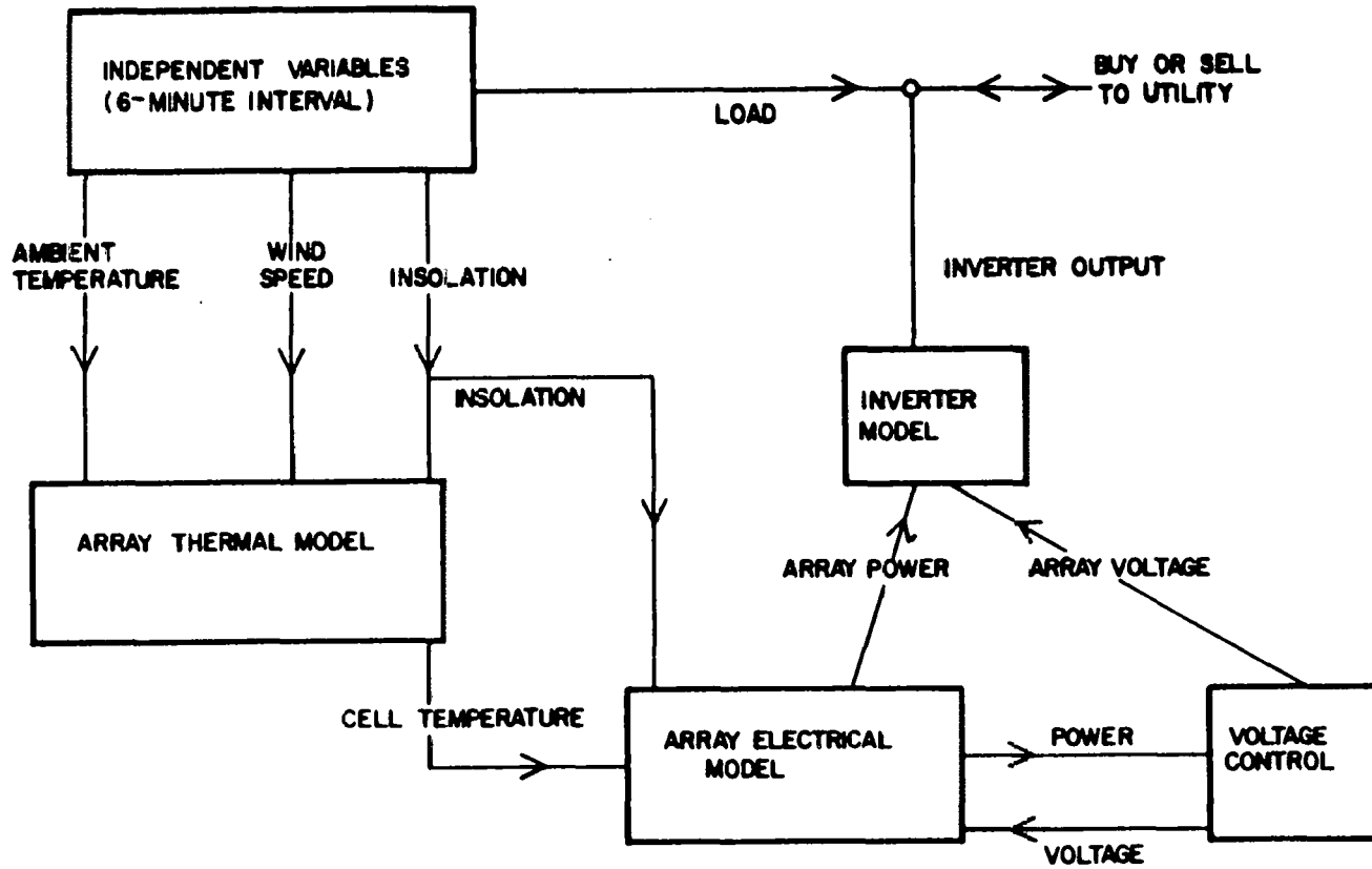
Figure 4-11. Transient Simulation Program (MIT Version) Framework (Source: Hart and Raghuraman, 1982b)
