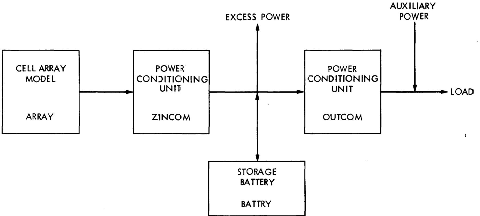
Figure 4-9. Solar Energy Systems Analysis Model Structure (Source: Edenburn, 1980)
