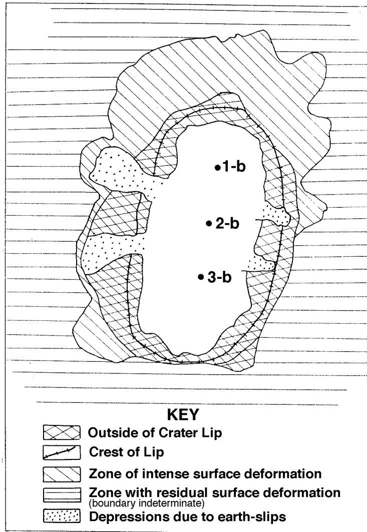
Figure 3. Sketch map of the “Taiga” Crater along the proposed alignment of the Kama-Pechora Canal showing the outline of the crater and areas where there was failure of the crater slopes (from Ref. 34).
