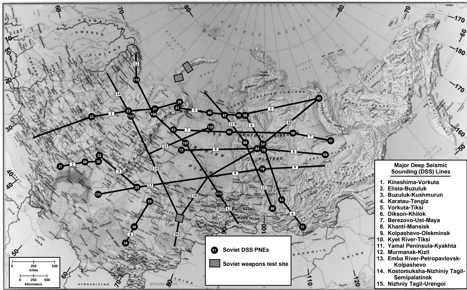
Figure 6. Map of Soviet Union showing the Deep Seismic Sounding (DSS) explosions and the DSS lines connecting them along which seismometers were placed every 10–20 km to record the seismic signals to learn about the structure of the crust and upper mantle.
