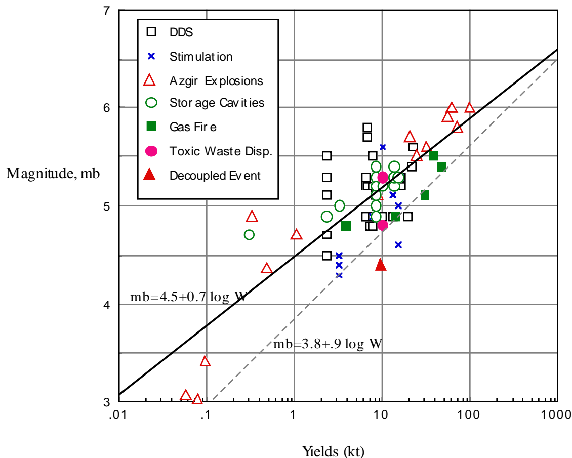
Figure 9. Plot of seismic magnitudes vs yield for 102 contained Soviet PNEs. (Many data points do not appear on the plot because they have the same coordinates and are on top of one another.) The various symbols indicate the purpose of the PNEs. Also shown is a regression fit to the PNE data (solid line) and, for comparison purposes, a fit often associated in the past with estimates of the yields of Soviet weapons tests and PNEs (dashed line).
