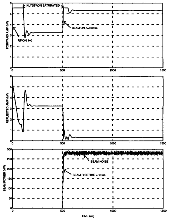
Figure 3. Normal RF and beam turn-on. Forward signal out of klystron, cavity reflected signal, beam power in the cavity.
