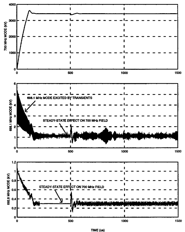
Figure 4. Normal RF and beam turn-on: cavity modes excited.
