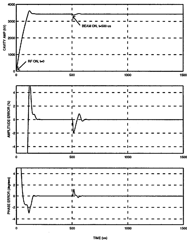
Figure 2. Normal RF and beam turn-on. Cavity field, amplitude and phase errors.
