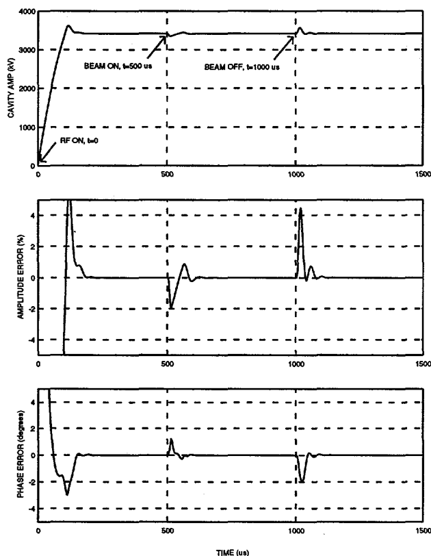
Figure 5. Beam turn-off effect on cavity field, error signals.
