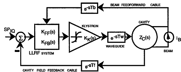
Figure 1. LLRF control system model block diagram.
