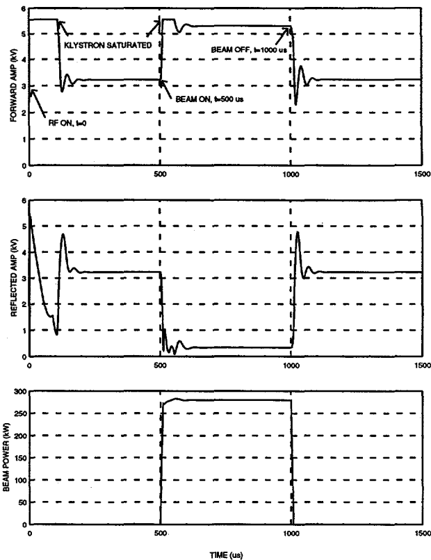
Figure 6. Beam turn-off effect on forward signal out of klystron, cavity reflected signal. Beam power shown.
