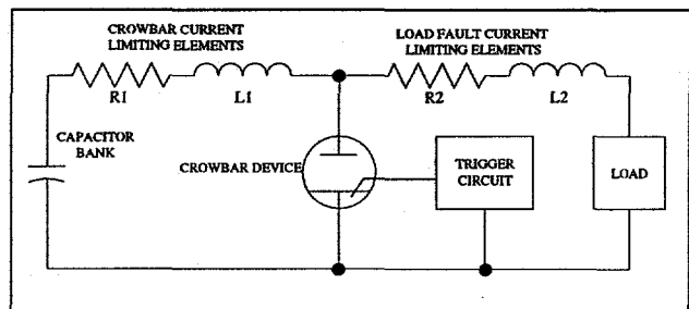
Figure 1: Simplified diagram of a typical crowbar circuit.
