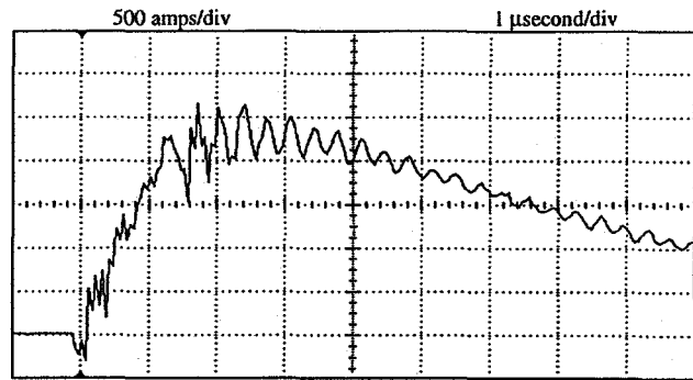
Figure 4: Current through the fault test wire.
