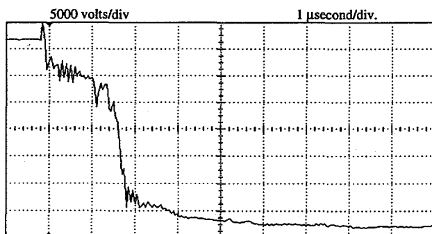
Figure 3: Ignitron voltage during fault.
