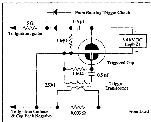
Figure 2: Simplified diagram of the High Speed Crowbar Trigger Circuit.
