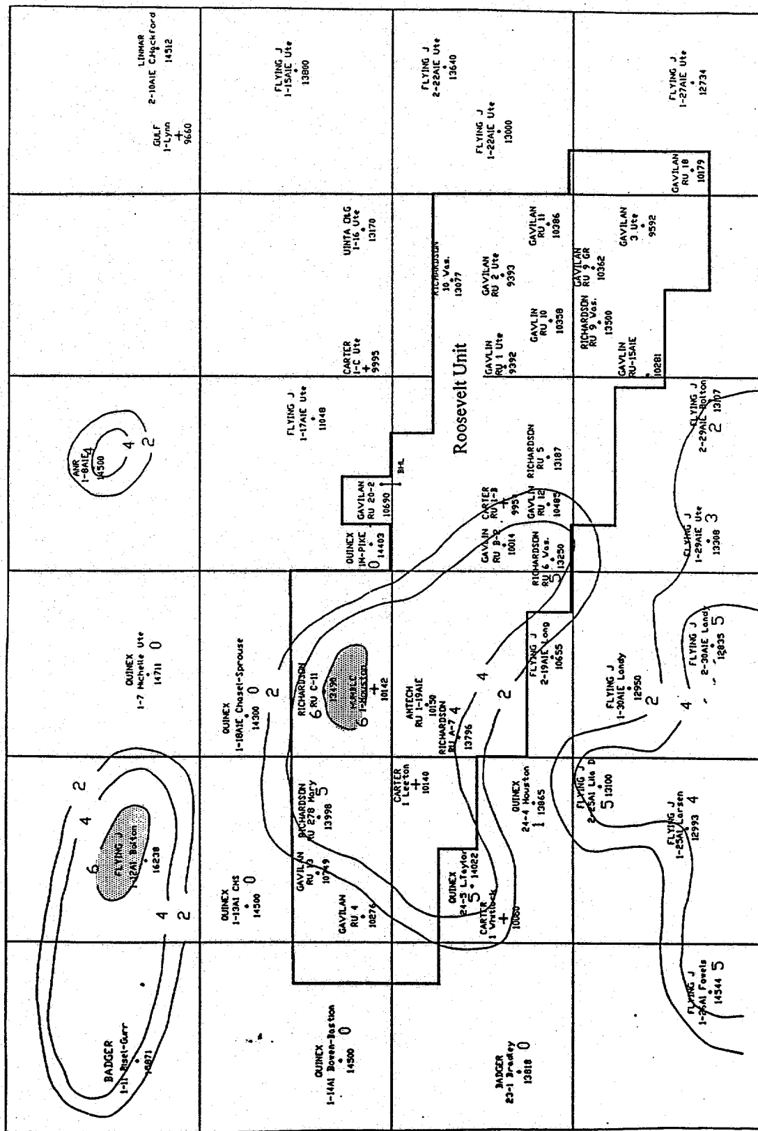
Isopach Map Bed 25a Eastern Bluebell Field Uintah County, Utah
