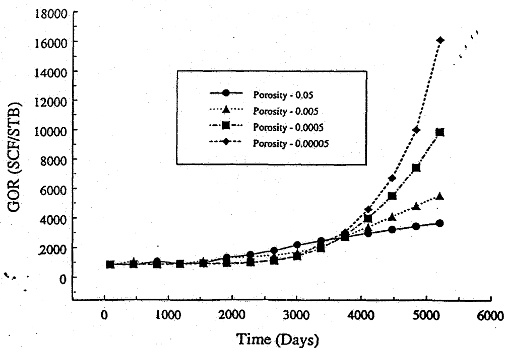
Figure 4.14. Effect of fracture porosity on GORs for Michelle Ute well.
