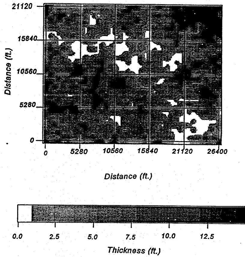
Figure 3.2. Thickness distribution of bed 18 in the 20-square-mile (51.8-km 2 ) area.
