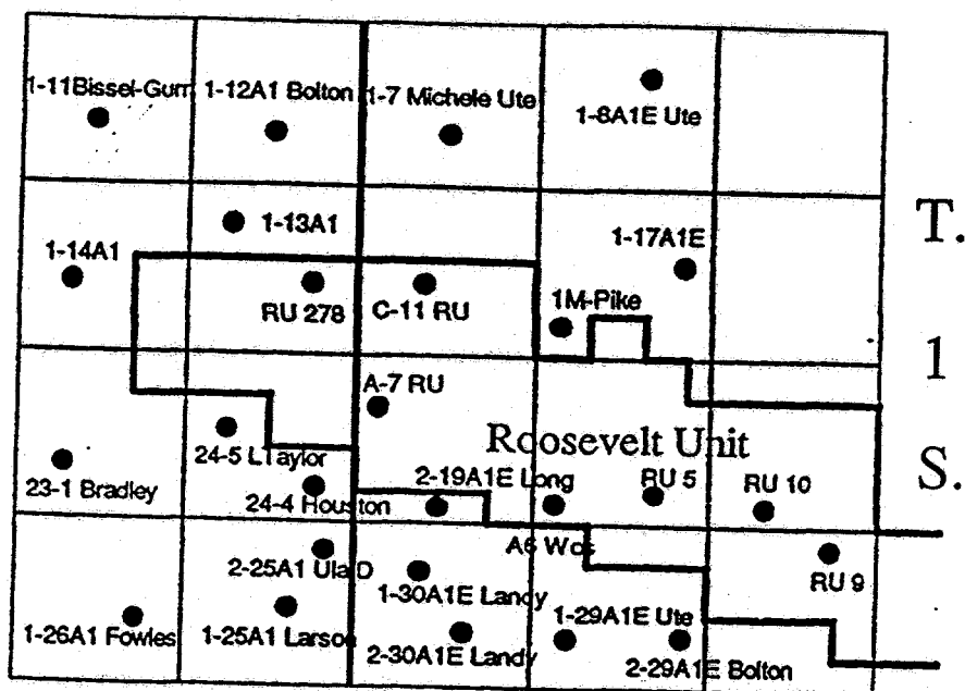
Figure 3.1. Map of the 20-square-mile (51.8-km 2 ) area showing well locations and names.
