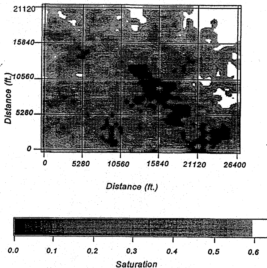
Figure 3.4. Water-saturation distribution of bed 18 in the 20-square-mile (51.8-km 2 ) area.
