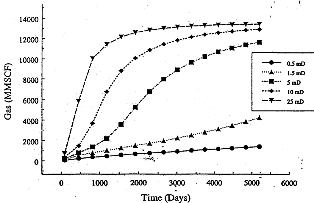
Figure 4.6. Effect of fracture permeability on cumulative gas production in the
