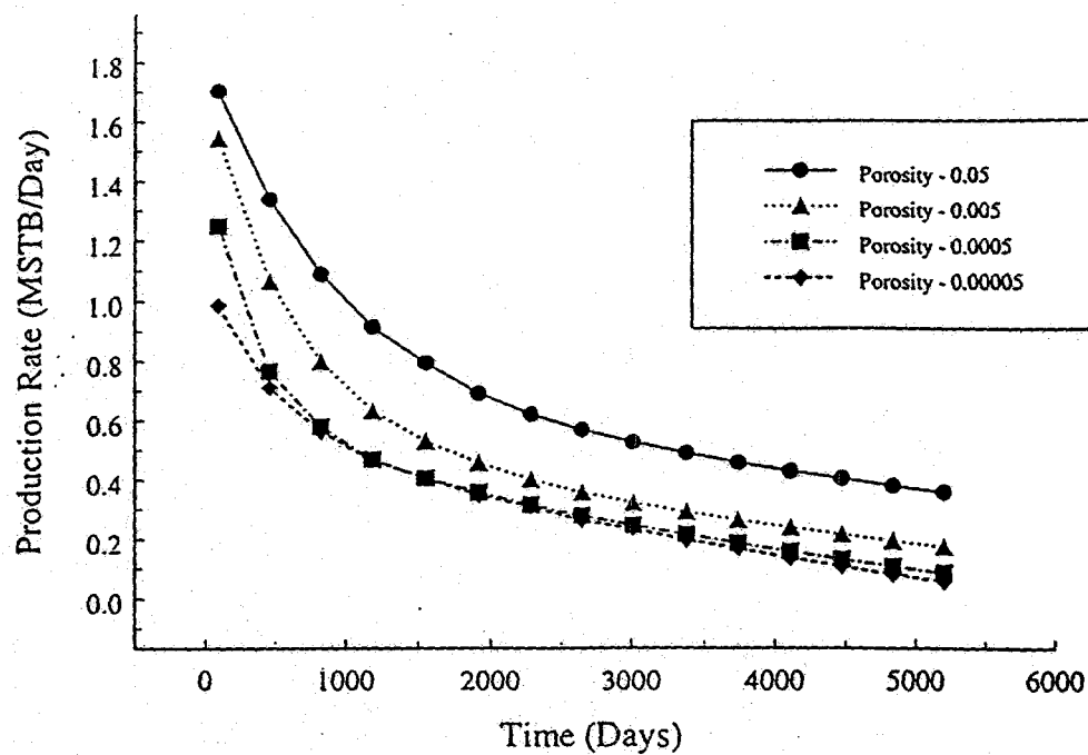
Figure 4.9. Effect of fracture porosity on oil-production rate in the 20-square-mile (51.8-km 2 ) area.
