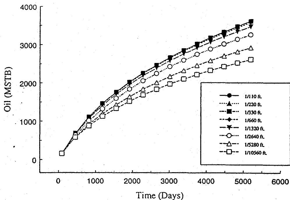
Figure 4.1. Effect of fracture spacing on cumulative oil production in the 20-square-mile (51.8-km 2 ) area.
