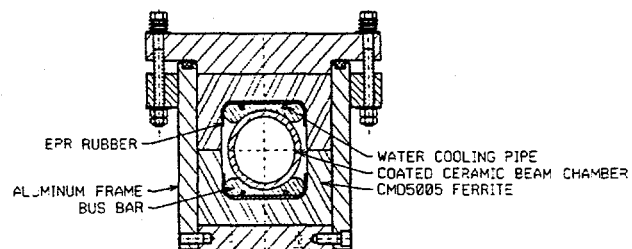
Figure 1. Cross section of the PEP II injection kicker magnet.
