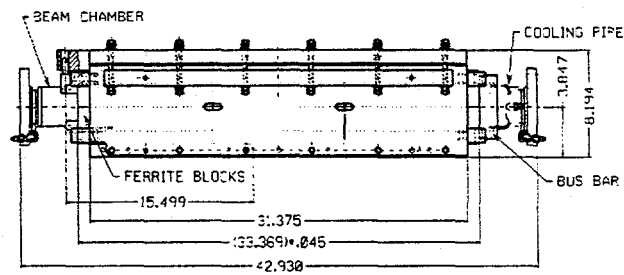
Figure 2. Longitudinal view of the PEP II HER injection kicker magnet.
