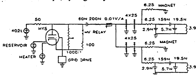
Figure 5. Schematic of the PEP II, HER injection kicker system.
