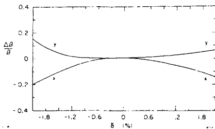
Fig. 2. Beta function variations at an interaction region.
