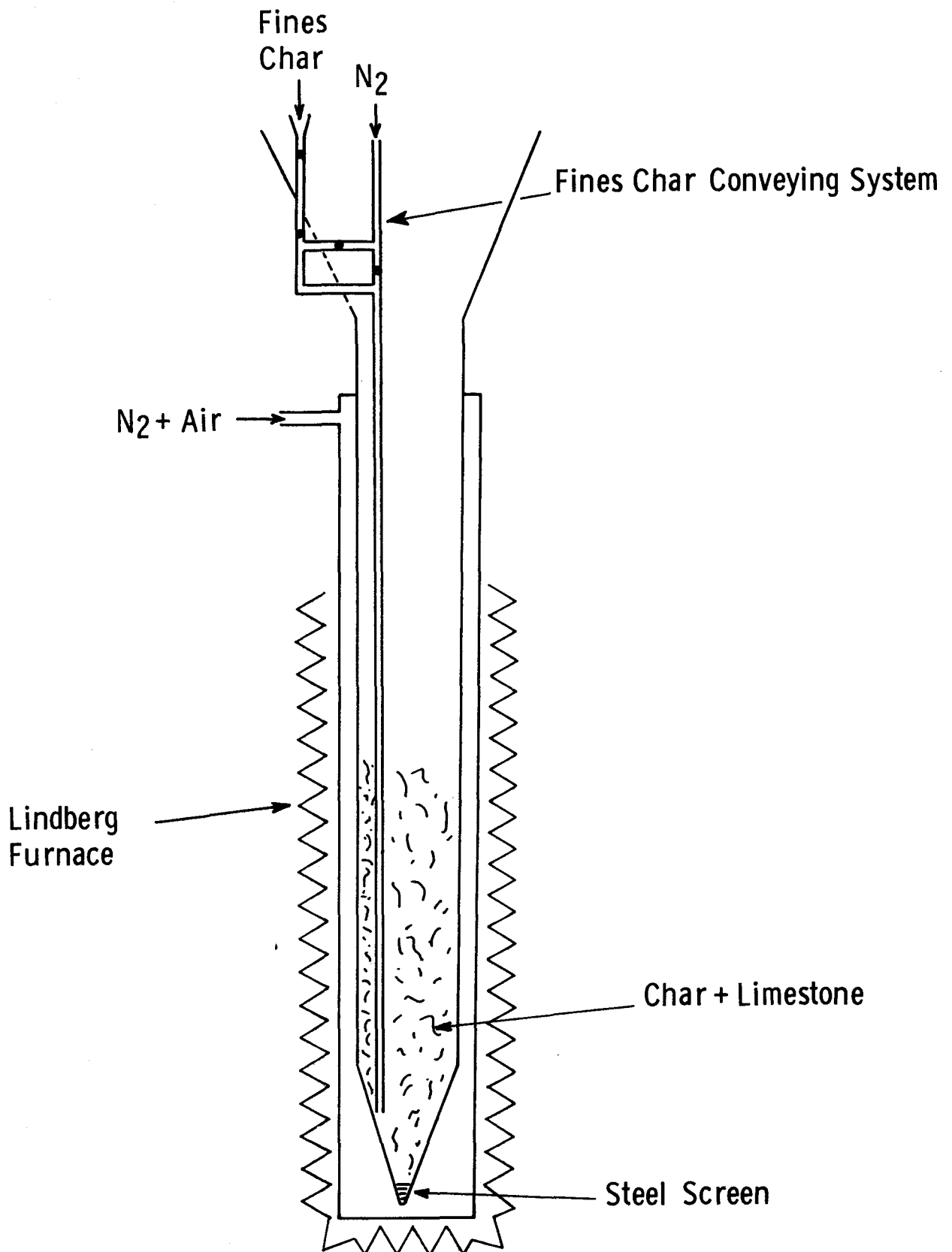
FIGURE 1.1-1 FLUIDIZED CHAR-LIMESTONE COMBUSTER
