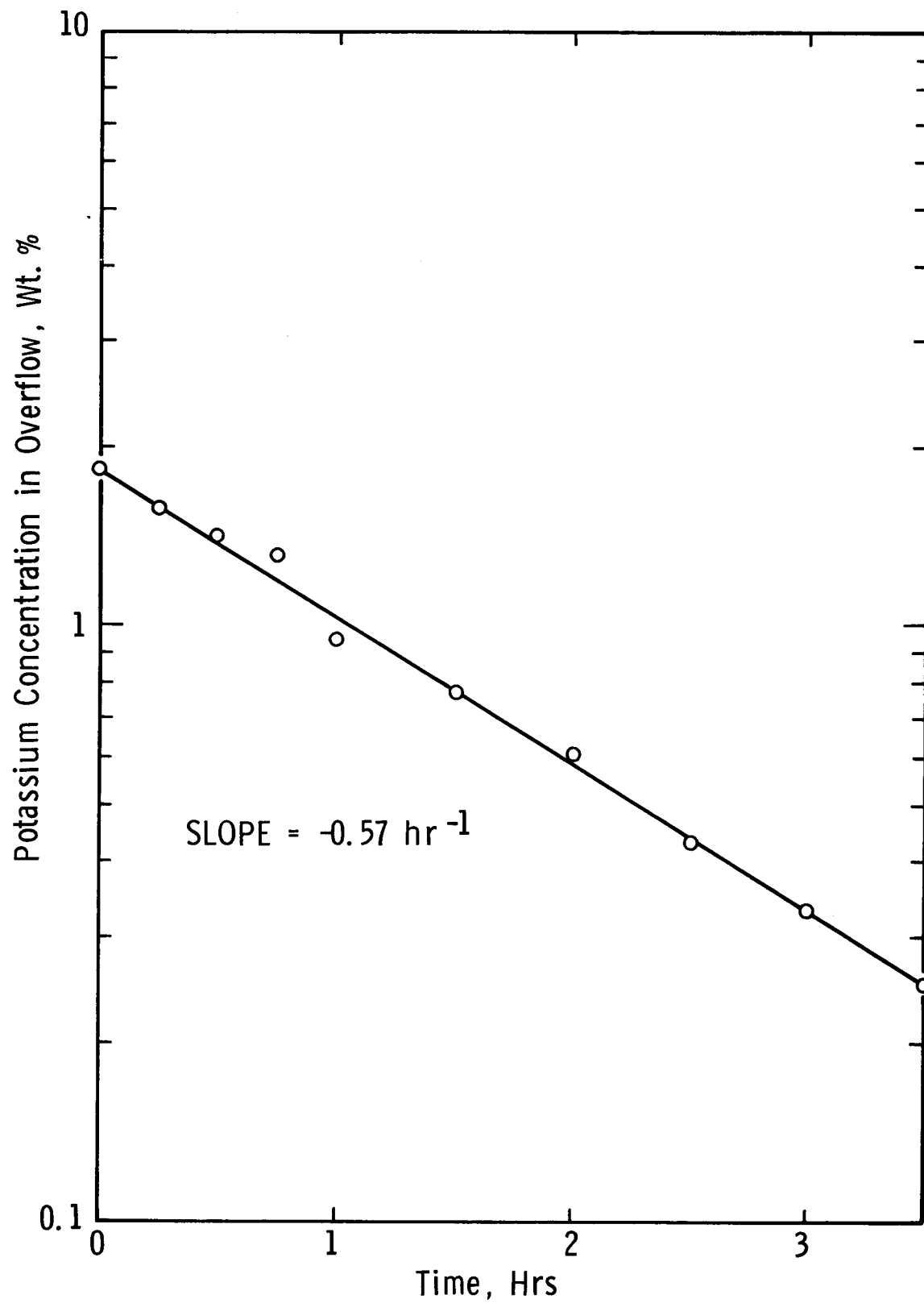
FIGURE 2.2-4 LEACHING TANK PERFORMANCE
