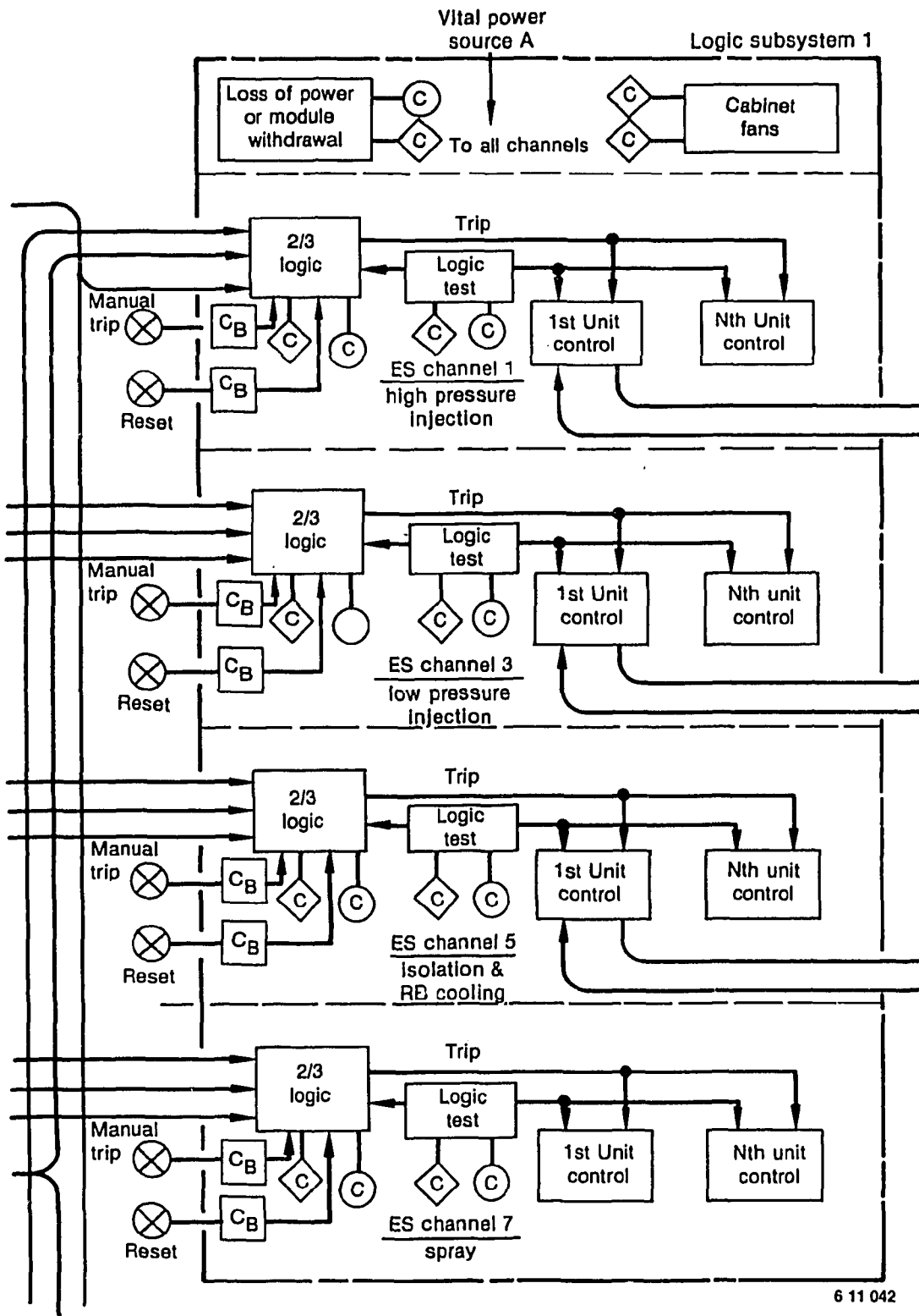
Figure 19. Logic subsystem.
