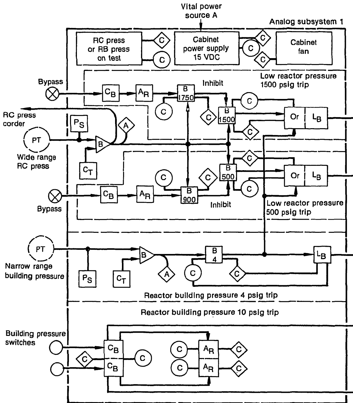
Figure 18. Analog subsystem.
