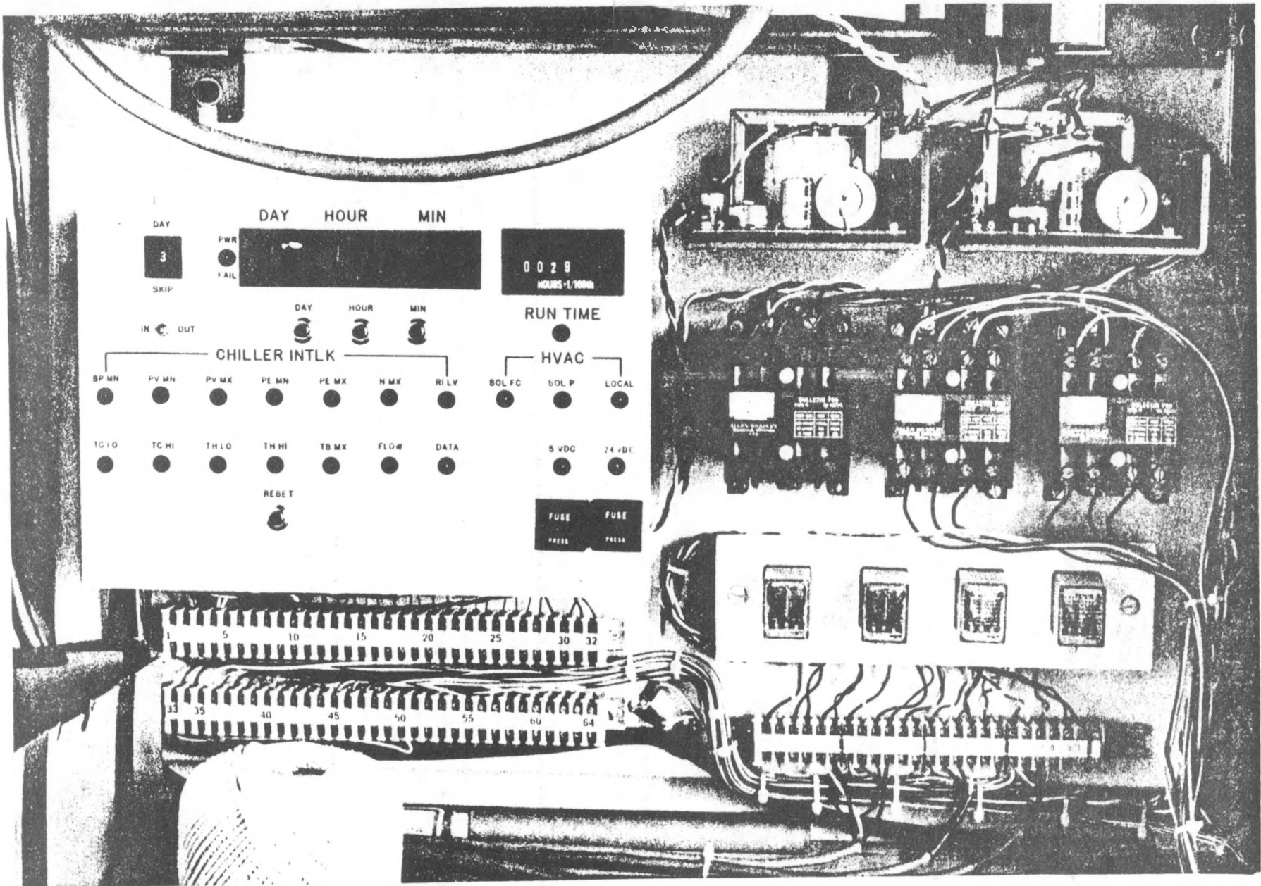
CHILLER INTERLOCK PANEL
