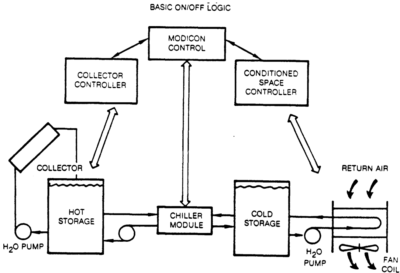
FIGURE S-4. CONTROL SYSTEM CONCEPT
