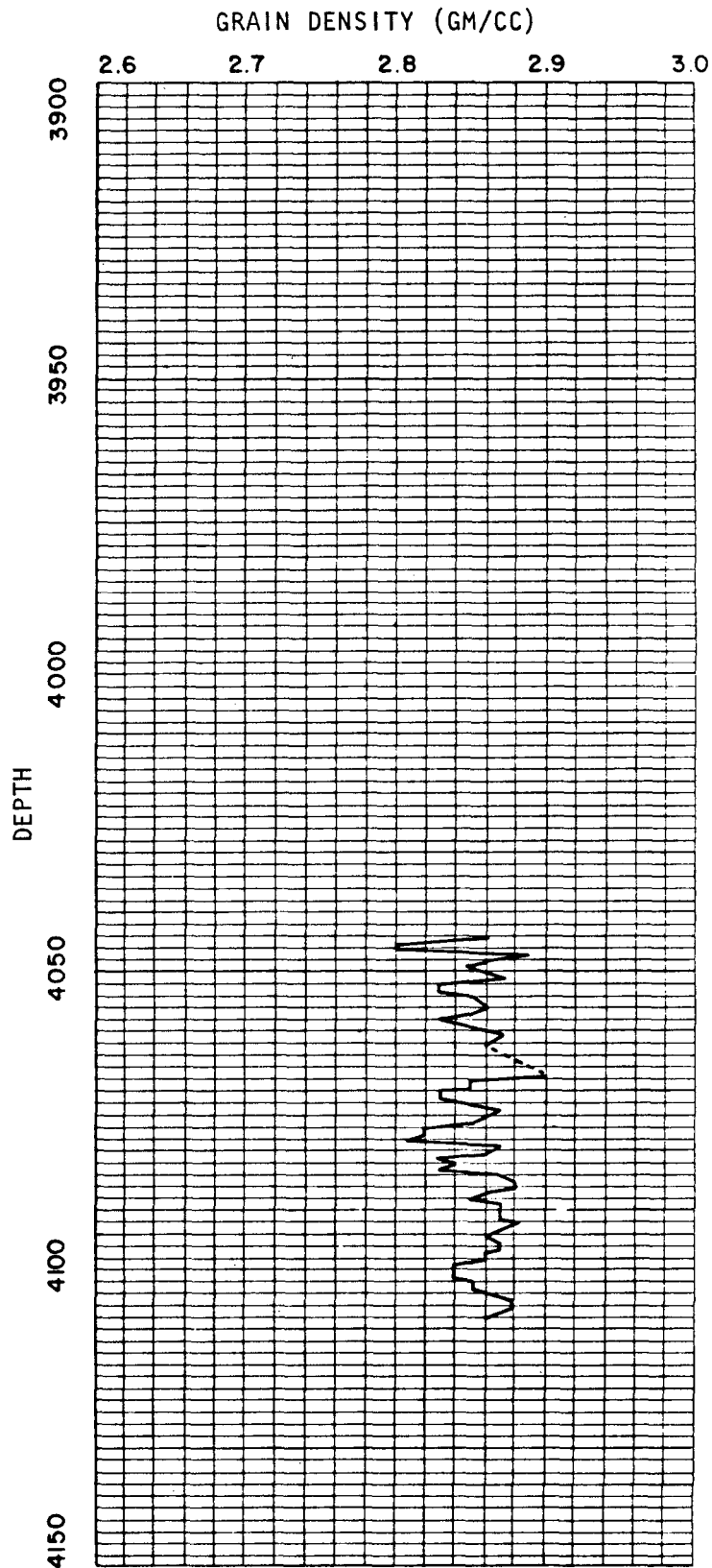
Figure 34.--Core data: grain density of recovered cores.
