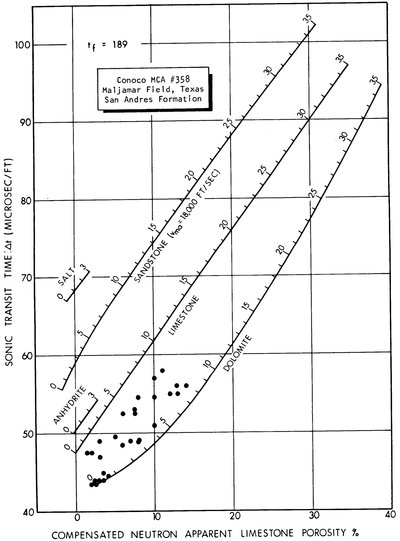
Figure 53.--Sonic-neutron cross plot, zone 7, cores 7-9.
