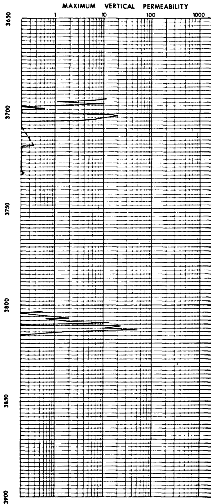
Figure 25.--Core data: maximum vertical permeability to air vs. depth.
