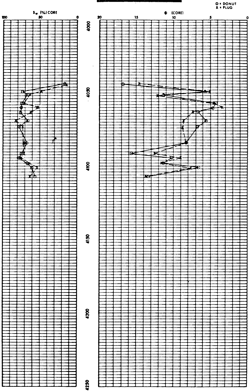
Figure 36.--Porosity and water saturation of plug and donut core samples.
