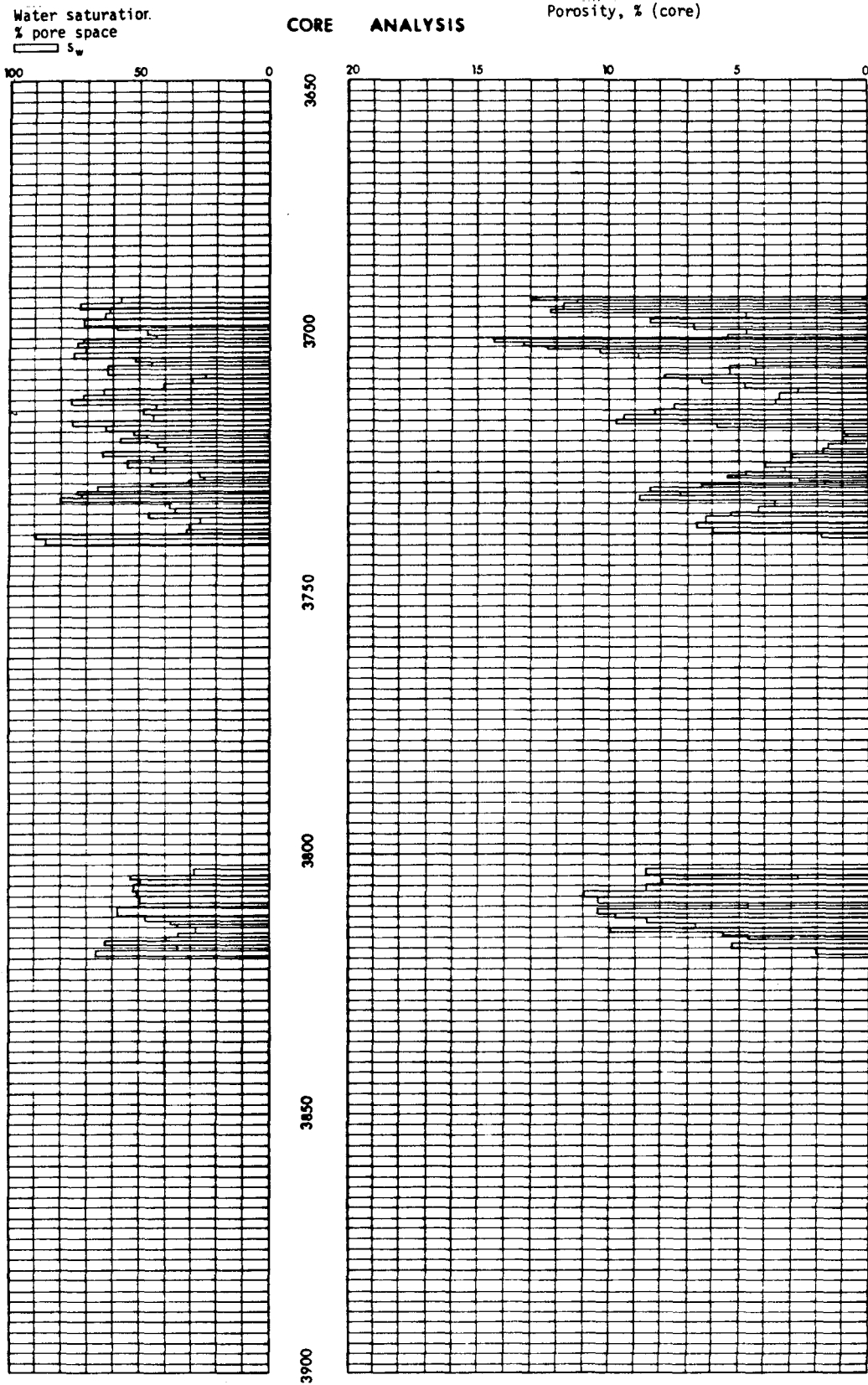
Figure 59.--Comparison of core and log analysis.
