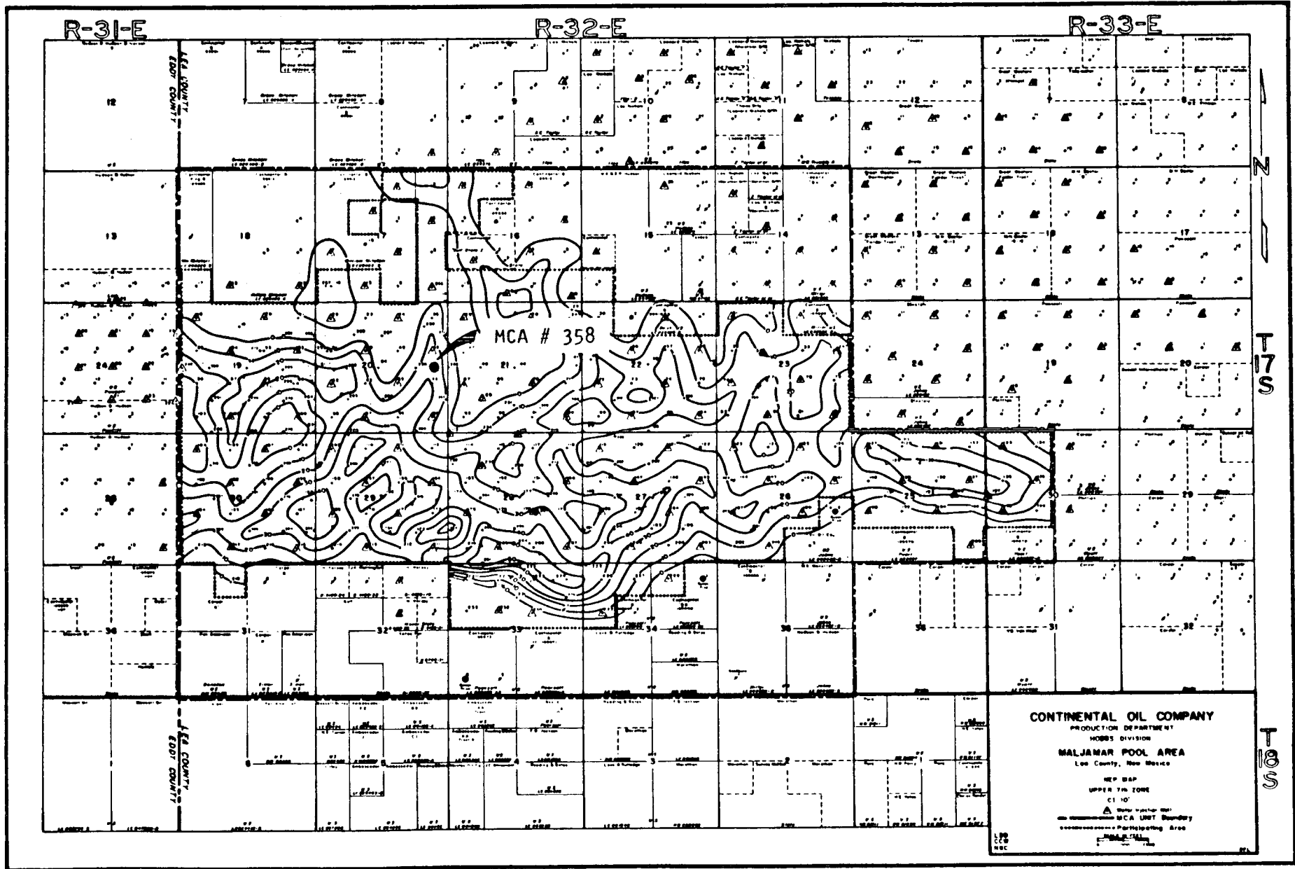
Figure 7.--Isopach map, zone 7 (upper).
