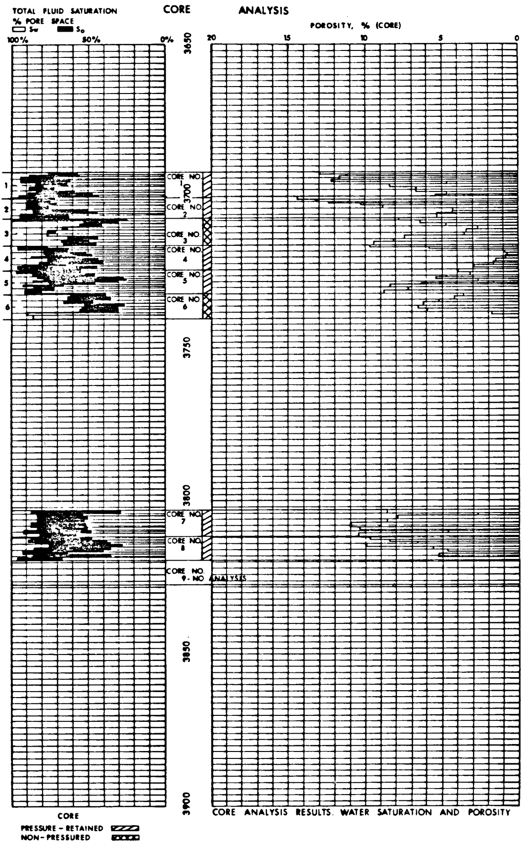
Figure 21.--Core analysis results: water saturation & porosity.
