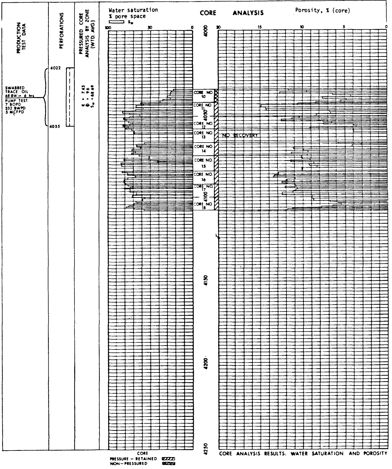
Figure 62.--Comparison of production test results and core analysis data.
