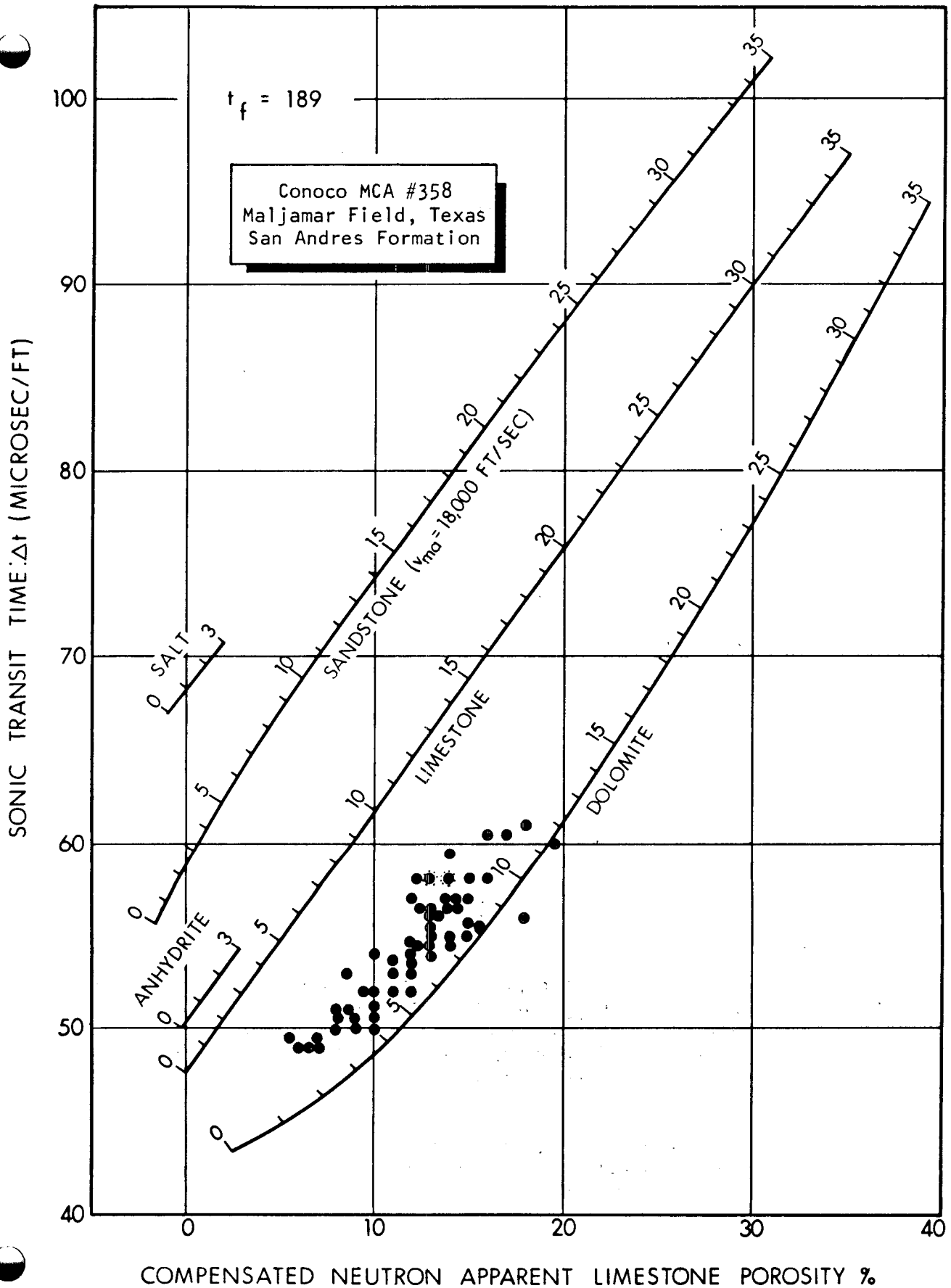
Figure 54.--Sonic-neutron cross plot, zone 9, cores 10-18.
