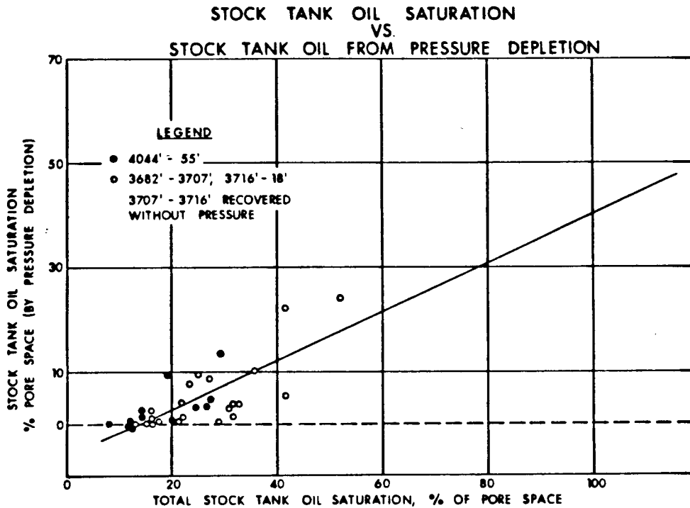
Figure 65.--Stock tank oil saturation cross-plot.
