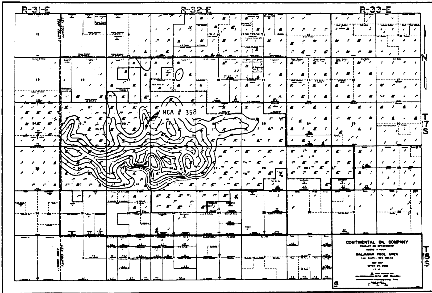
Figure 9.--Isopach map, zone 9 (upper).
