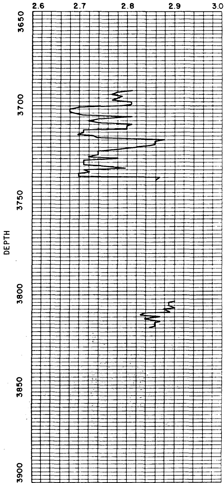
Figure 33.--Core data: grain density of recovered cores.
