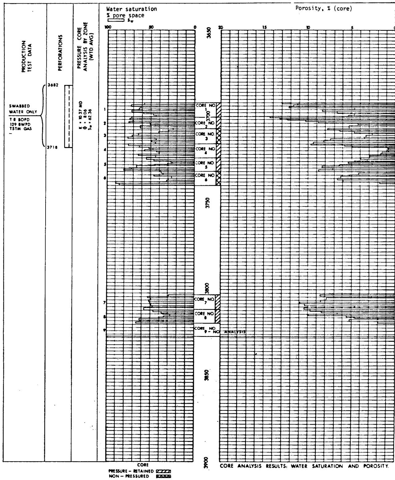
Figure 61.--Comparison of production test results and core analysis data.
