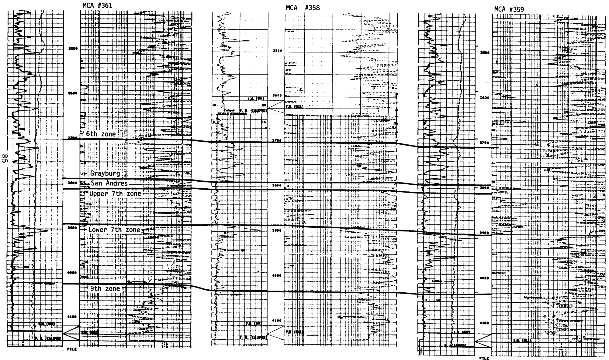
Figure 48.--Cross-section line 1-1'.
