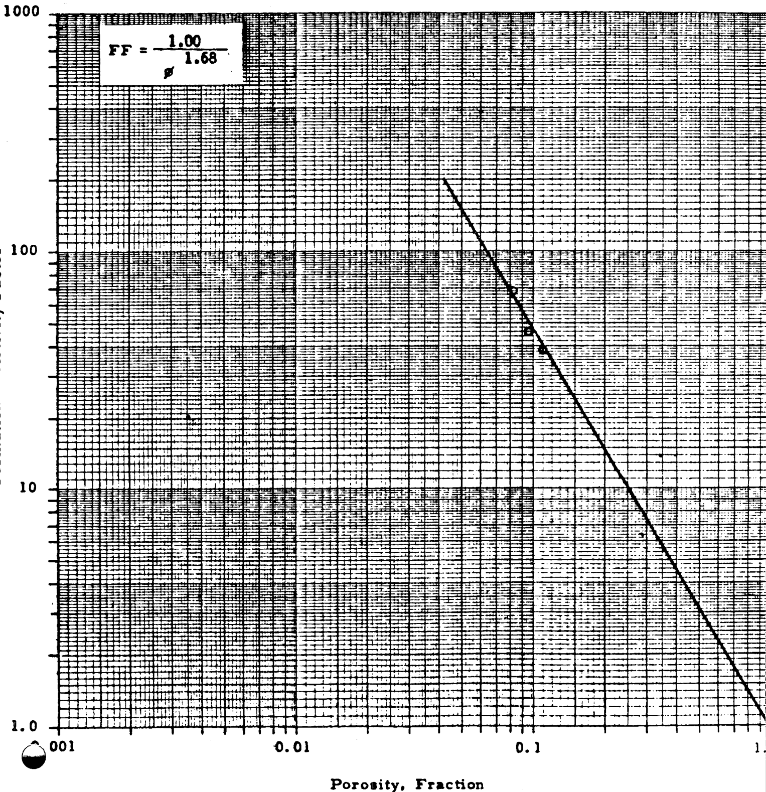
Figure 42.--Determination of cementation exponent m for sandstone samples.
