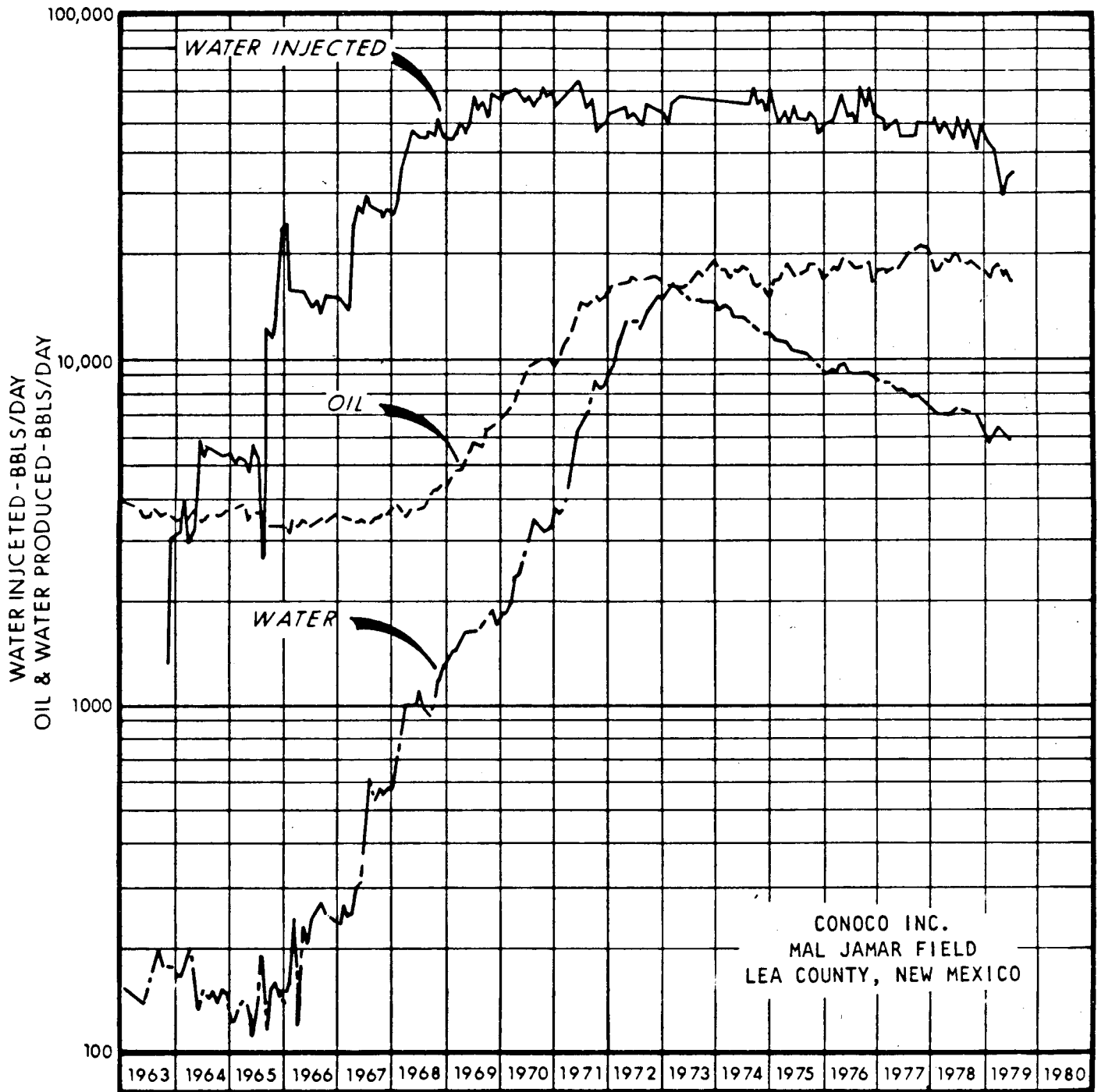
Figure 12.--MCA unit performance curve.
