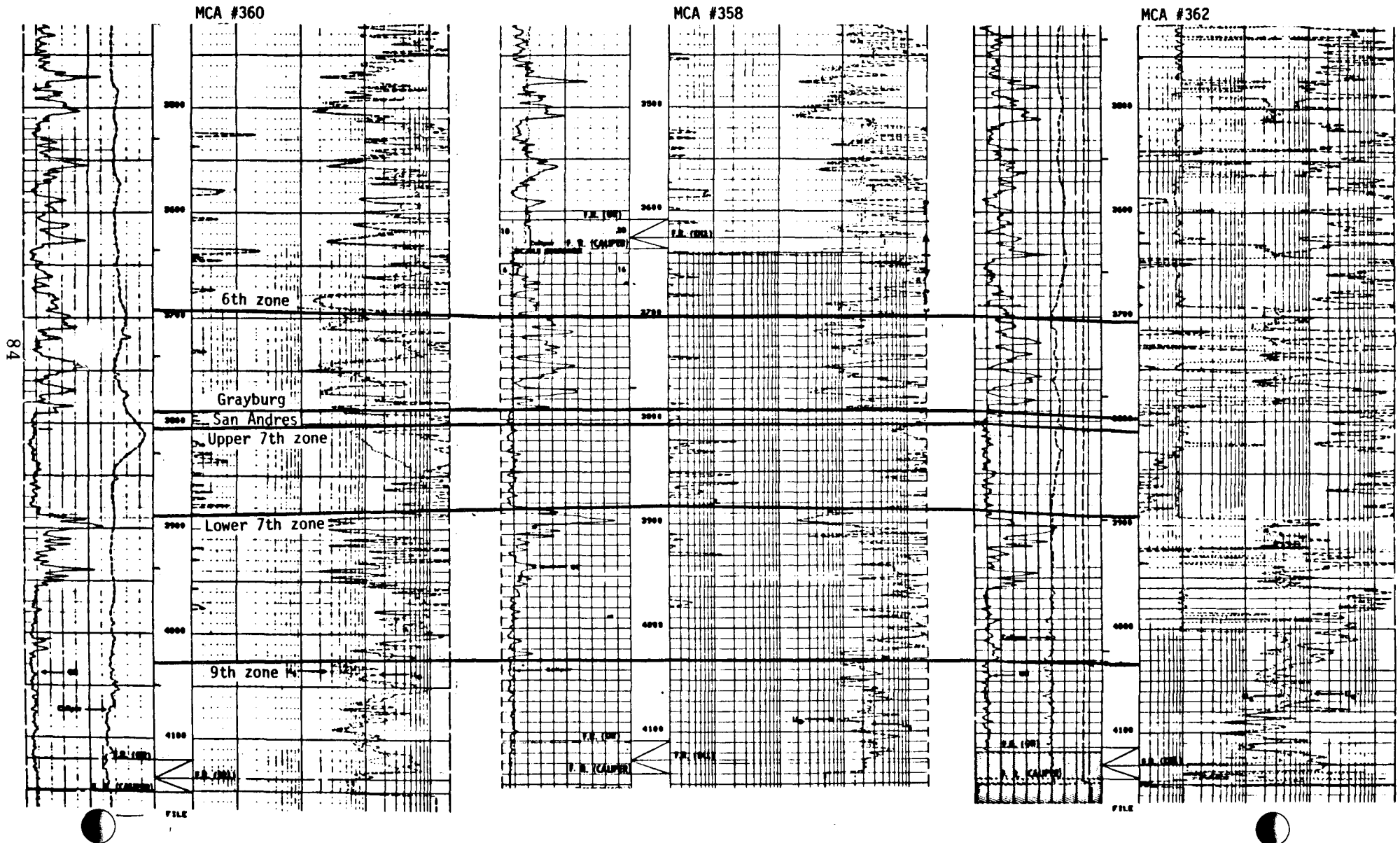
Figure 47.--Cross-section line 2-2'.
