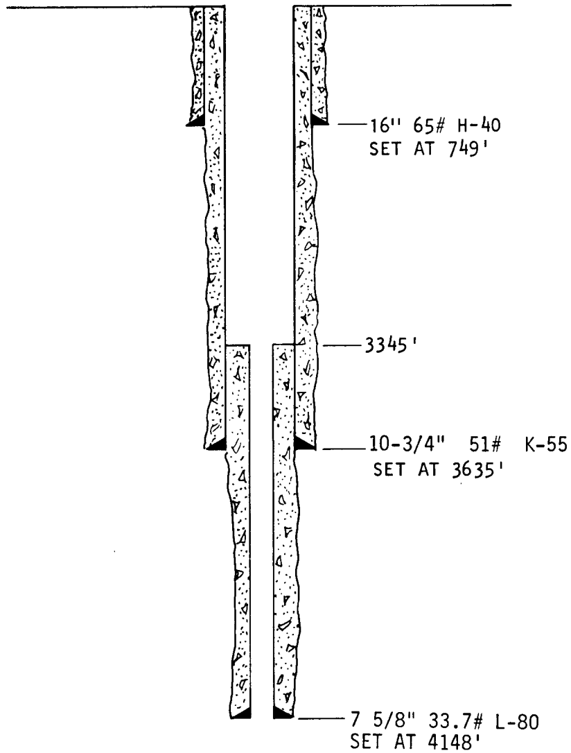
Completion diagram.
