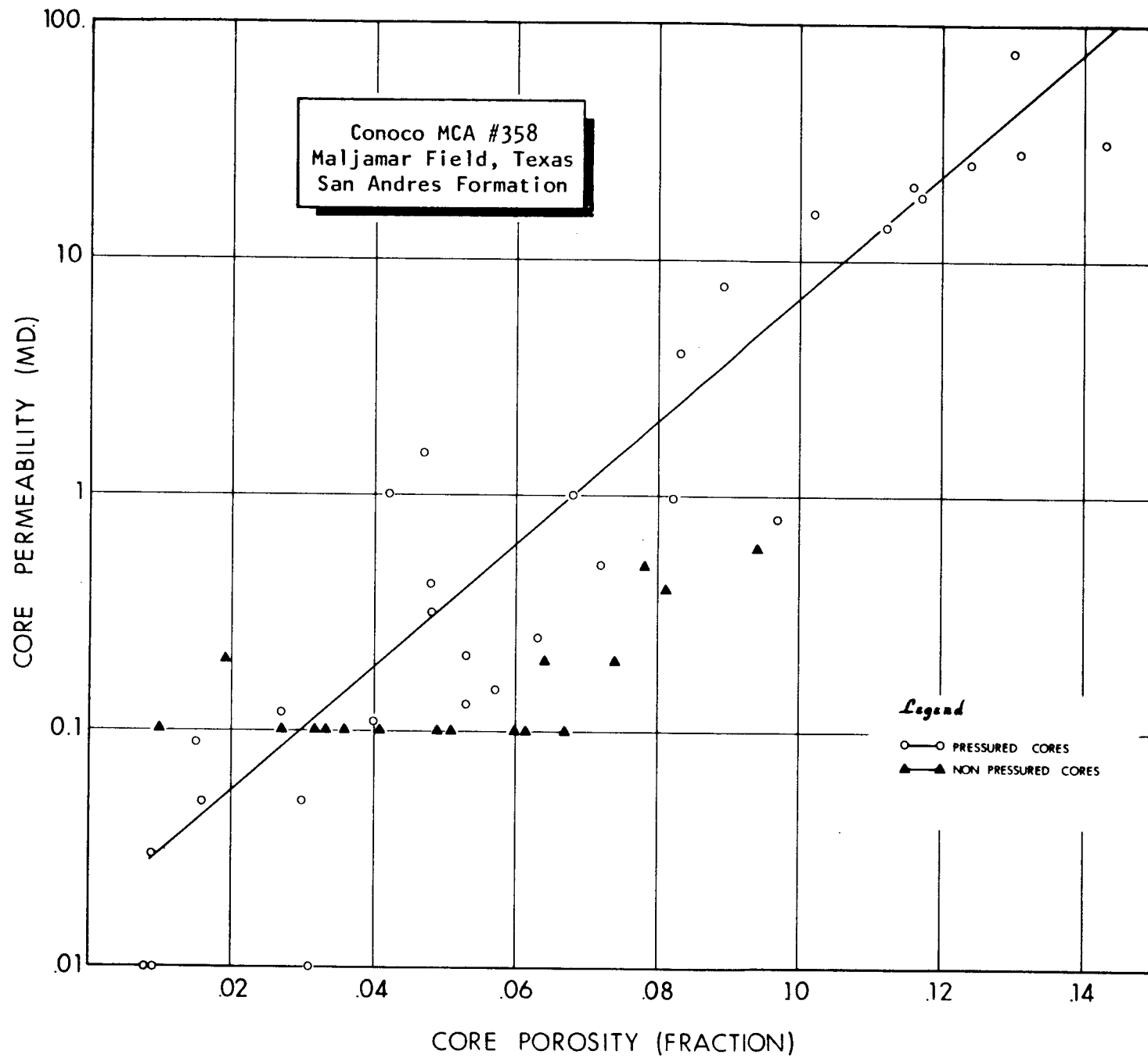
Figure 27.--Porosity versus maximum horizontal permeability to air, zone 6, cores 1-6.
