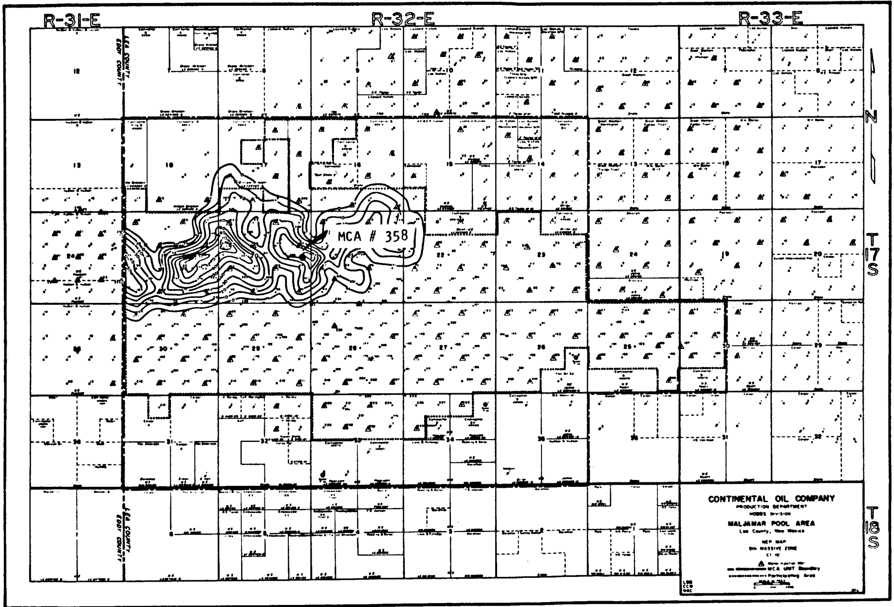
Figure 10.--Isopach map, zone 9 (massive).
