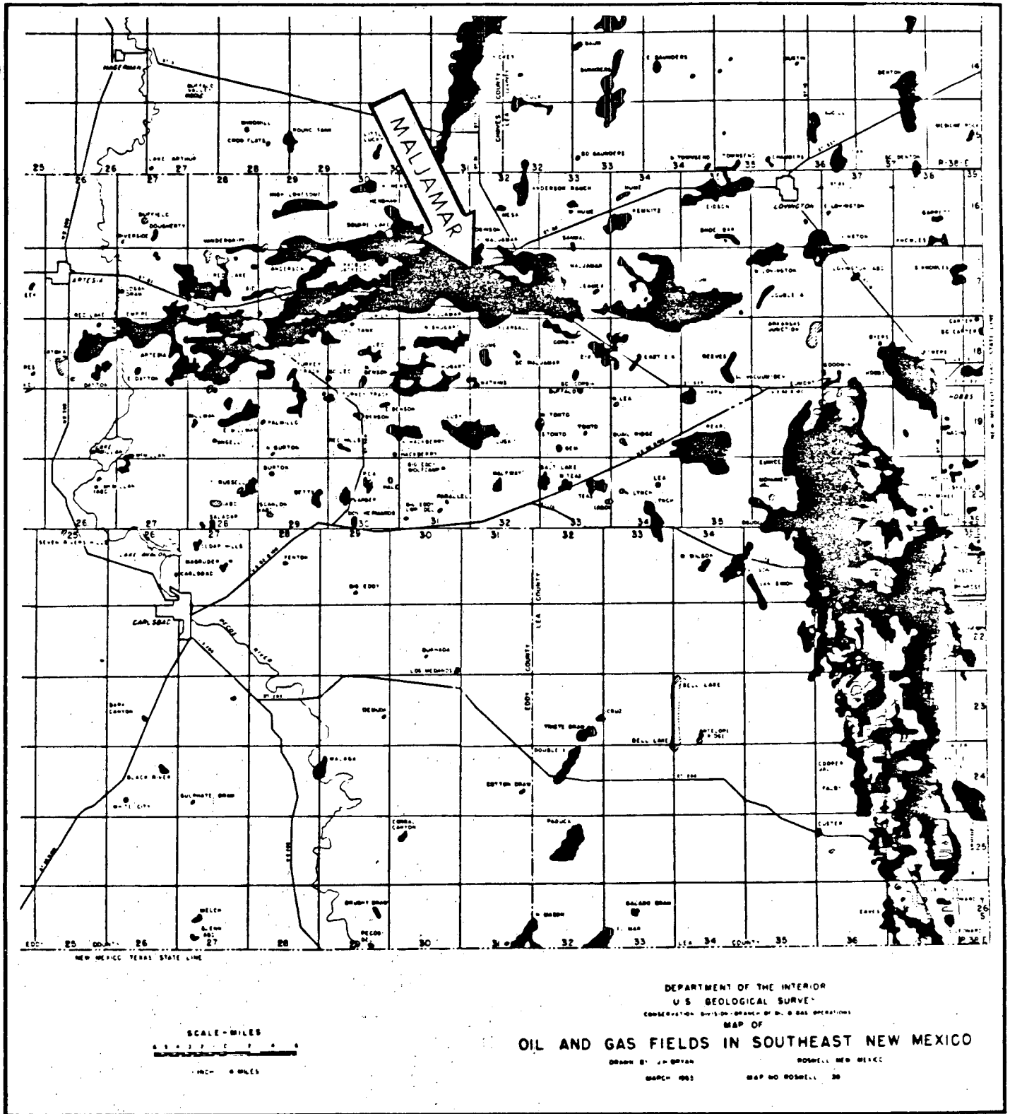
Figure 2.--Location of Maljamar field in southeast New Mexico.
