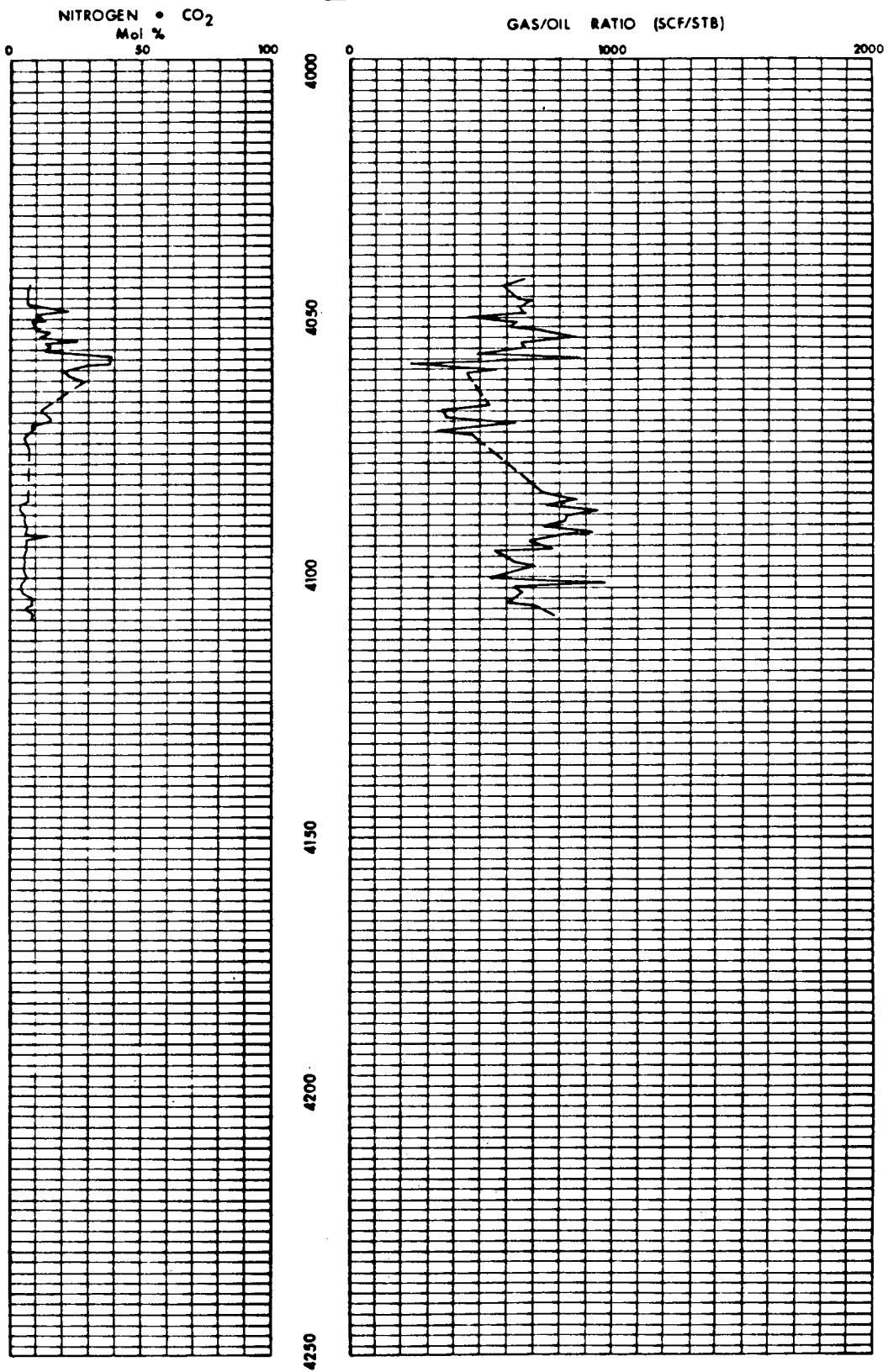
Figure 41.--N 2 and CO 2 concentration and gas/oil ratio for full diameter cores recovered with pressure.
