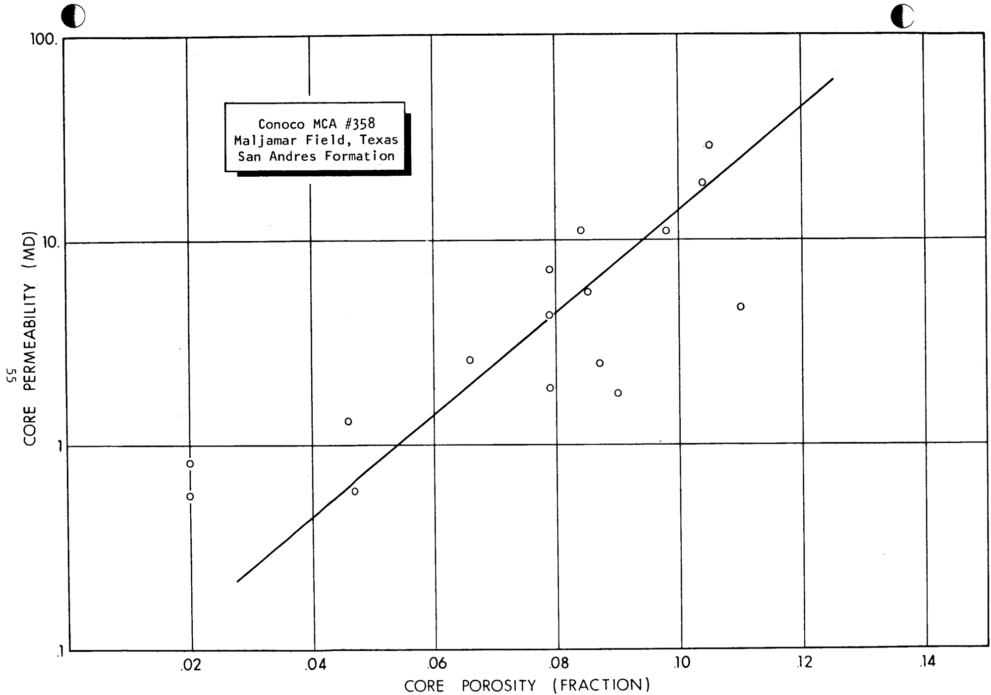
Figure 28.--Porosity versus maximum horizontal permeability to air, zone 7, cores 7-9.
