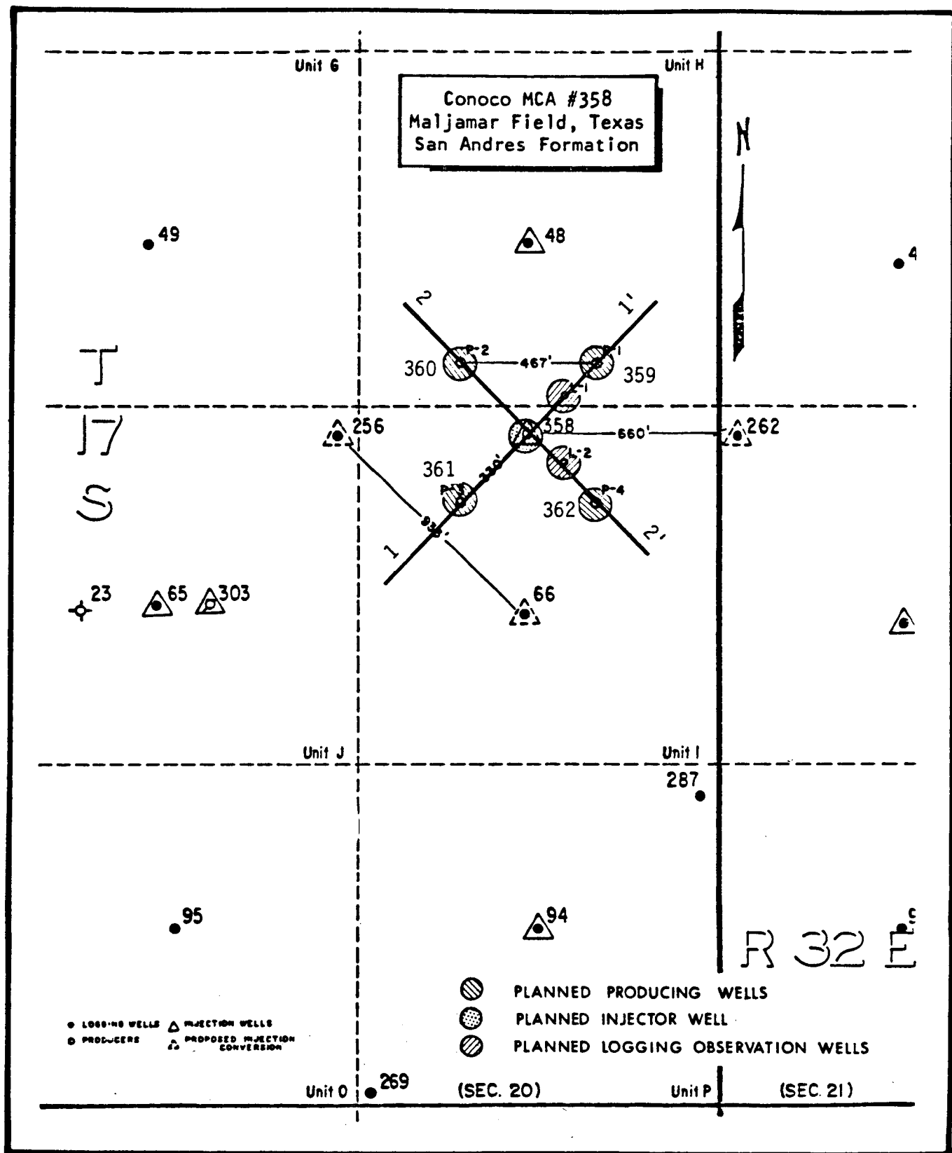
Figure 46.--Location of wells in geologic correlation and cross-section lines.
