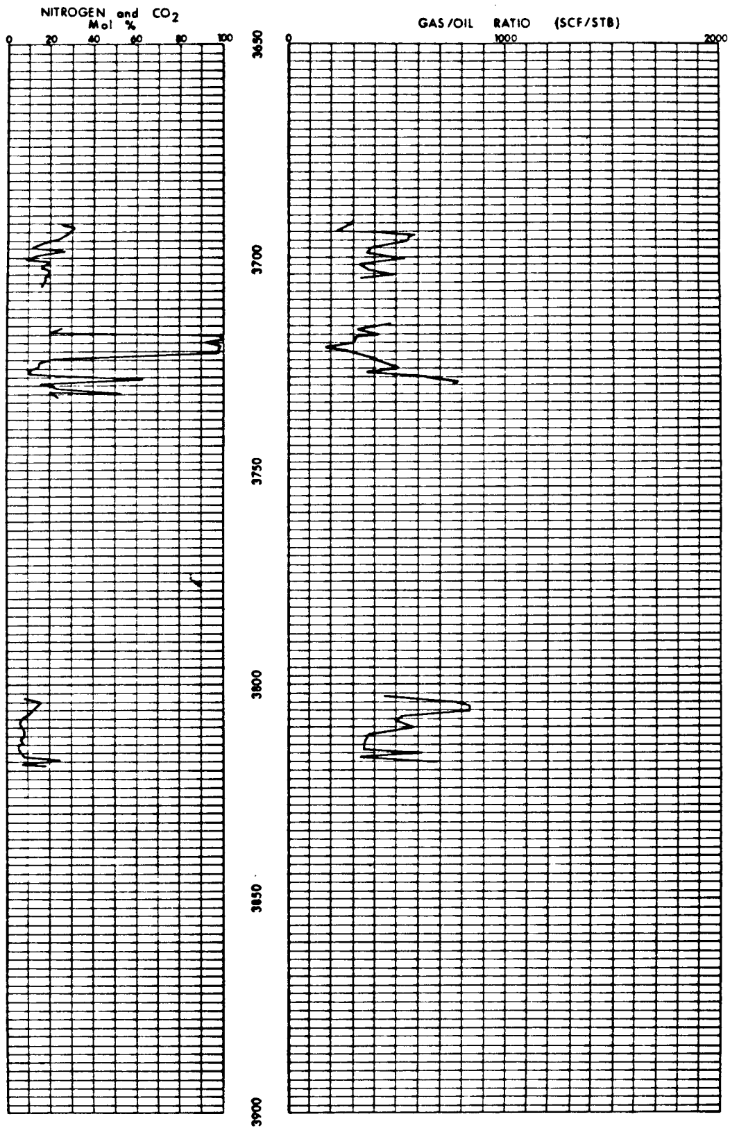
Figure 40.--N 2 and CO 2 concentration and gas/oil ratio for full diameter cores recovered with pressure.
