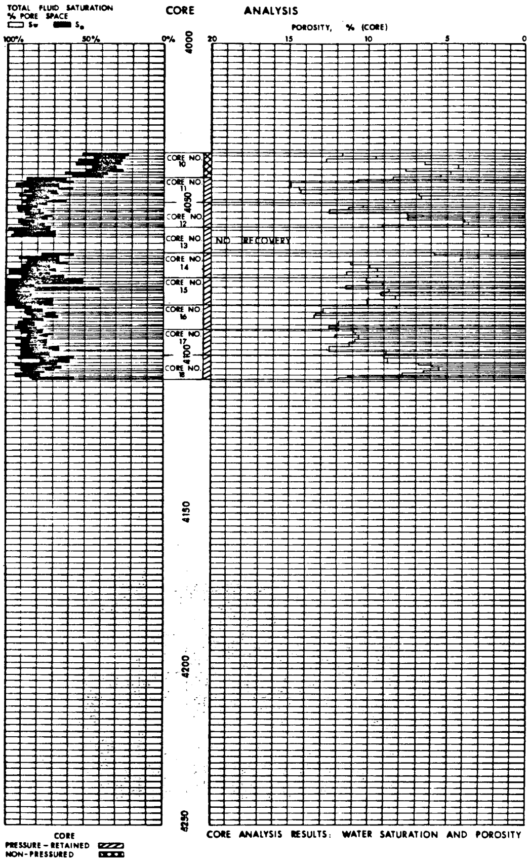
Figure 22.--Core analysis results: water saturation & porosity.
