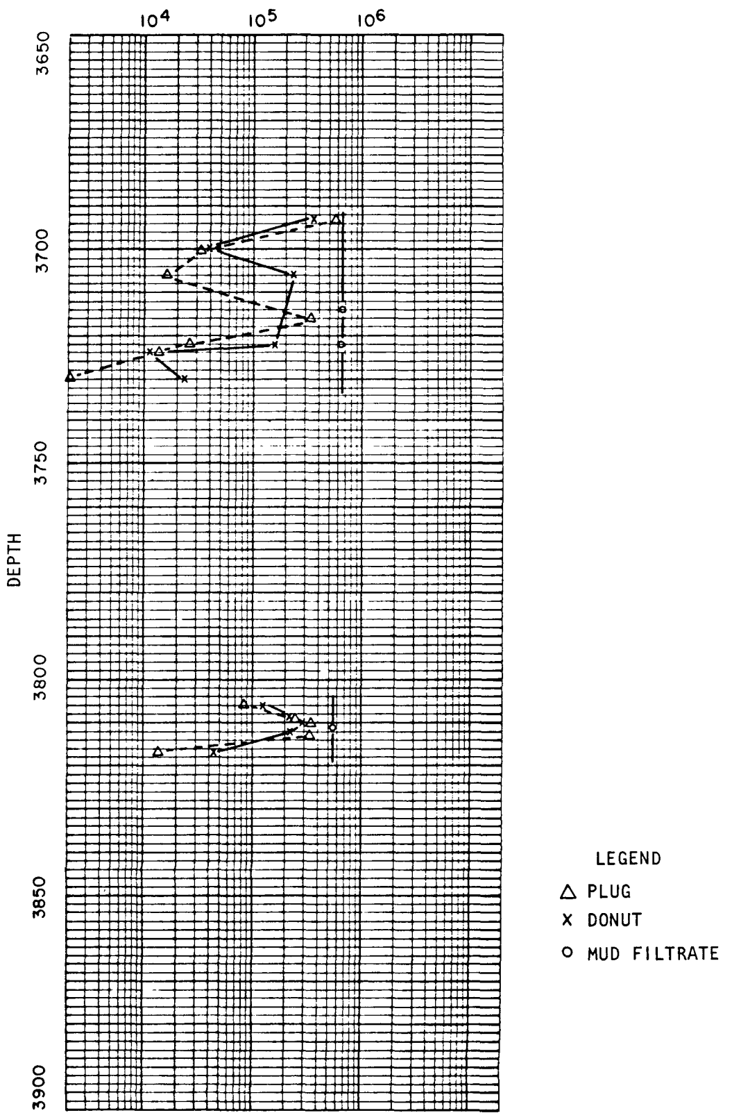
Figure 37.--Tritium activity of plug and donut pore water.
