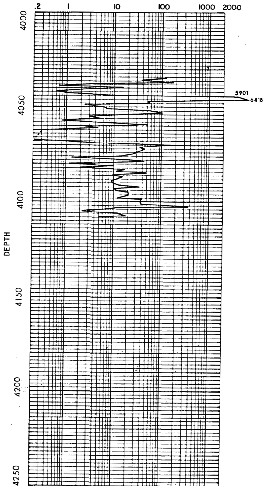
Figure 24.--Core data: maximum horizontal permeability to air vs. depth.
