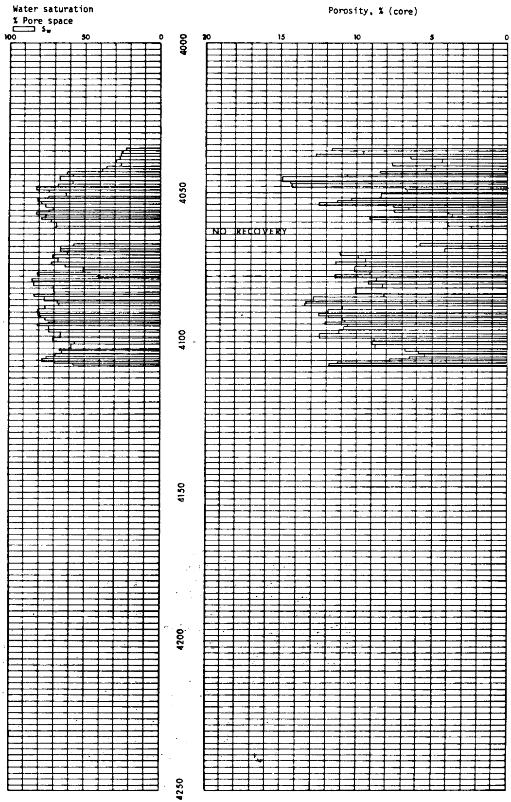
Figure 60.--Comparison of core and log analysis.
