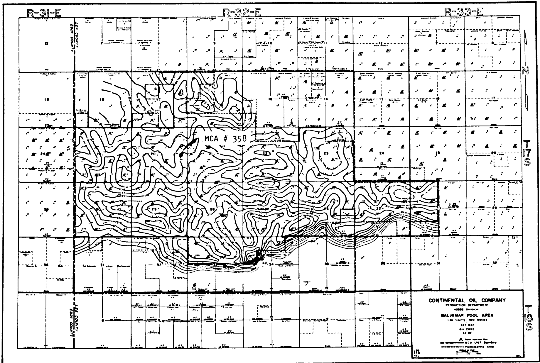
Figure 6.--Isopach map, zone 6.
