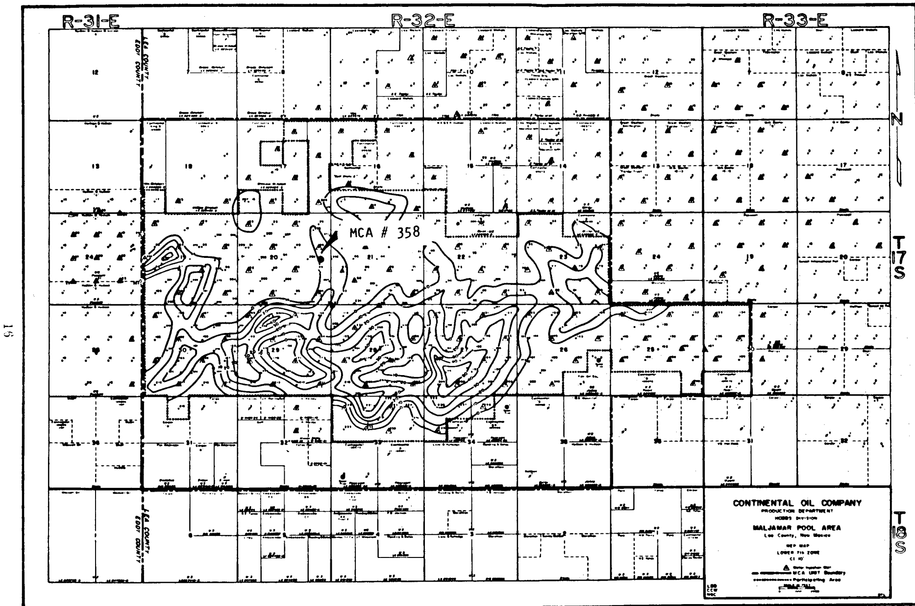
Figure 8.--Isopach map, zone 7 (lower).
