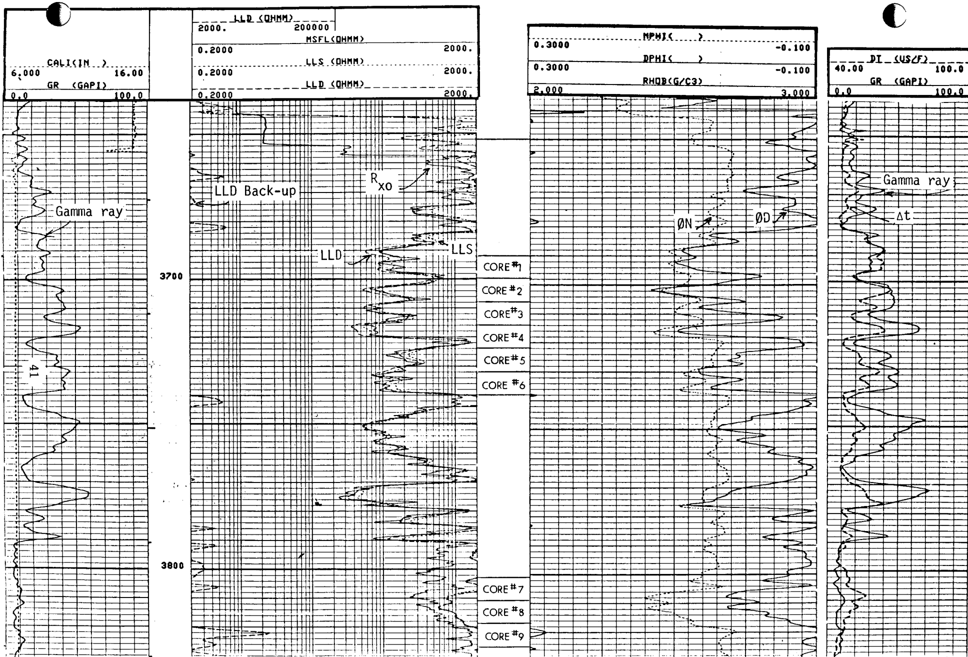
Figure 18.--Logging suite from MCA unit 358.
