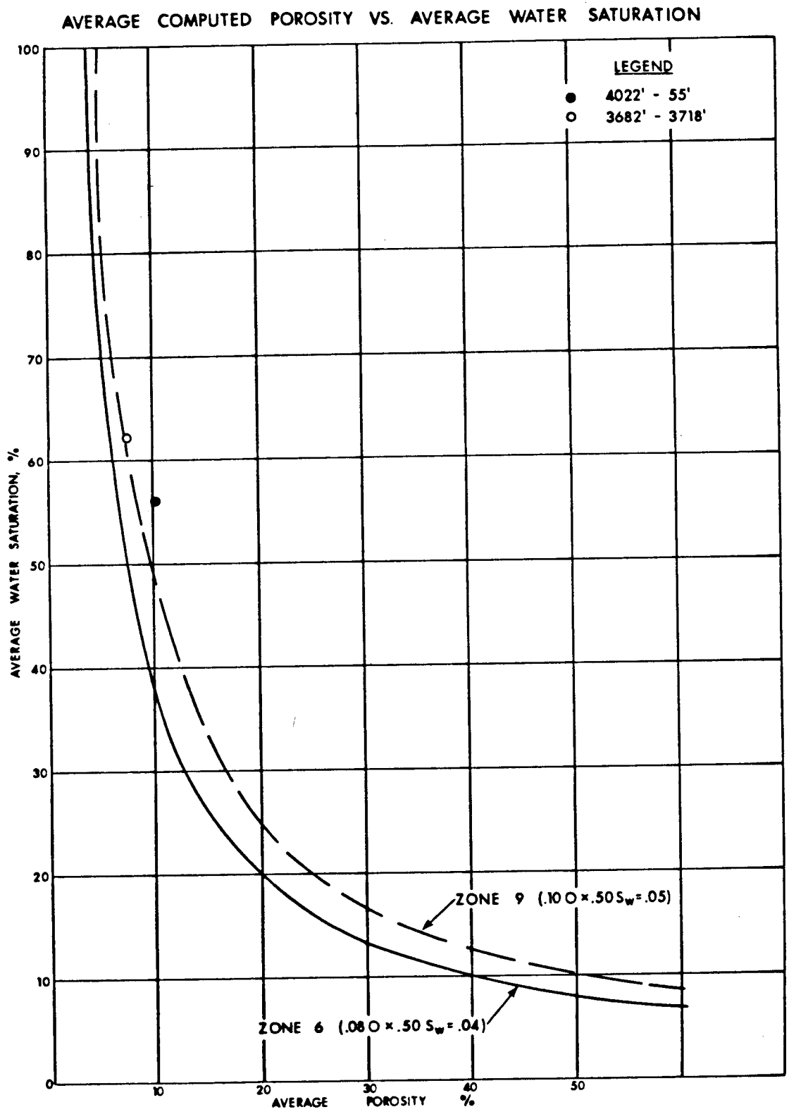
Figure 64.--Average computed porosity versus average water saturation.
