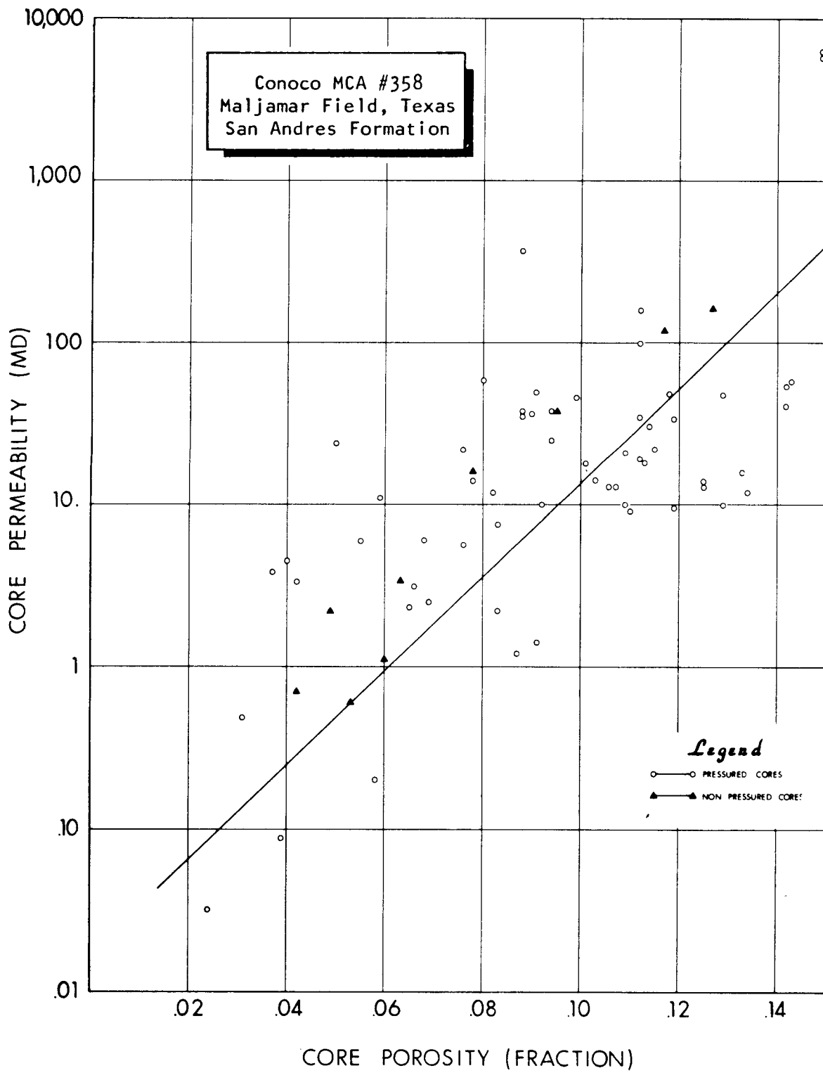
Figure 29.--Porosity versus maximum horizontal permeability to air, zone 9, cores 10-8.
