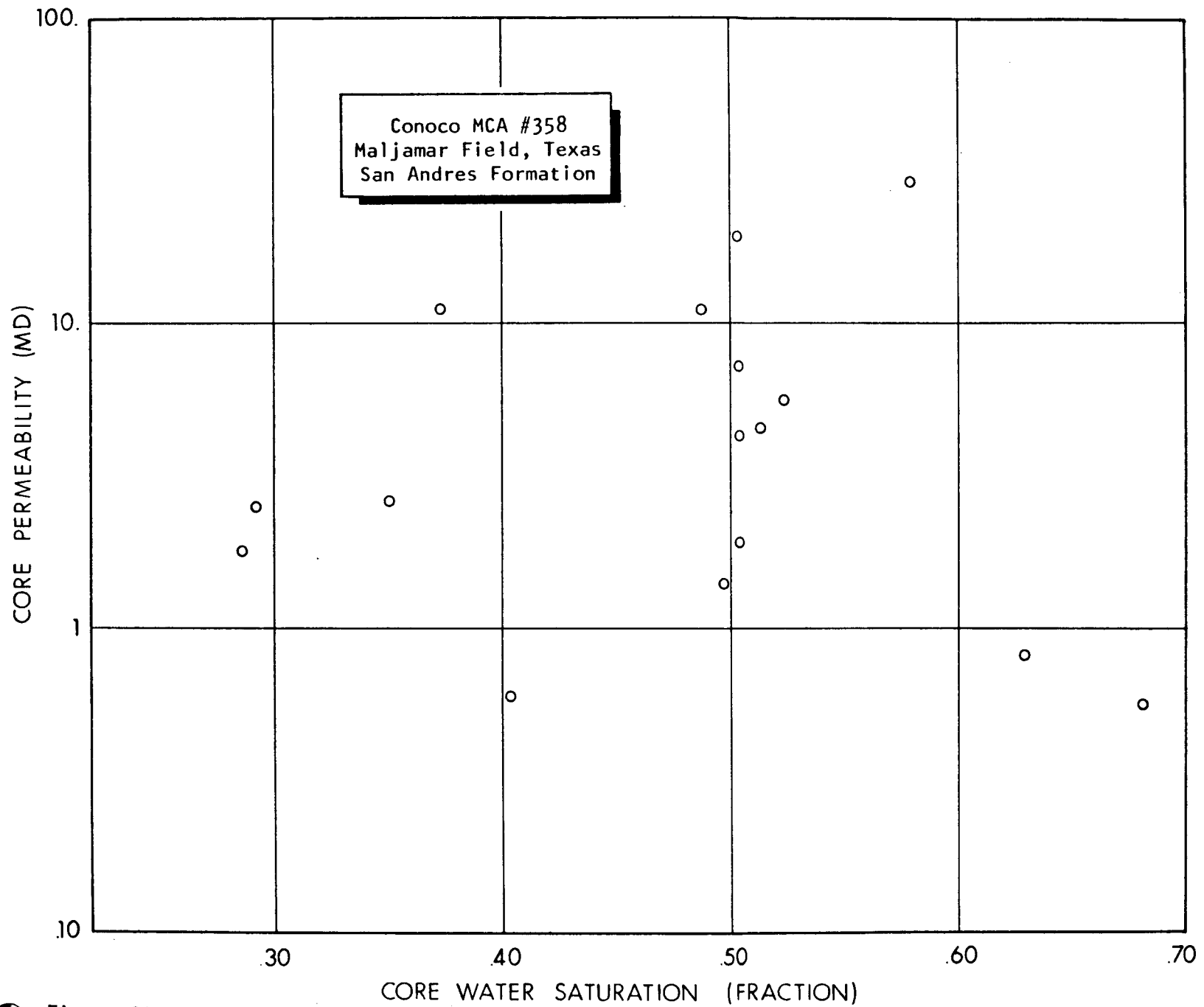
Figure 31.--Salt water saturation versus maximum horizontal permeability to air, zone 7, cores 7-9.
