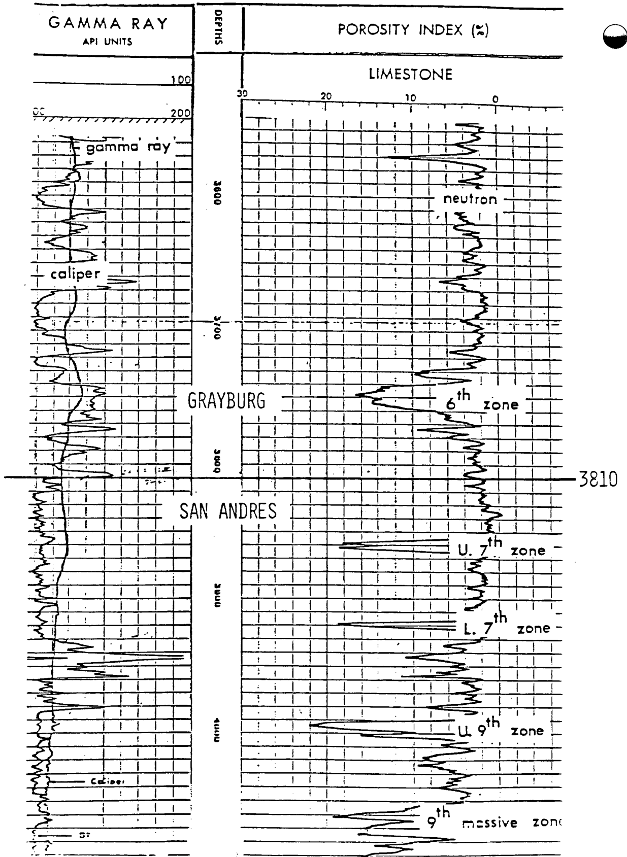
Figure 5.--Well log MCA Unit #287.
