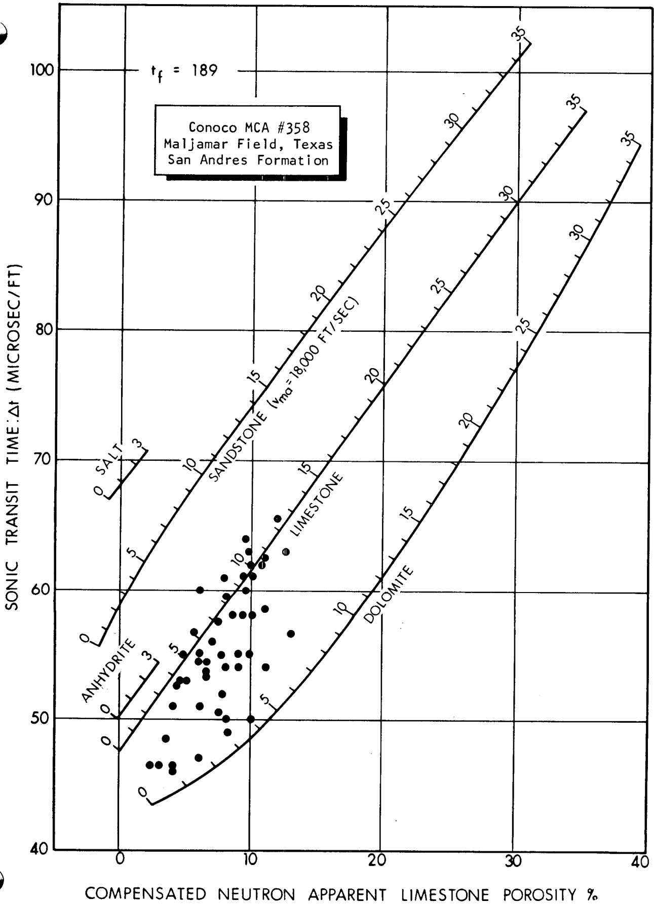
Figure 52.--Sonic-neutron cross plot, zone 6, cores 1-6.
