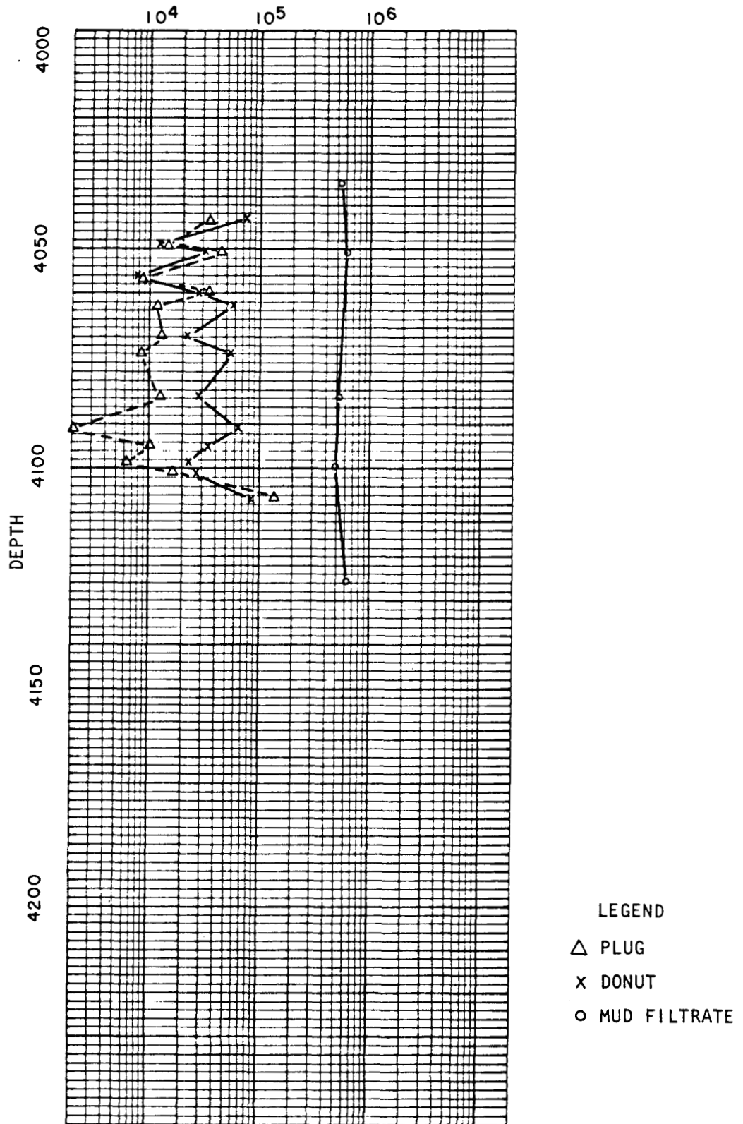
Figure 38.--Tritium activity of plug and donut pore water.
