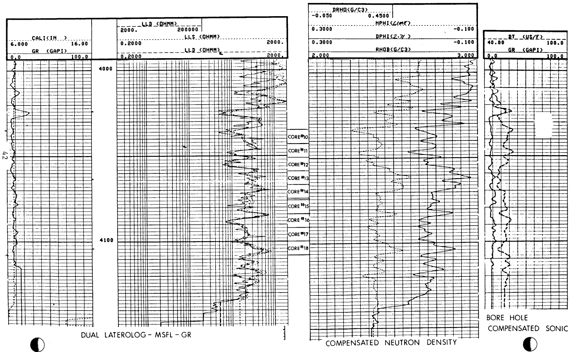
Figure 19.--Logging suite from MCA unit 358.
