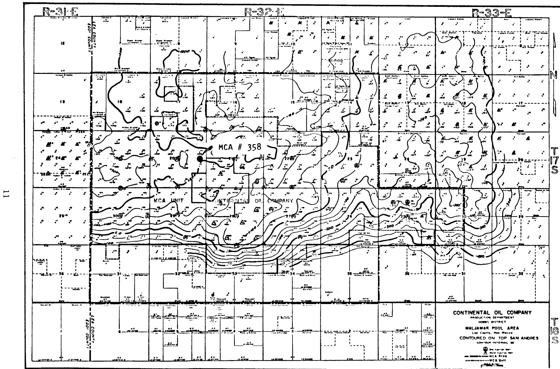
Figure 4.--Structure map on top of the San Andres.
