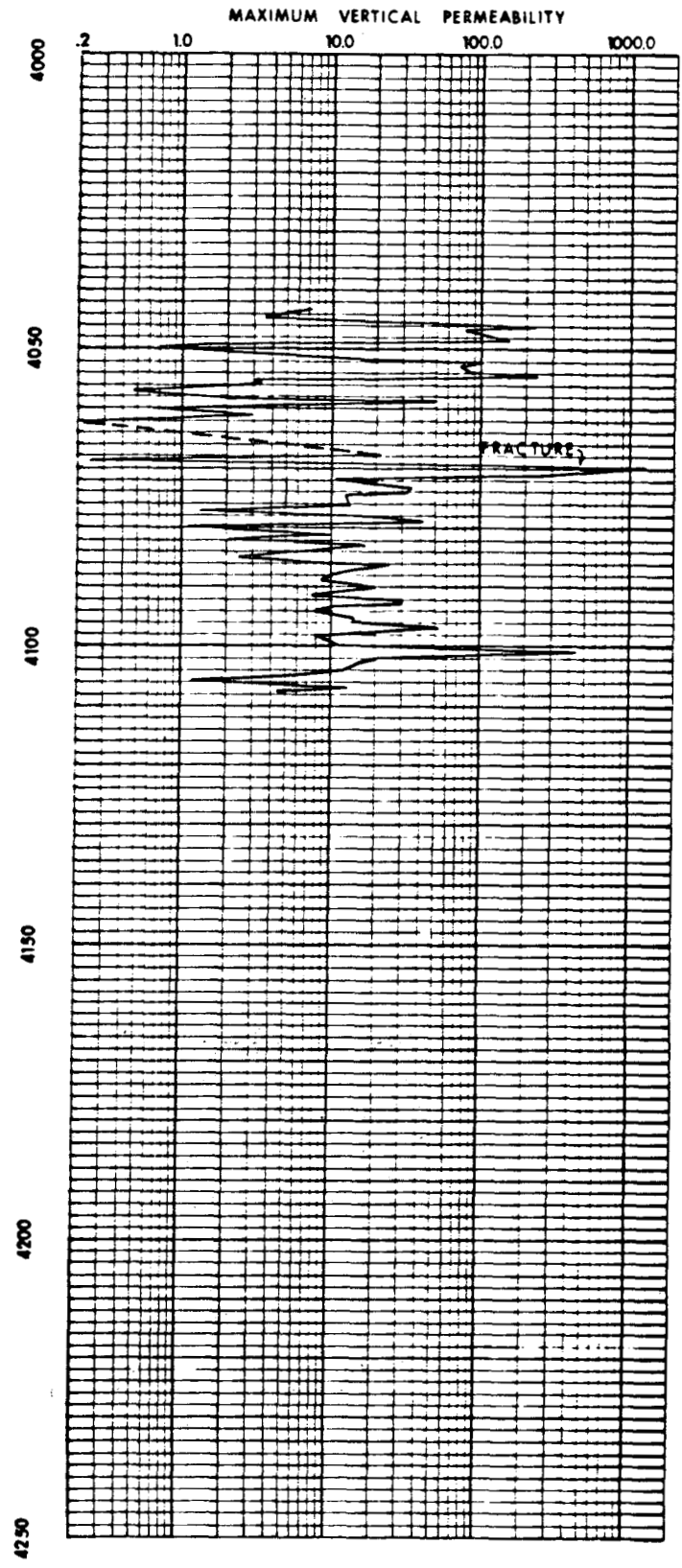
Figure 26.--Core data: maximum vertical permeability to air vs. depth.
