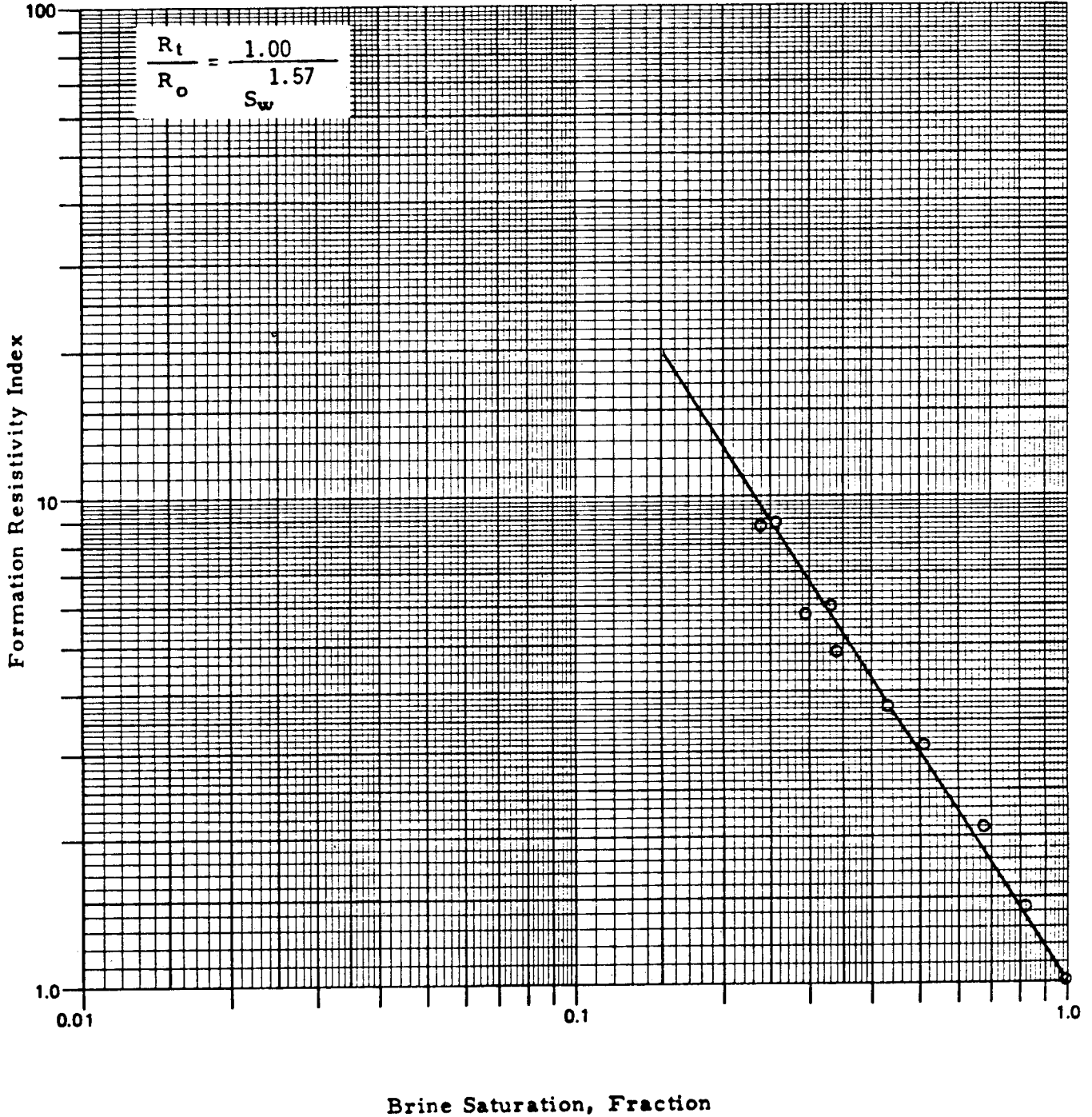
Figure 44.--Determination of saturation exponent n composite for sandstone samples.
