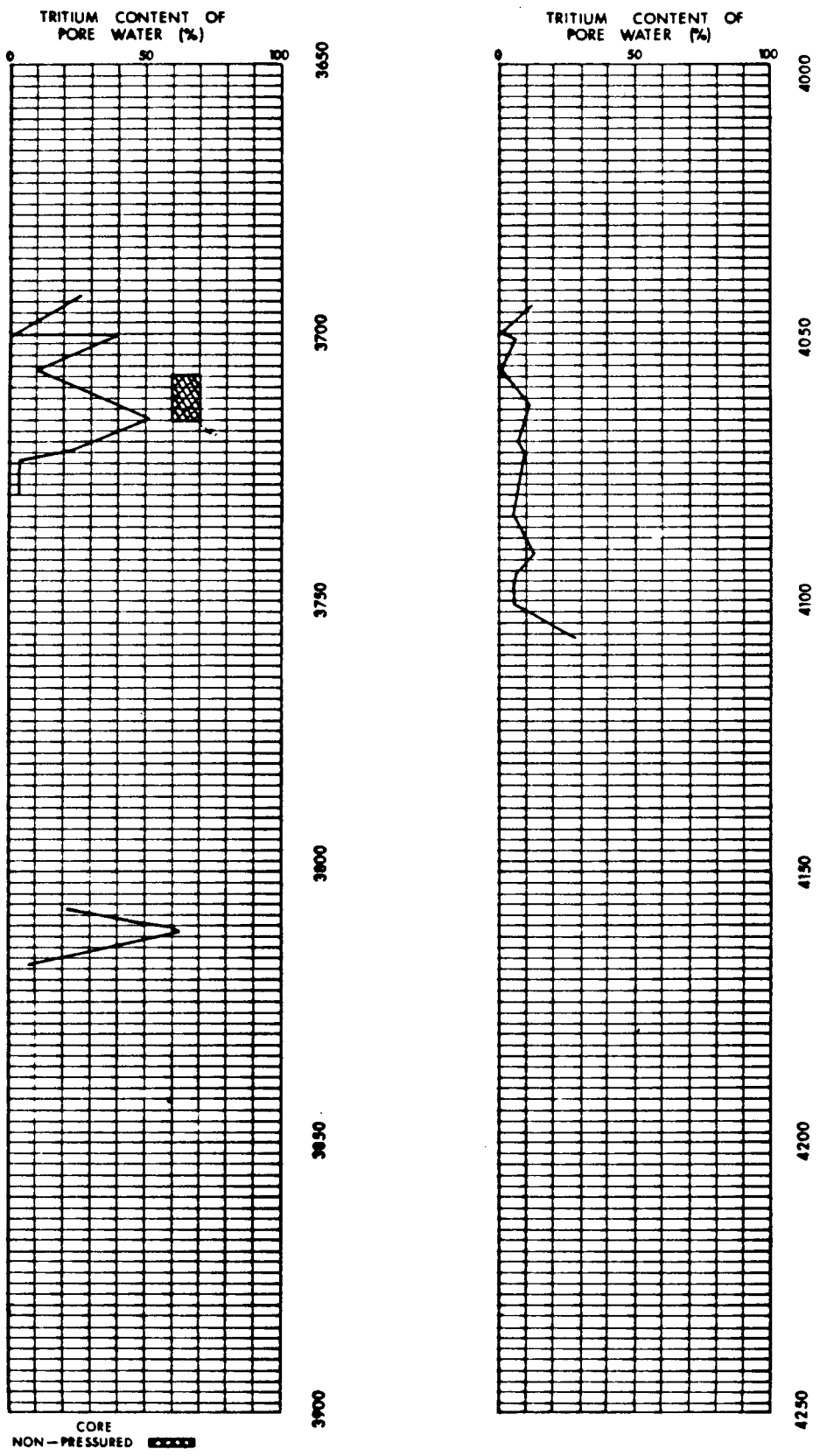
Figure 39.--Percent tritium content of pore water.
