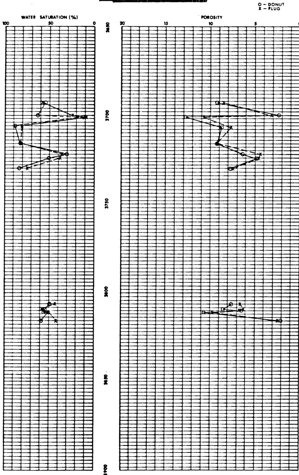
Figure 35.--Porosity and water saturation of plug and donut core samples.
