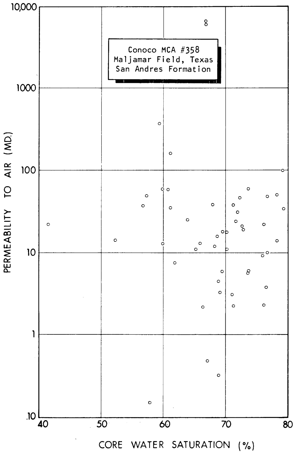
Figure 32.--Salt water saturation versus maximum horizontal permeability to air, zone 9, cores 10-18.
