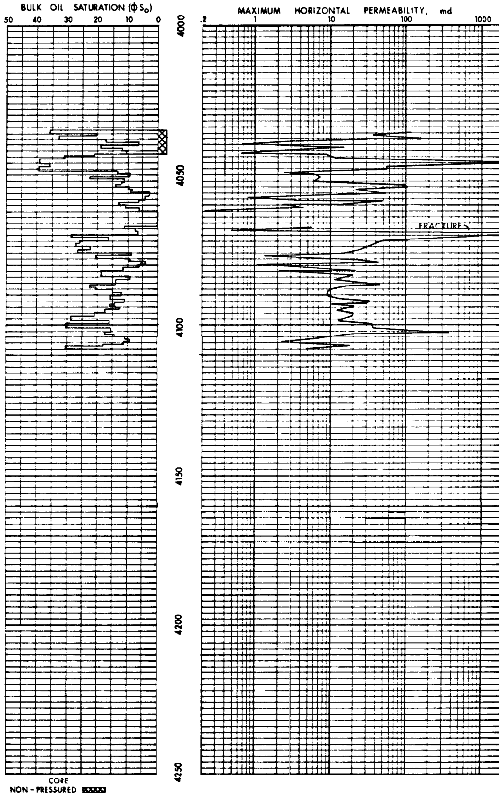
Figure 68.--Bulk residual oil saturation and maximum horizontal permeability versus depth.
