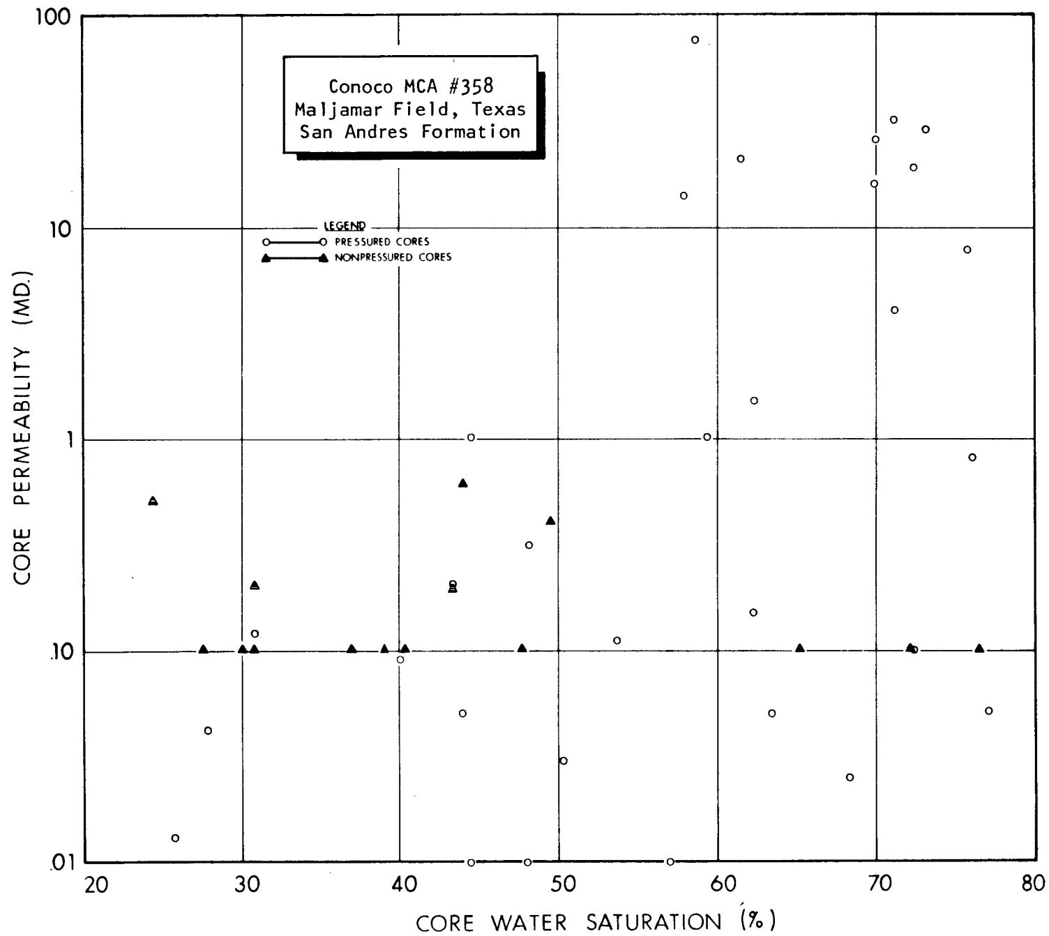
Figure 30.--Salt water saturation versus maximum horizontal permeability to air, zone 6, cores 1-6.
