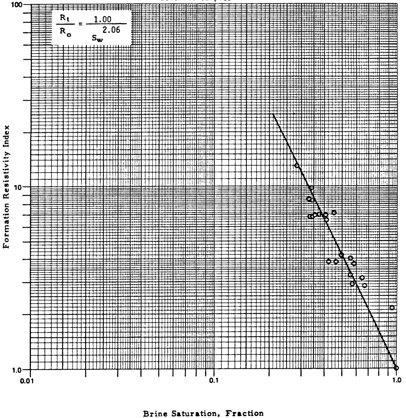
Figure 45.--Determination of saturation exponent n composite for sandstone samples.
