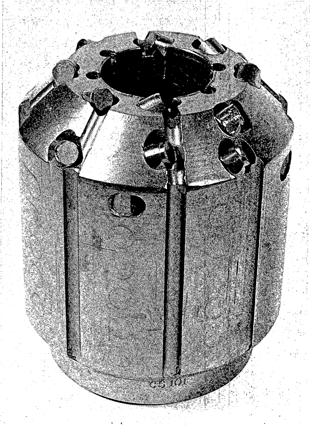
Figure 16.--Photograph of stratapax ® bit.
