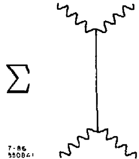
Fig. 1. Four graviton scattering.
